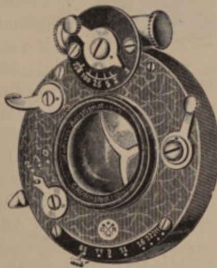
FIG. 144.—Compound Sector Shutter.
