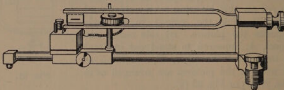
FIG. 24.—Electrically-driven Tuning-fork with Slits.
