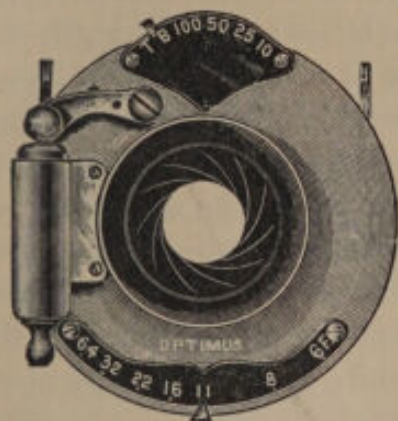
FIG. 143.—Perken's Iris Shutter.
