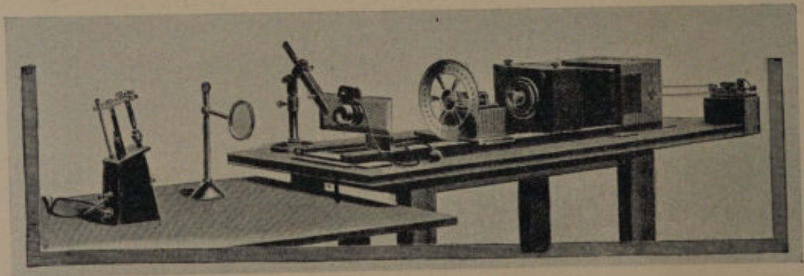
FIG. 152.—Sir William Abney's apparatus for determining the speed of a shutter.
