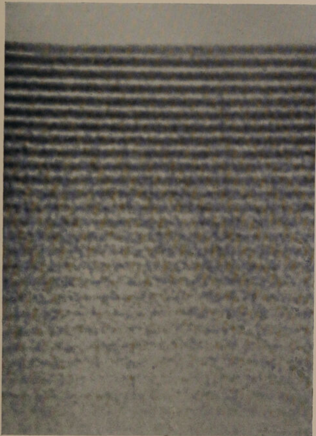
FIG. 163.—Section of a Lippmann Photographic Film, made through the red end of the spectrum of arc light ( \times 11,000 ). Prepared and photographed by Edgar Senior, Esq., and reproduced here by his permission. Zeiss' Apoch. Obj. 3 mm. Oc. 2; yellow screen.
