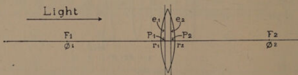
FIG. 51.—Gauss' points in a biconvex lens.
