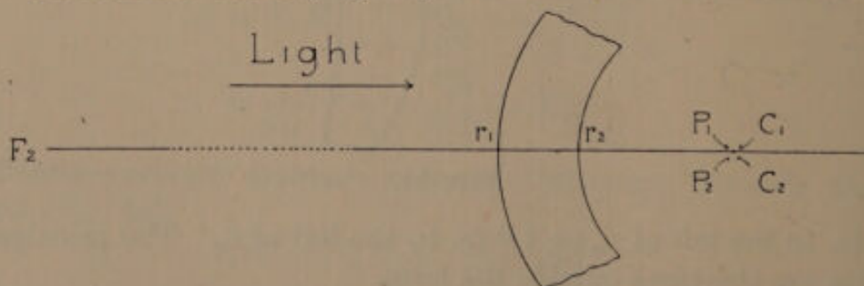
FIG. 57.—Concentric lens.
