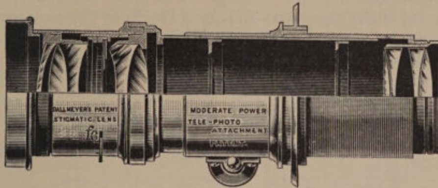
FIG. 81.—Construction of a Telephoto Lens (Dallmeyer).
