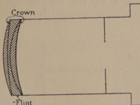
FIG. 73.—Single Achromatic Landscape Lens.
