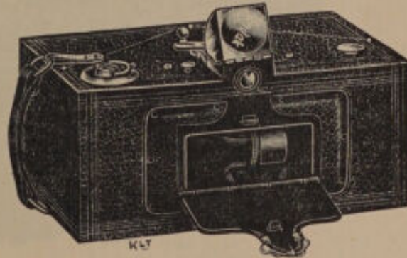
FIG. 16.—Kodak Panoramic Camera.
