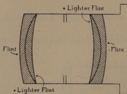
FIG. 77.—Diagram of an R.R. Lens.
