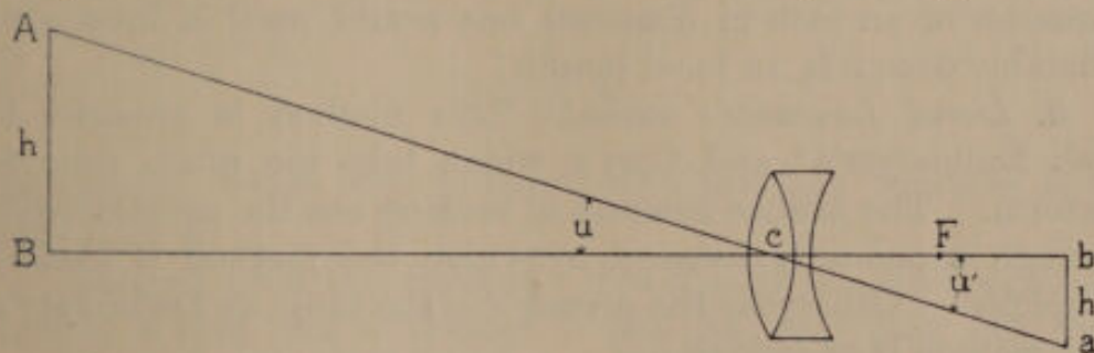
FIG. 65.—Angular method of finding the focal length.
