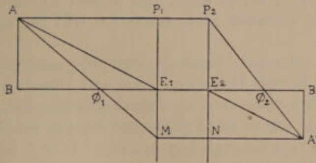
FIG. 44.—Diagram showing Gauss' points and planes.
