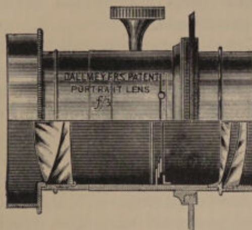
FIG. 75.—Dallmeyer's Improved Portrait Lens.
