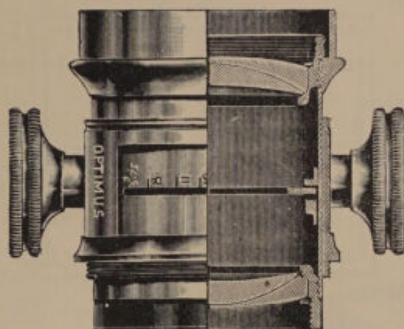
FIG. 130.—Perken & Son's Grossar Enlarging Lens.
