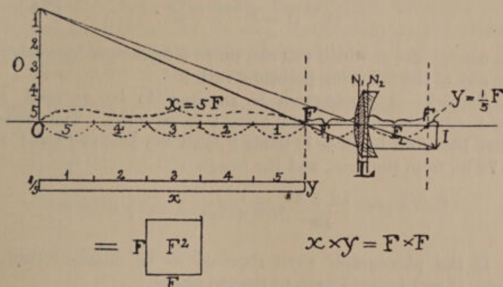
FIG. 125.—Graphic demonstration of the formula xy = F^2 .
