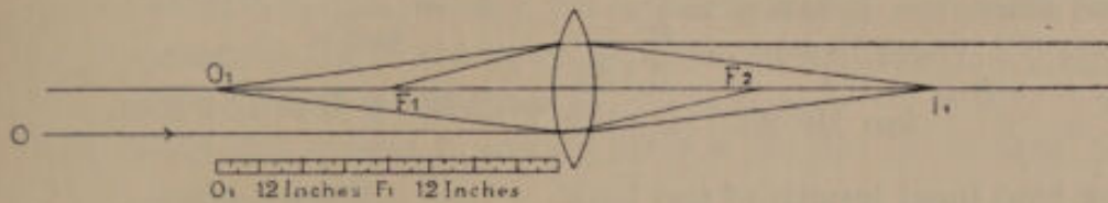
FIG. 64.—Conjugate method of finding the focal length.
