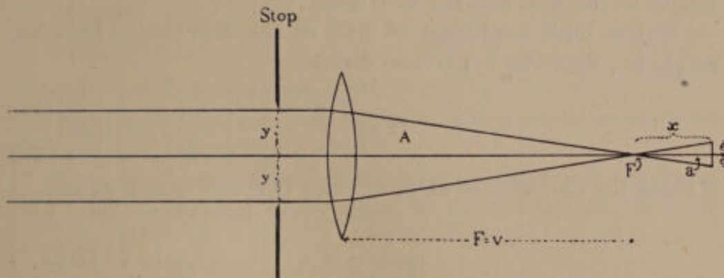
FIG. 69.—Diagram illustrating depth of focus.
