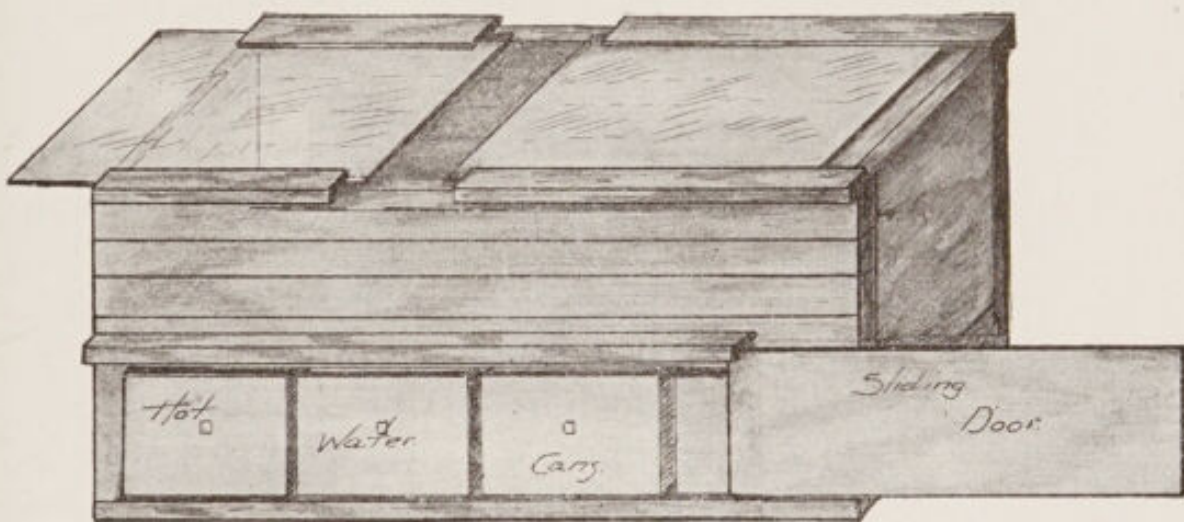
FIG. 49.—Improved incubator.
