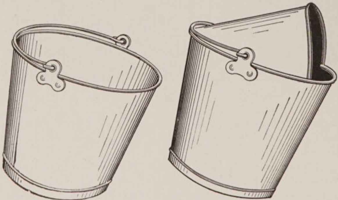
FIG. 52.—Open and hooded milk pails. A hooded pail will keep much dirt out of the milk. The hood can be put on by any competent tinsmith for a small price. (Courtesy U. S. Bureau of Animal Industry.)
