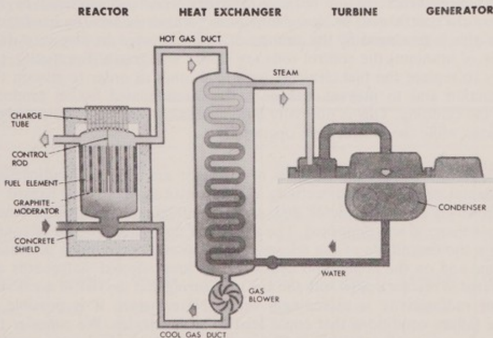
Schematic diagram of a thermal reactor (Magnox).
