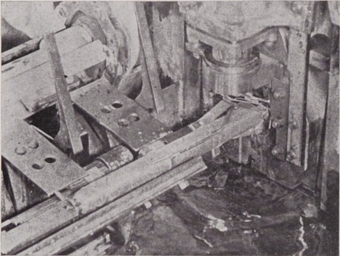
Plate 10. Magnox fuel cladding being removed.
