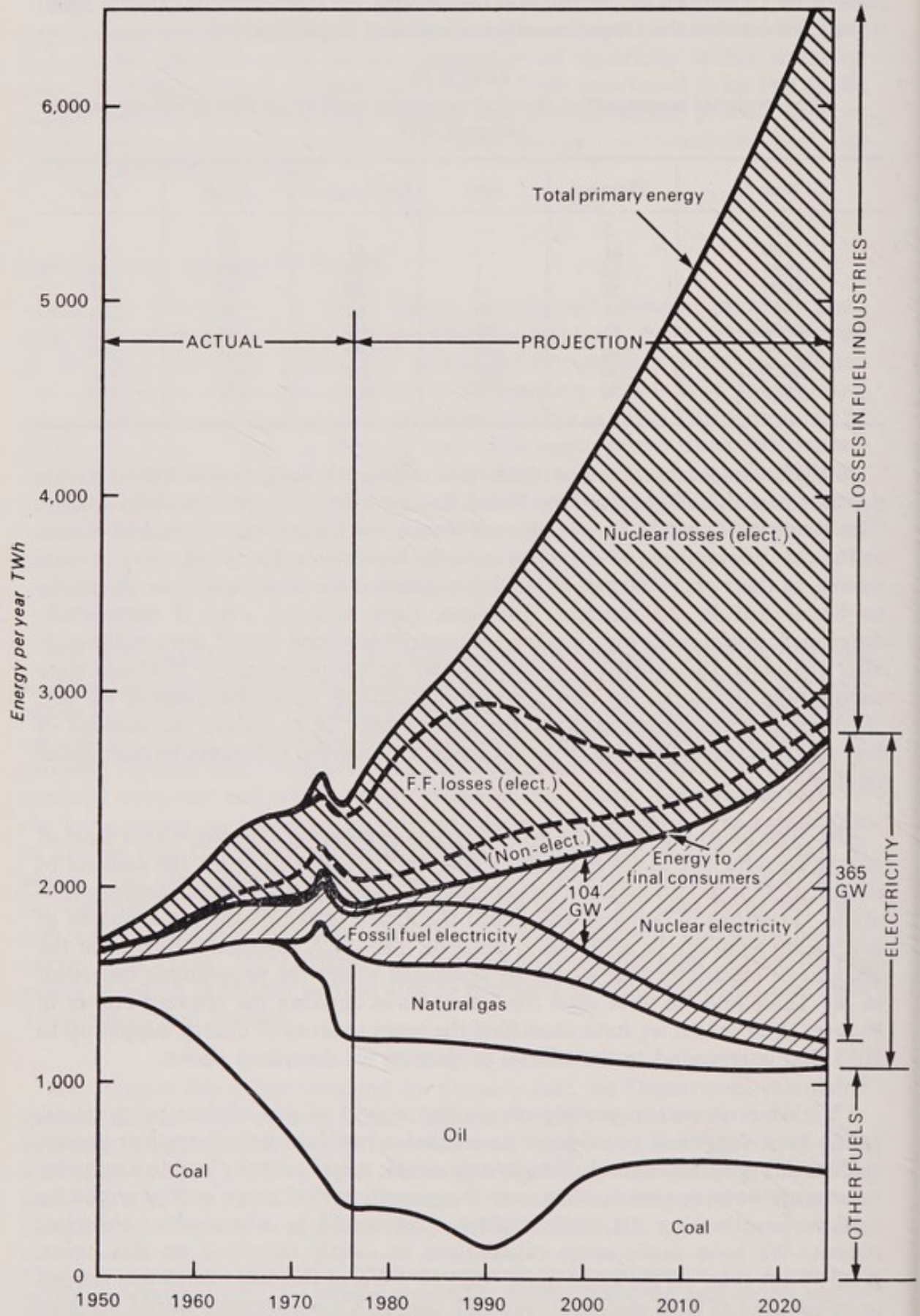
The provision of energy for the UK, projected to 2025, on the 'official strategy'.
