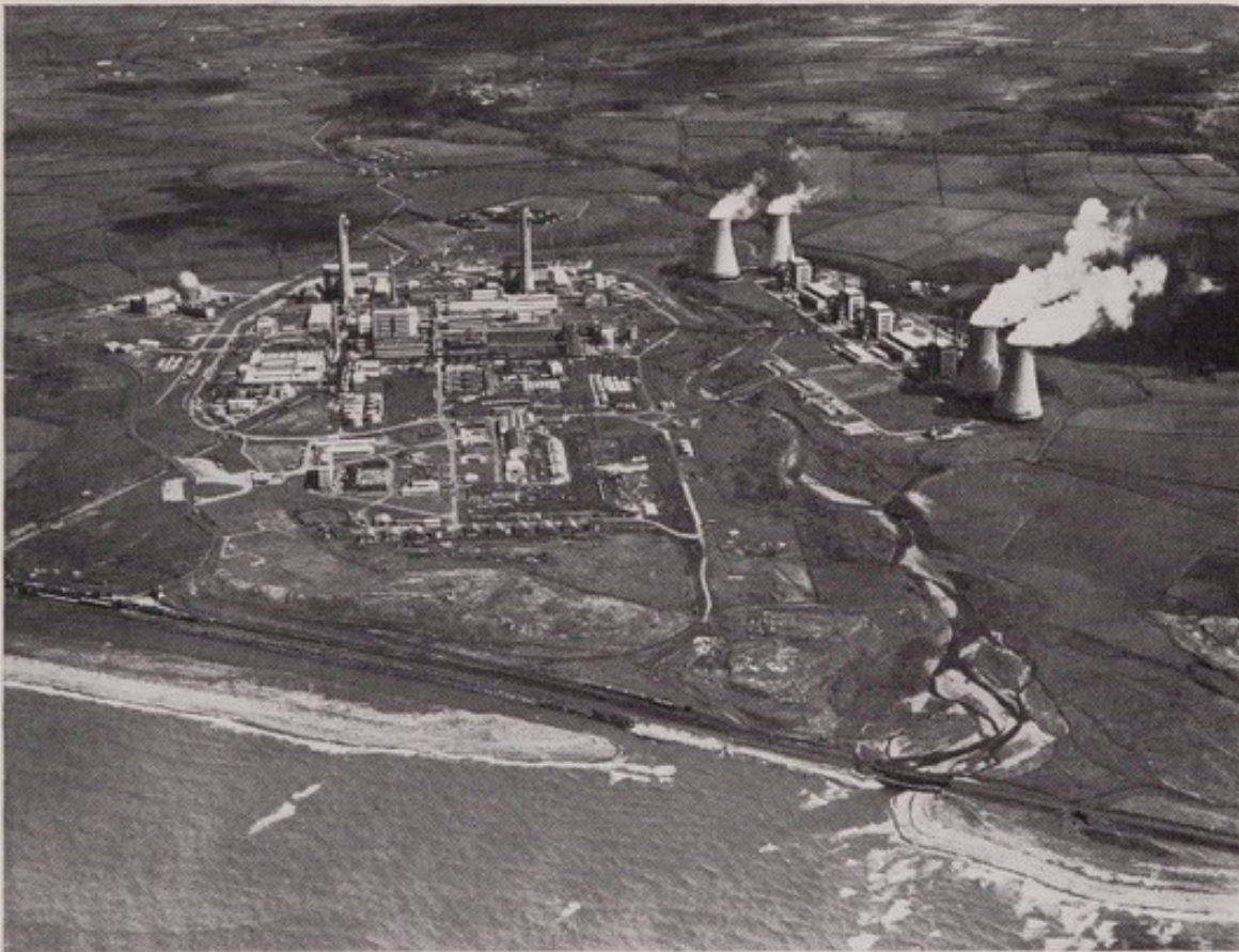
Plate 8. The Windscale works of BNFL on the Cumbrian coast. On the right are the four 50 MW reactors at Calder Hall; on the left the sphere contains the 33 MW prototype AGR. The original 'Windscale Piles' are immediately behind the tall stacks. The reprocessing plant is in the centre of the site and the route of the discharge pipelines to sea can be seen on the extreme left.
