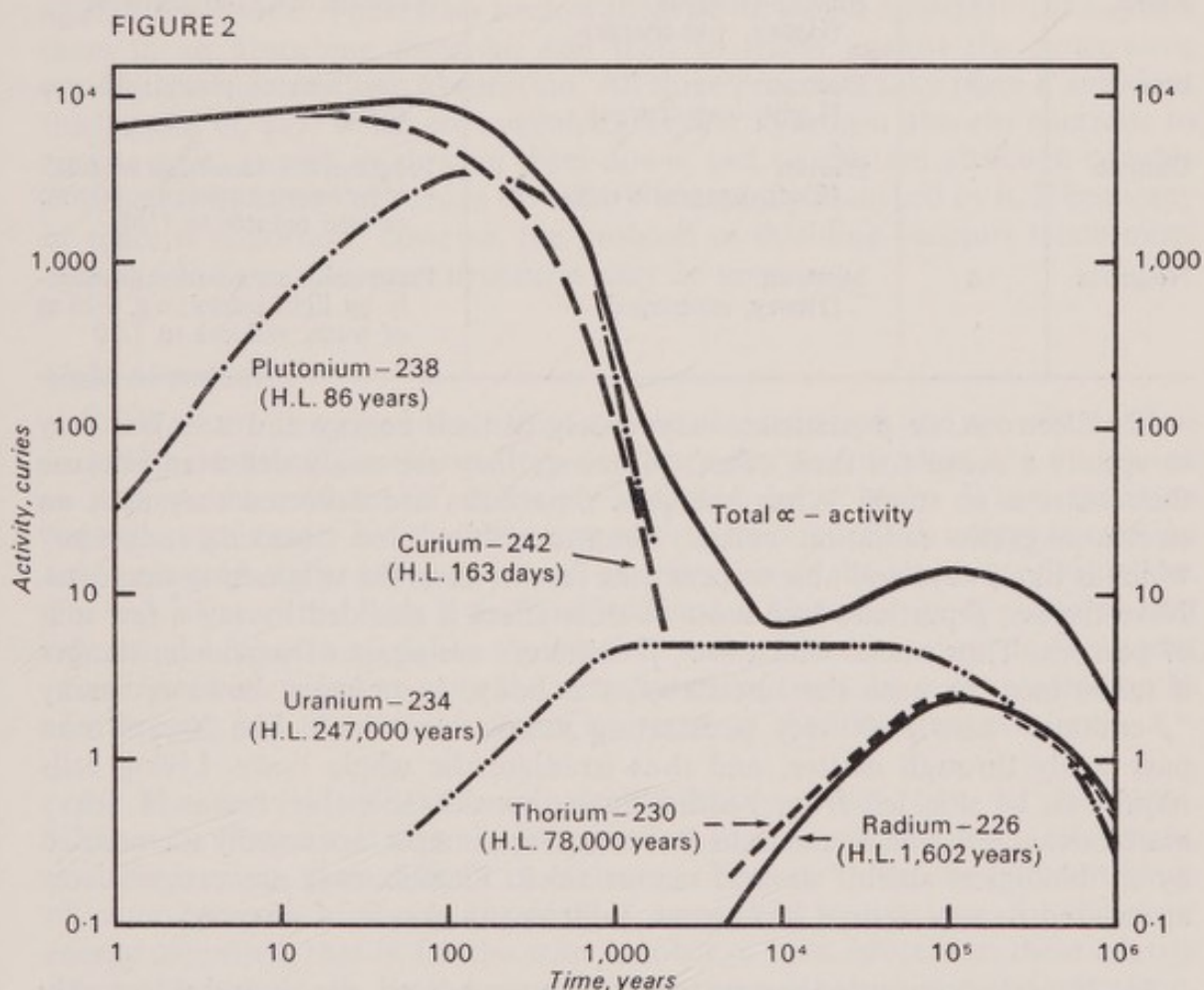
Alpha-activity from decay of 1 kg of americium-242m (half-life, 152 yr) and its decay daughters.
