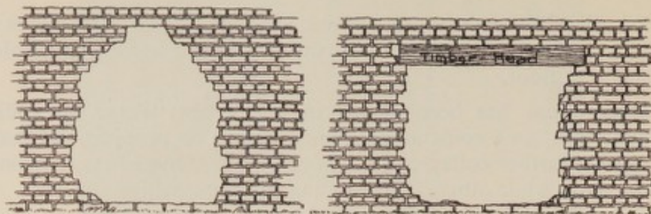
Fig. 80. Hole through brick wall: lime mortar
