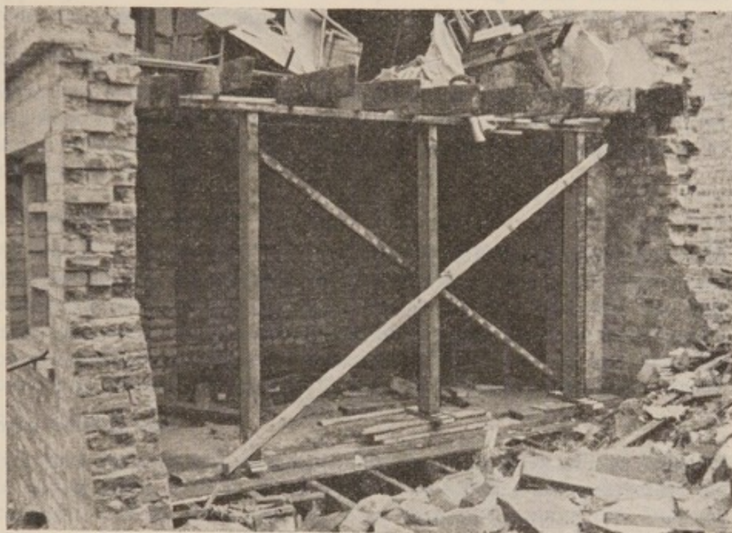
Fig. 130. Improvised dead shore
