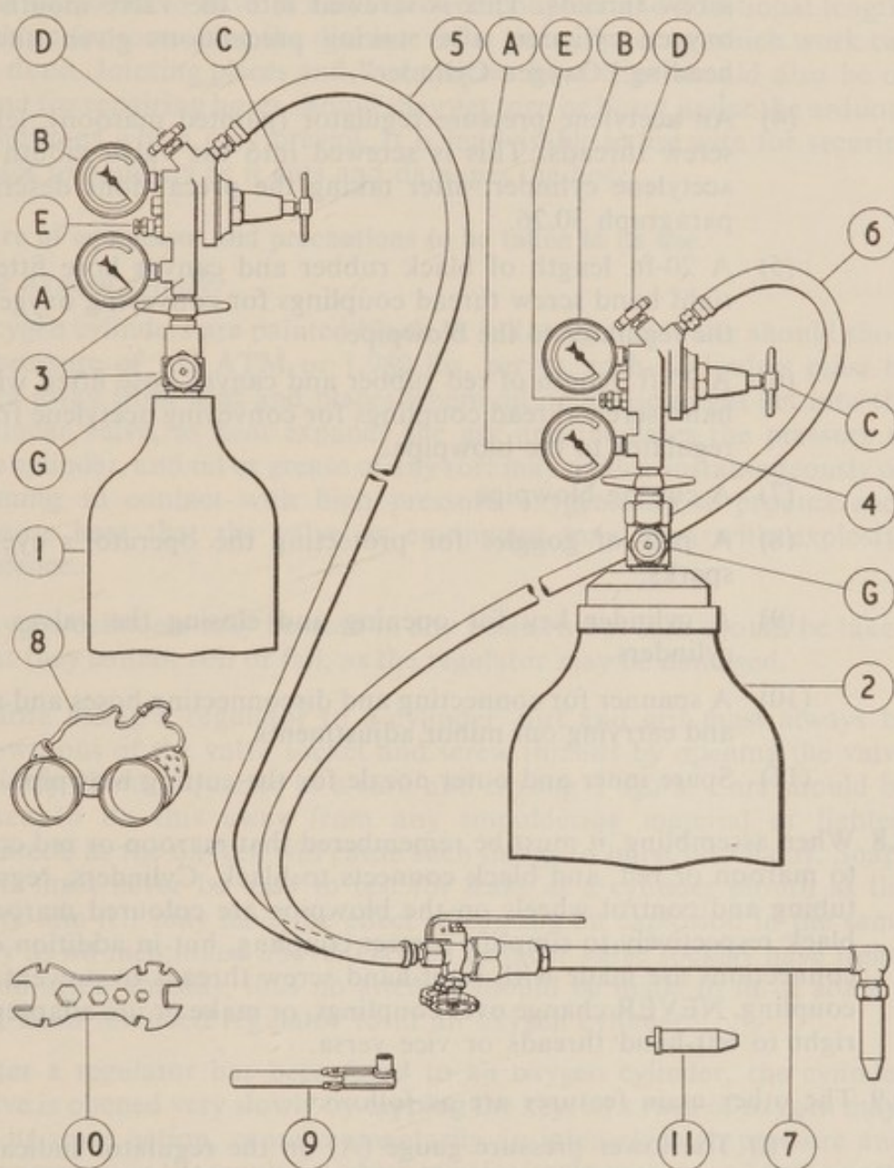
Fig. 135. Cutting equipment
