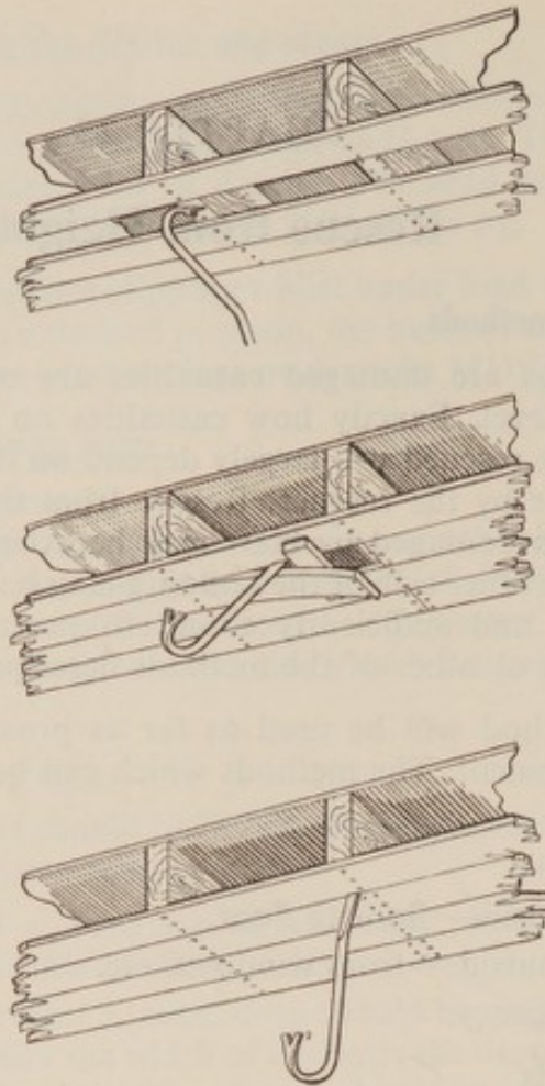
Fig. 95. Uses of wrecking bar
