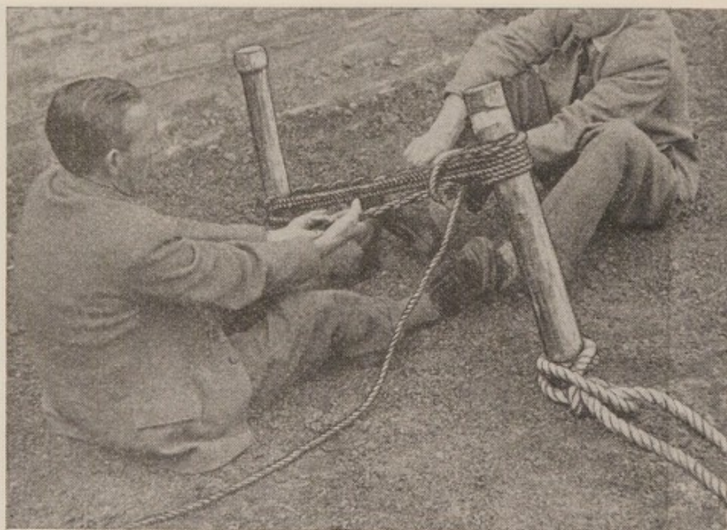
Fig. 85 (c). A 1 and 1 picket
