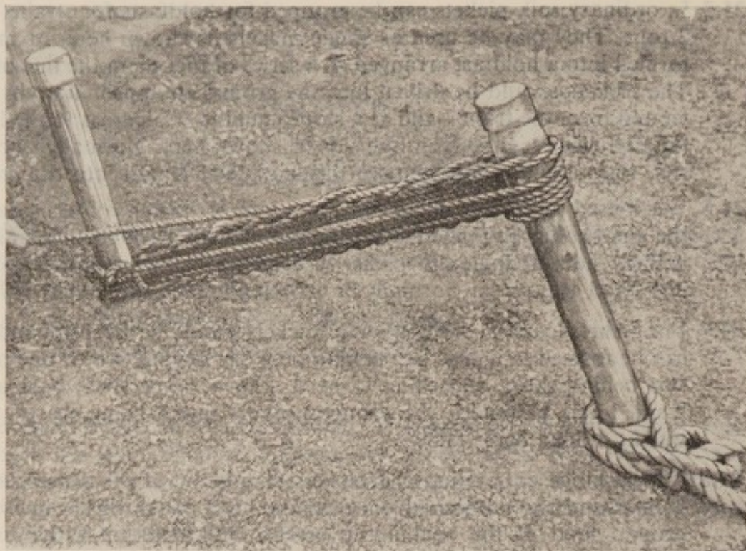
Fig. 85 (b). A 1 and 1 picket
