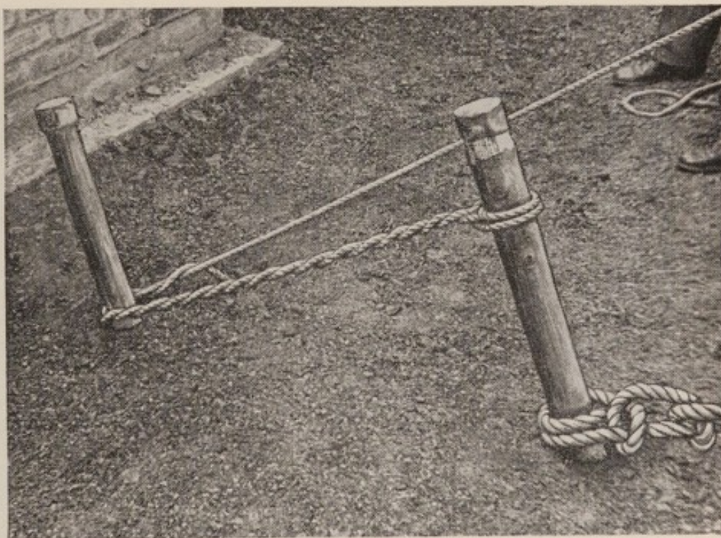
Fig. 85 (a). A 1 and 1 picket
