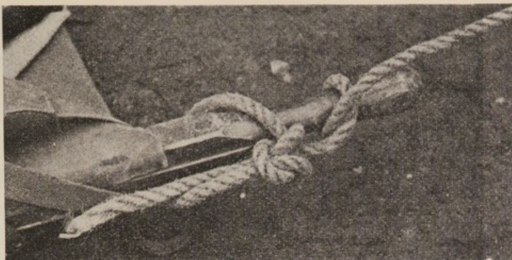
Fig. 96. Correct method of fastening 40 ft. lashing for two-point suspension
