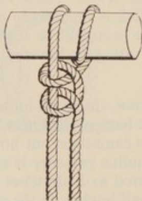
Fig. 61. Round turn and two half-hitches
