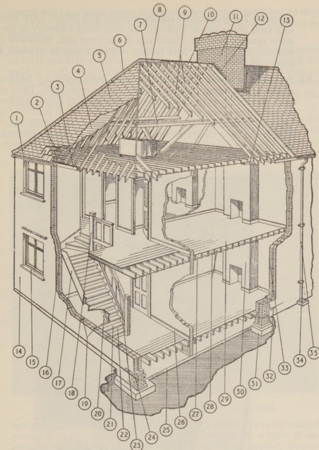
Fig. 11. Constructional details of an ordinary dwelling house
