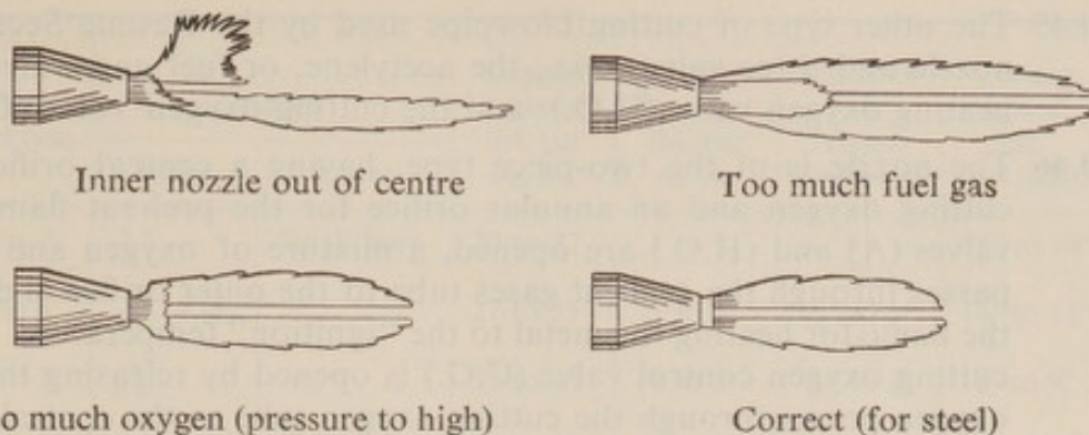
Fig. 138. Flame adjustment for cutting
