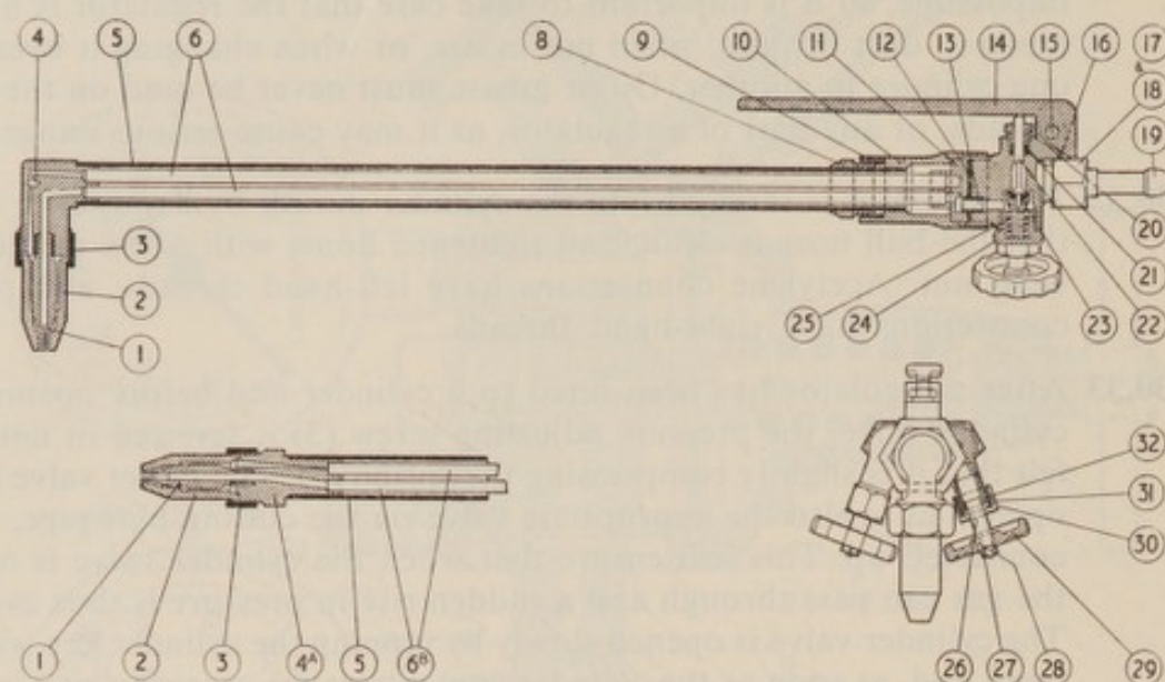
Fig. 137. One type of cutting blowpipe
