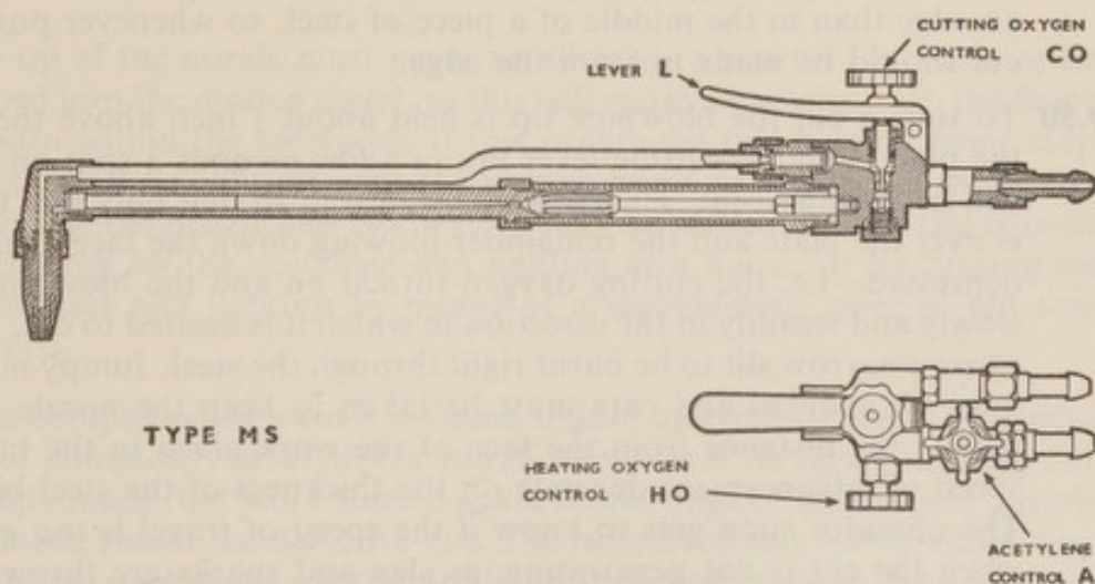
Fig. 139. Another type of cutting blowpipe
