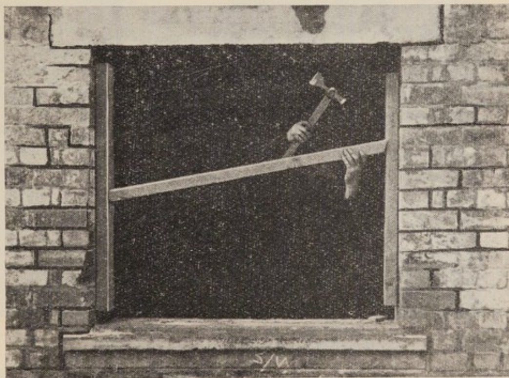
Fig. 69 (a-c). Strutting of window opening
