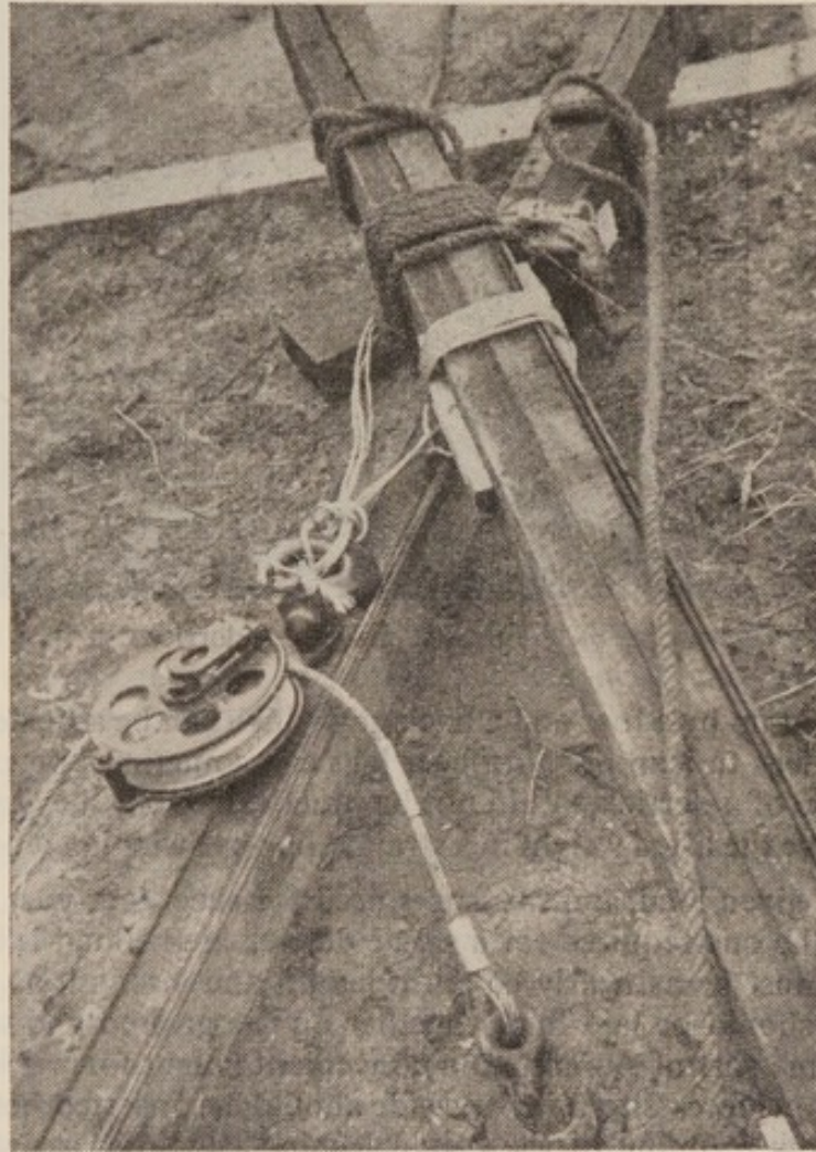
Fig. 93. Improvised shear leg frame, ready for positioning and erection
