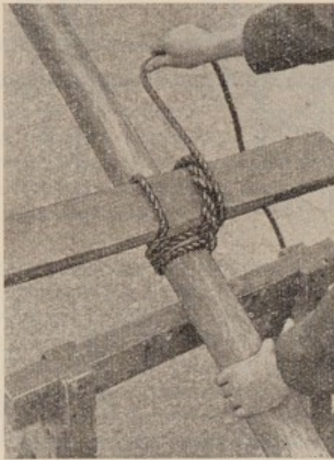
Fig. 64. Start of a square lashing
