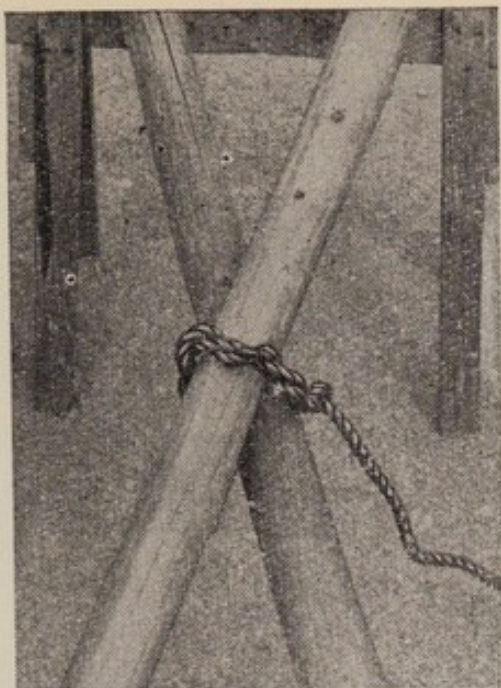
Fig. 66 (a). Diagonal lashing
