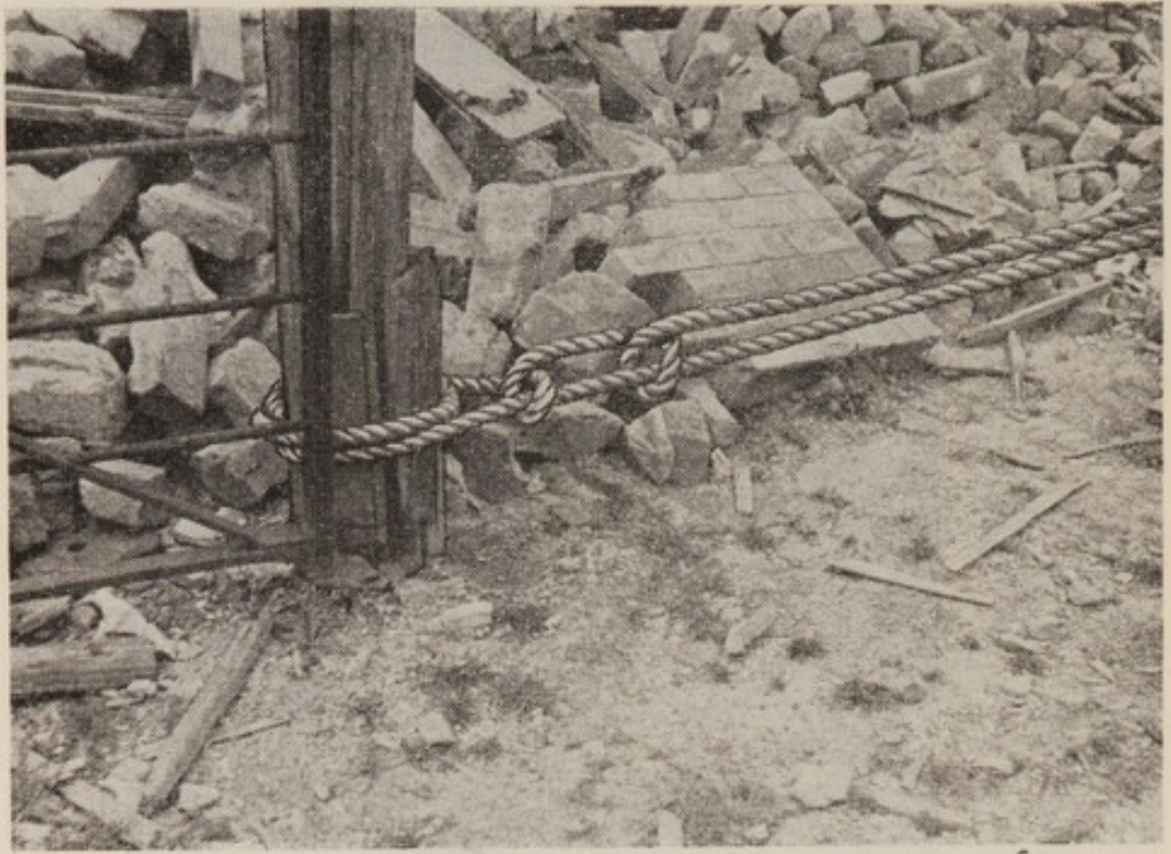
Fig. 89 (e). Improvised holdfasts
