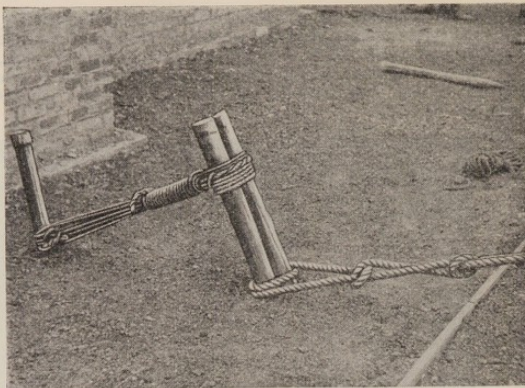
Fig. 86. A 2 and 1 picket
