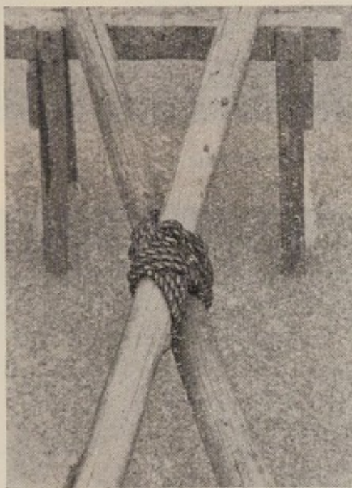
Fig. 66 (c). Diagonal lashing
