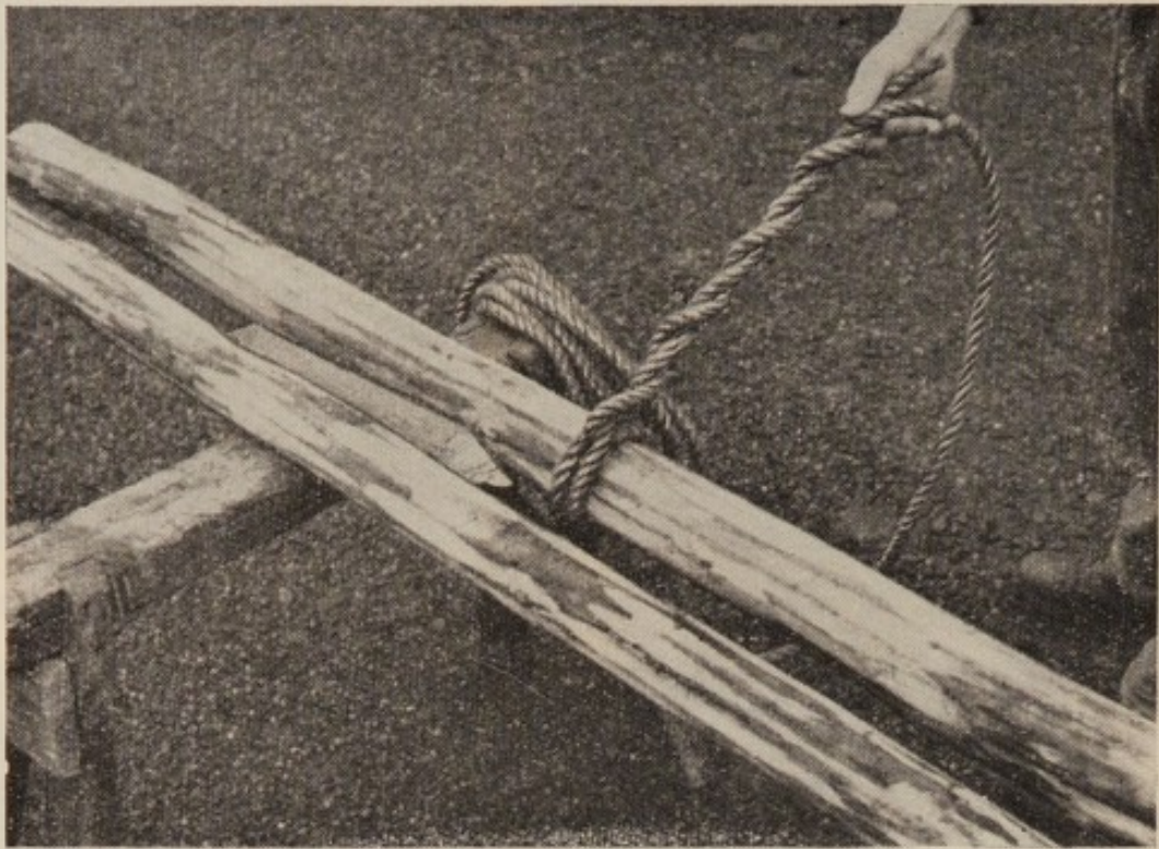
Fig. 67 (a). Round lashing
