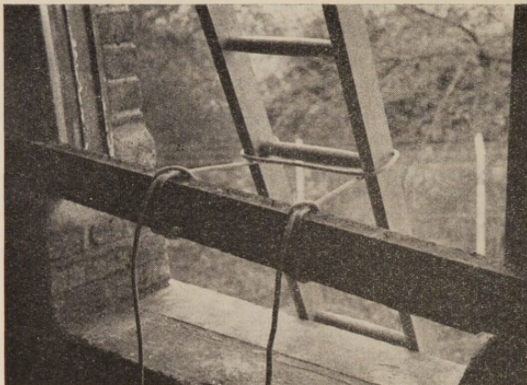
Fig. 76. Fastening head of ladder
