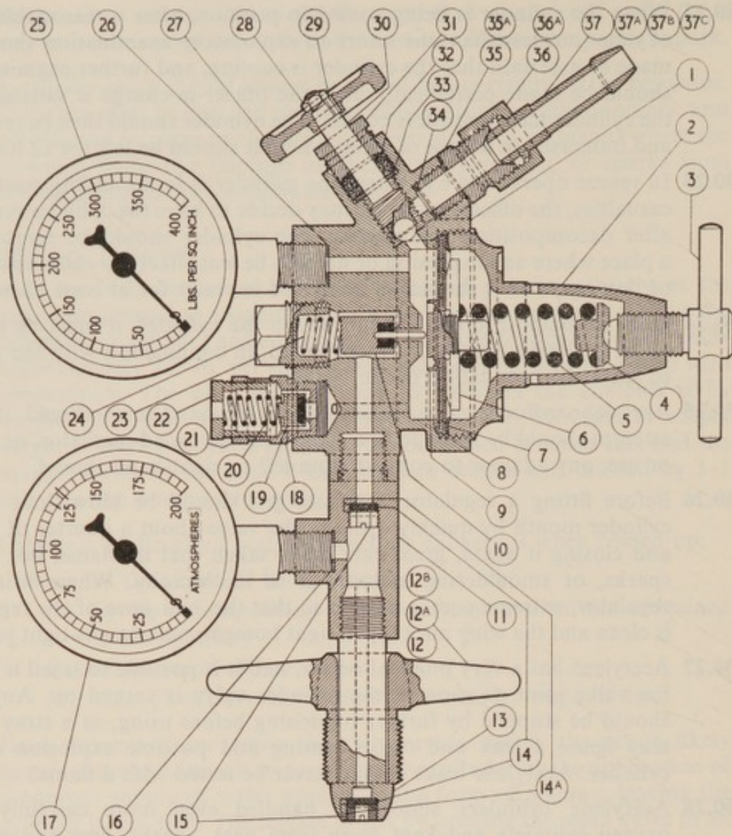
Fig. 136. The regulators
