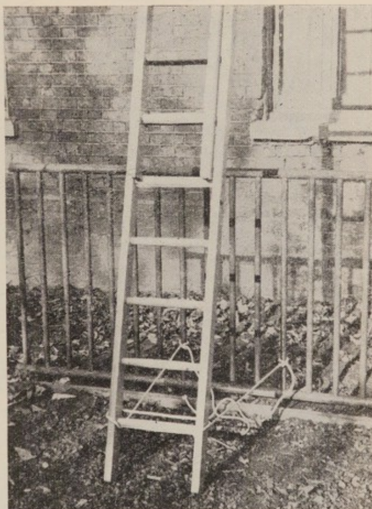
Fig. 75. Anchoring foot of ladder
