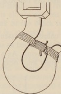
Fig. 53. Mousing
