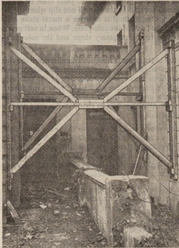
Fig. 128. Flying shore
