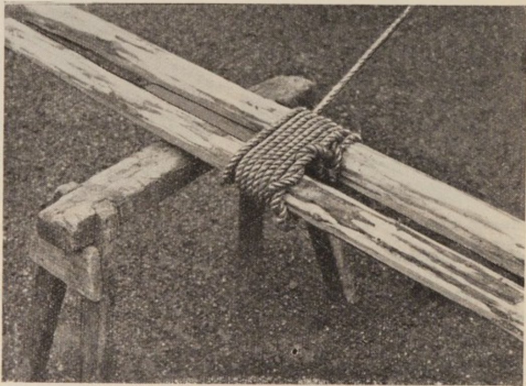
Fig. 67 (b). Round lashing
