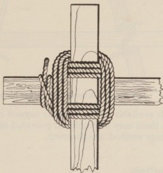
Fig. 99 (a). Improvised ladder hinge
