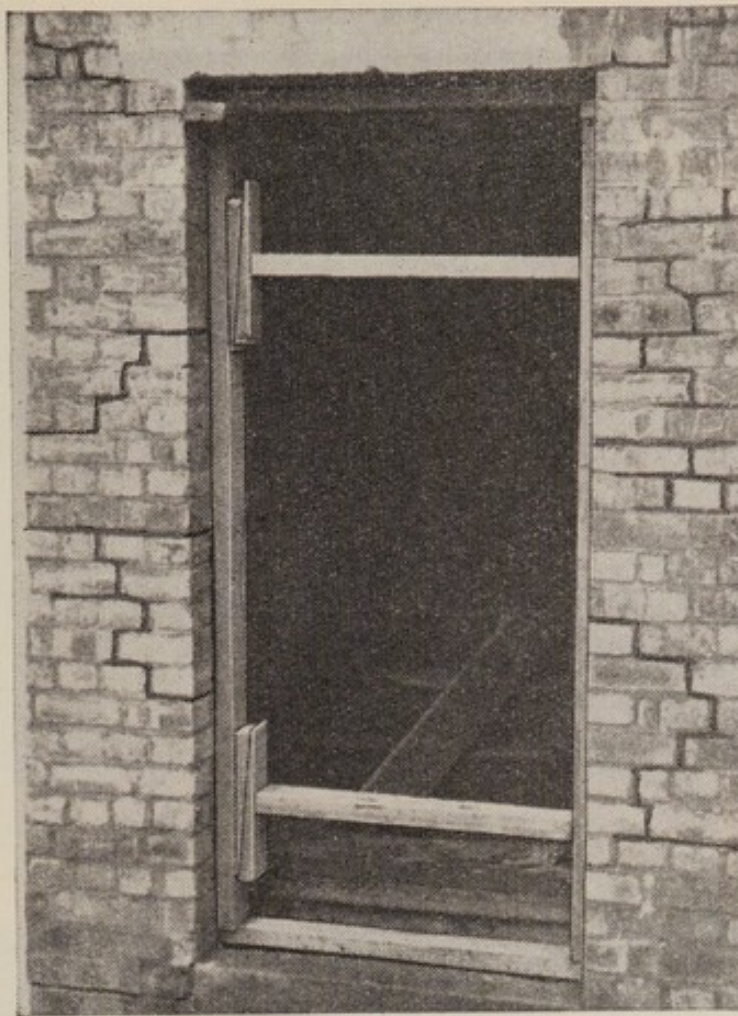
Fig. 70. Strutting a door opening
