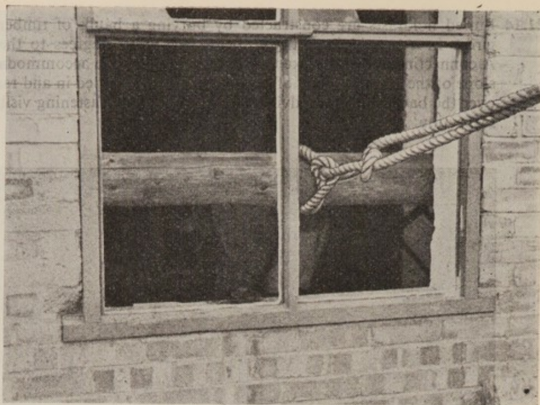
Fig. 89 (a). Improvised holdfasts
