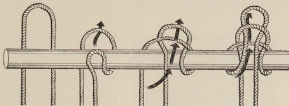
Fig. 63. Draw hitch
