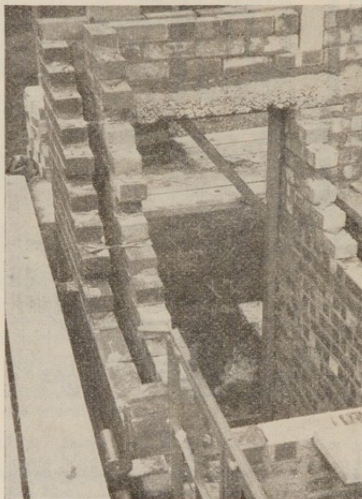
Fig. 12. Hollow wall construction
