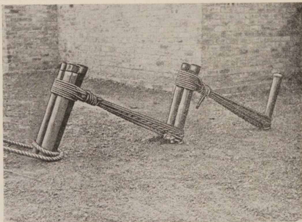
Fig. 87. A 3, 2 and 1 picket
