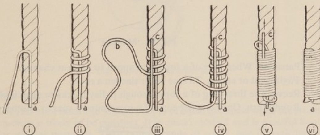
Fig. 51. Whipping the end of a rope
