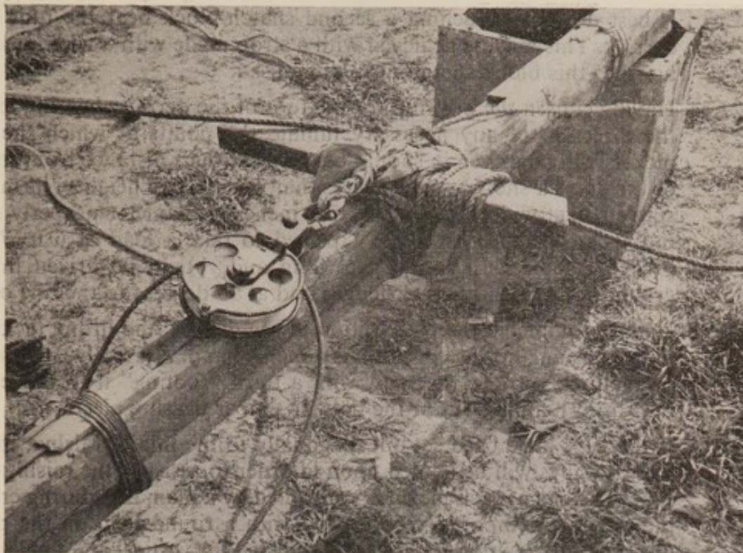
Fig. 91. Head of derrick
