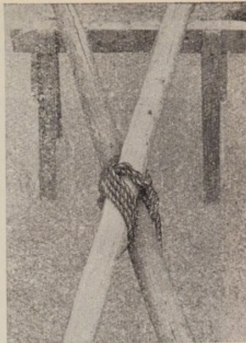
Fig. 66 (b). Diagonal lashing
