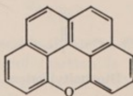
1,8,9-Perinaphthoxanthene
