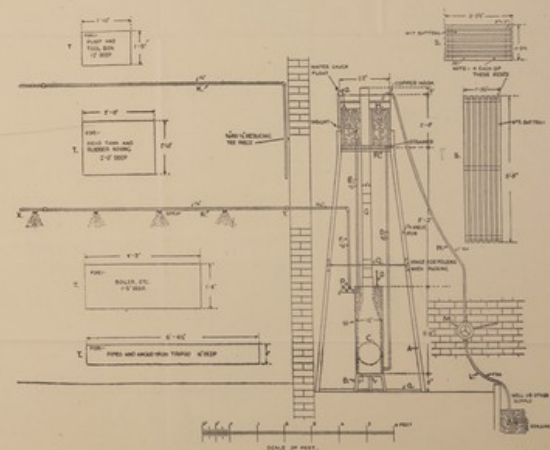
SECTIONAL DRAWINGS OF TRANSPORTABLE SHOWER-BATH.
