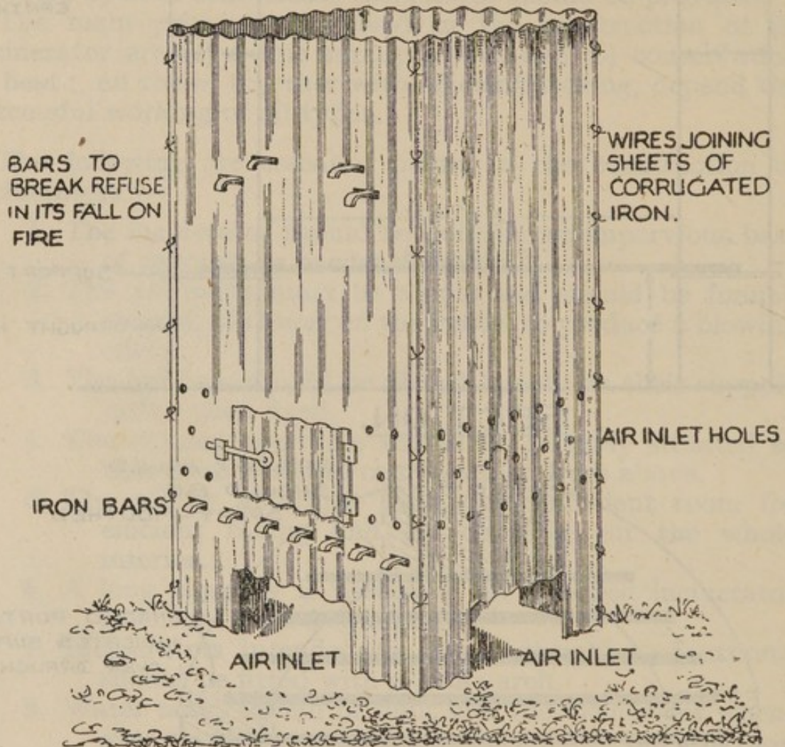
FIG. 39.—Open corrugated iron incinerator. 4 ft. 6 ins. high.
