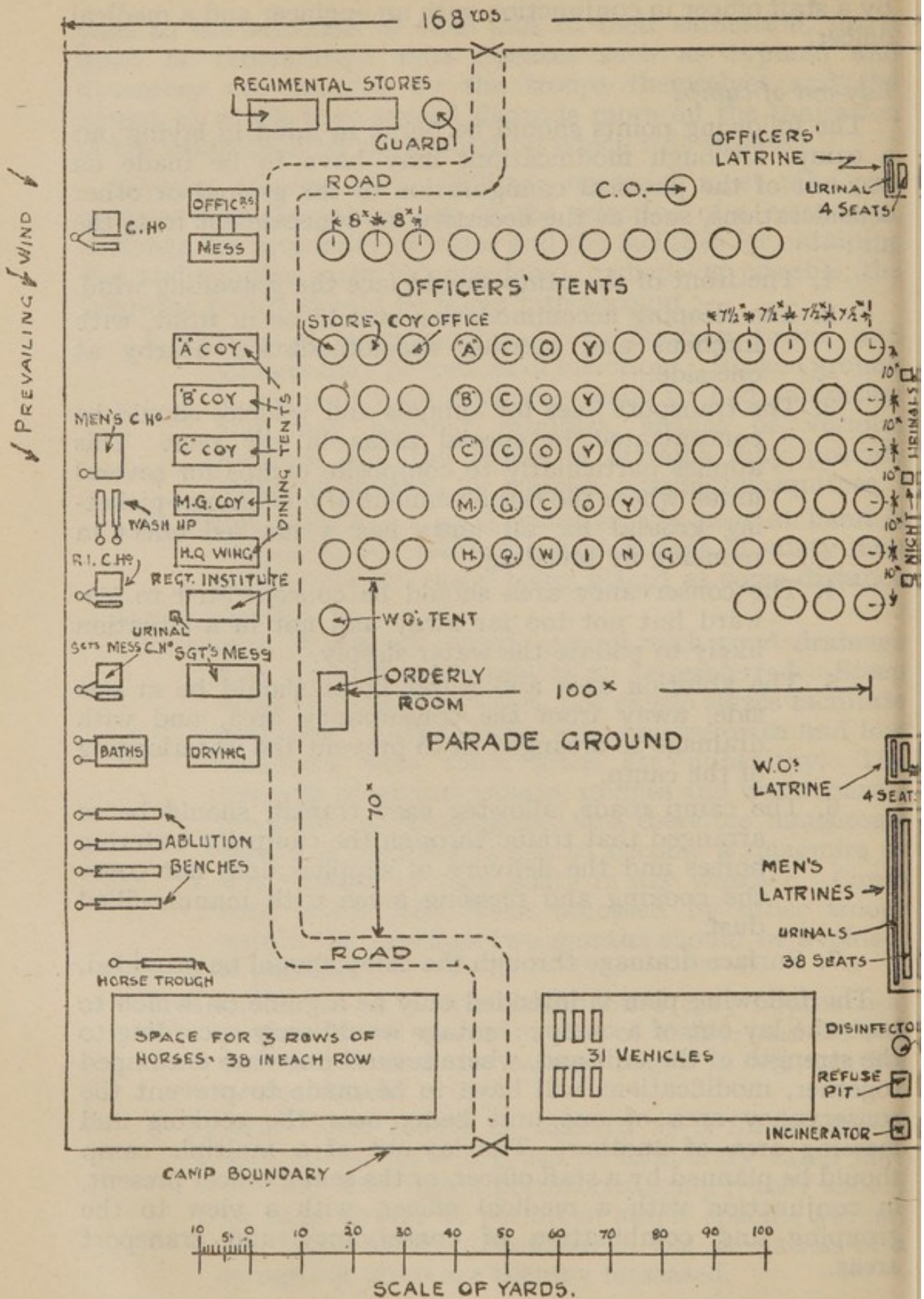
FIG. 20.—General Sanitary Principles of Lay-out of a Camp Site for a Battalion.
