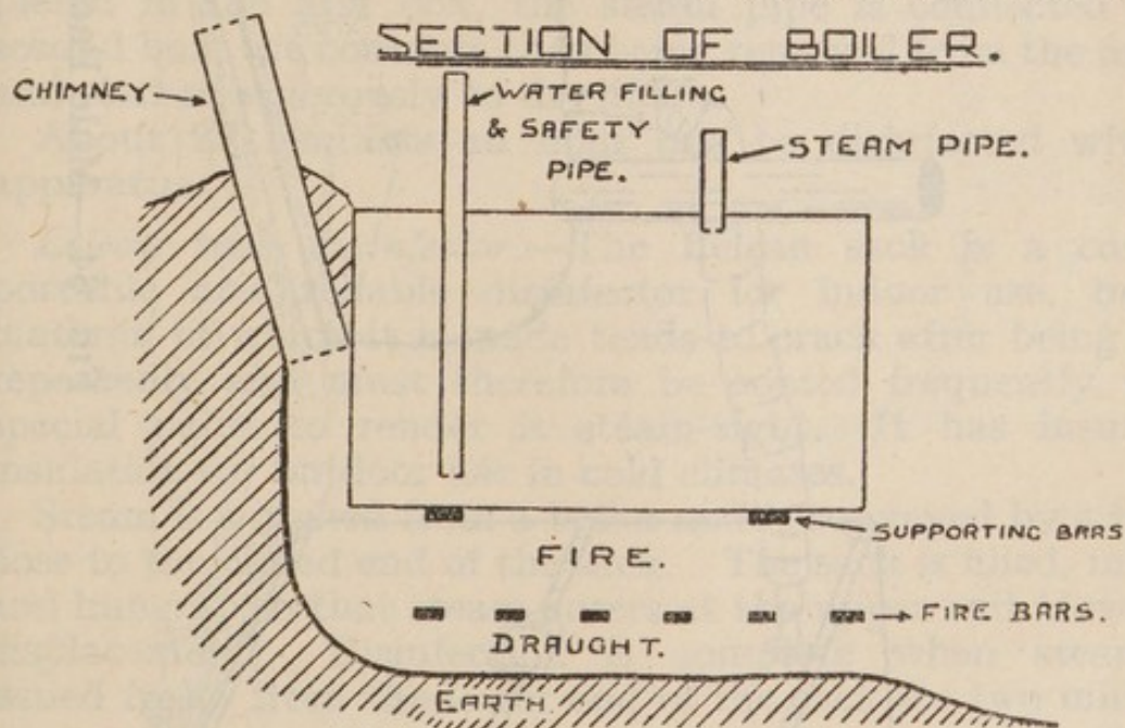
FIG. 63.—Serbian Barrel Disinfector.
