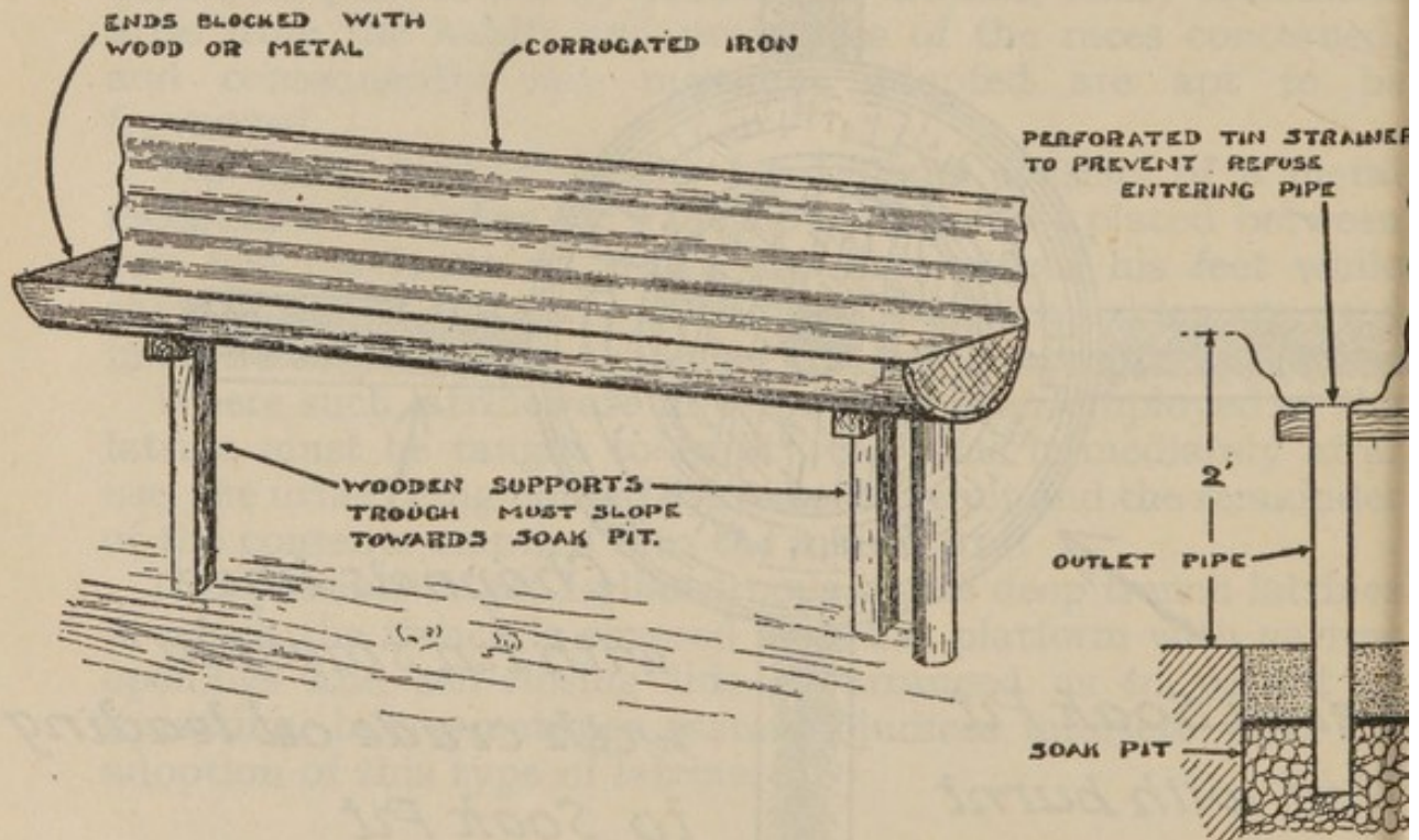
FIG. 27.—Trough urinal.
