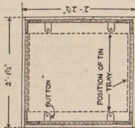
FIG. 14.—Portable fly-proof safe.
