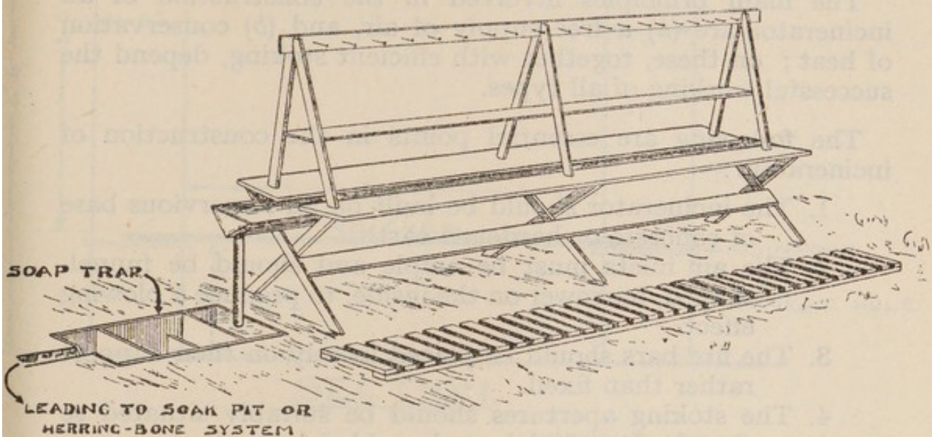
FIG. 35.—Ablution bench.
