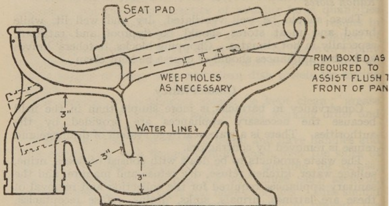
FIG. 17.—Squatting pattern wash-down water closet.
