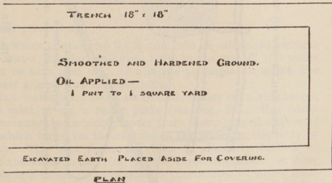
FIG. 31A.—Tight packing of manure. Using a trench.
