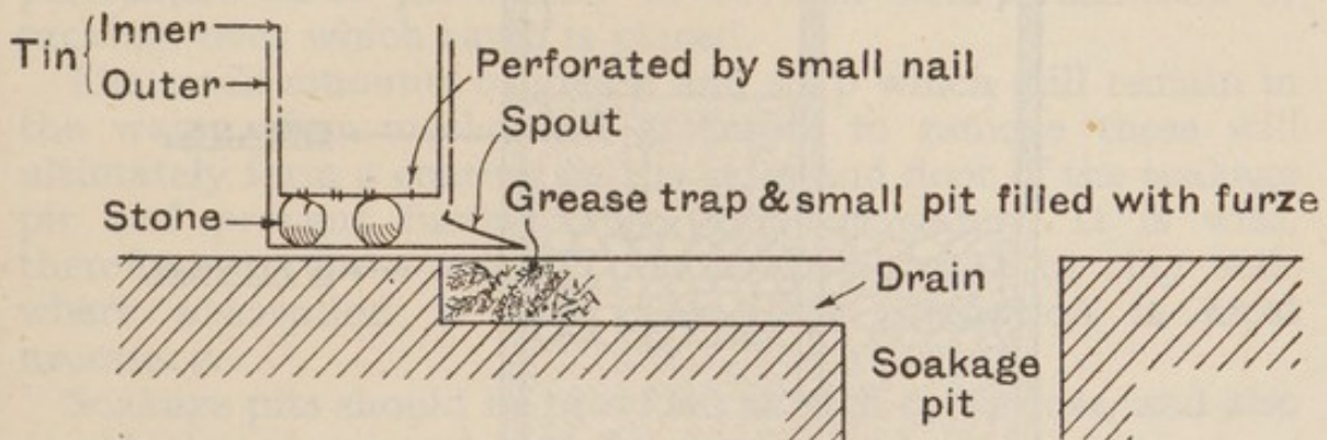
FIG. 33.—Strainer grease trap for temporary camps.
