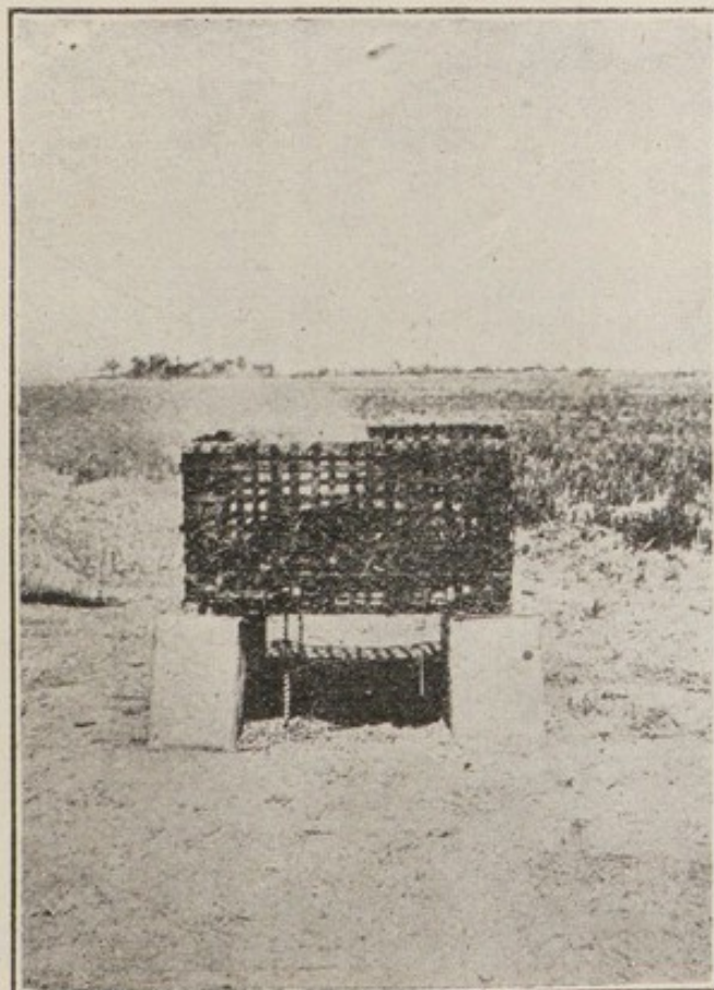
FIG. 30.—Basket incinerator.
