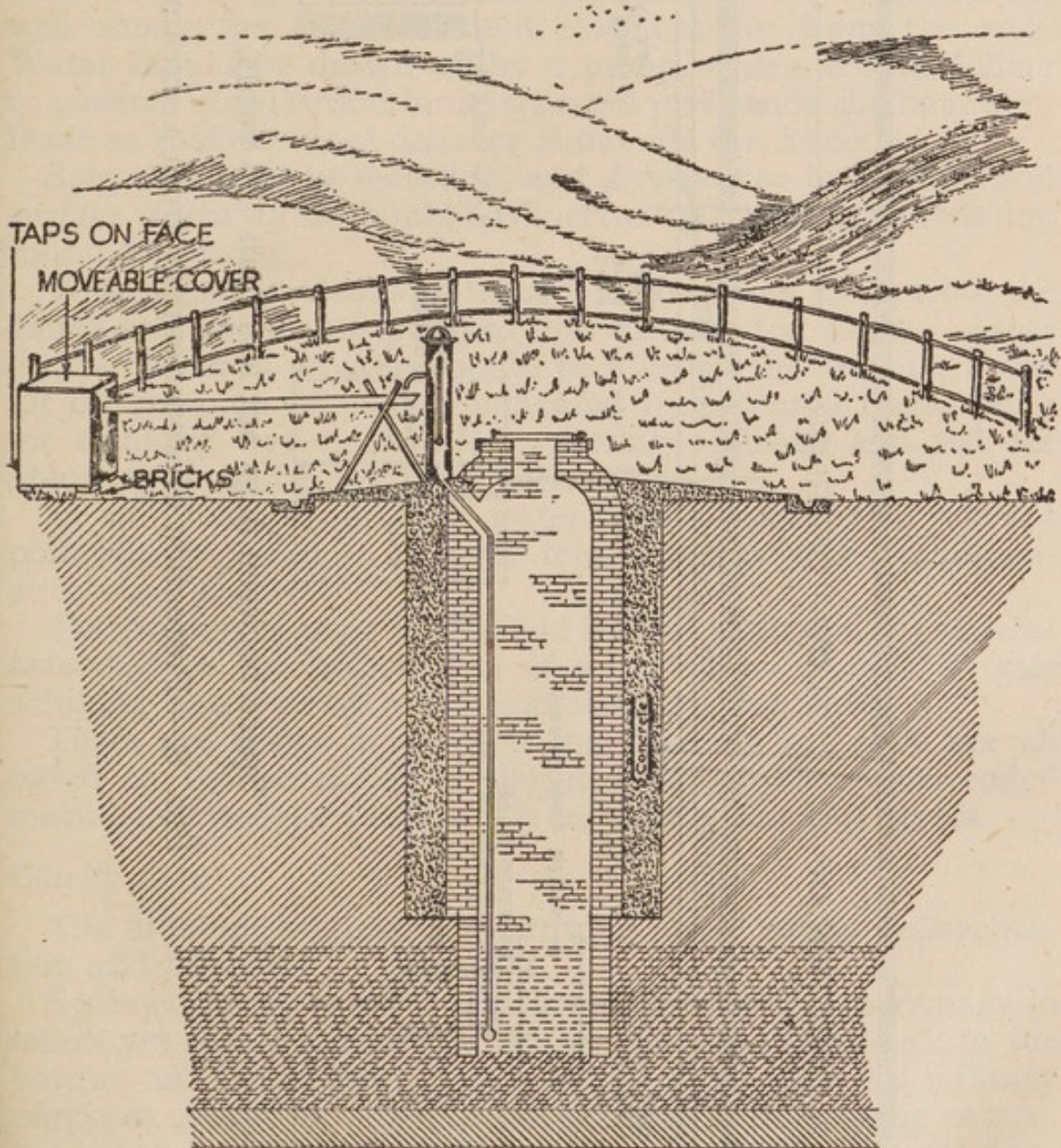
FIG. 7.—Protection of a well.
