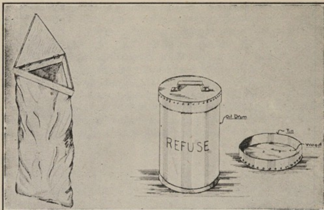
FIG. 37.—Fly-proof rubbish sack. Fly-proof bin and cover.
