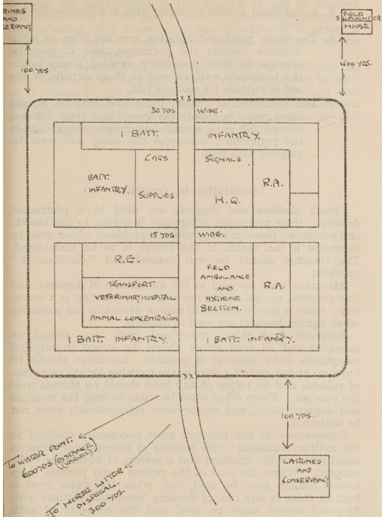
FIG. 22.—Schematic lay-out of a Perimeter camp.
