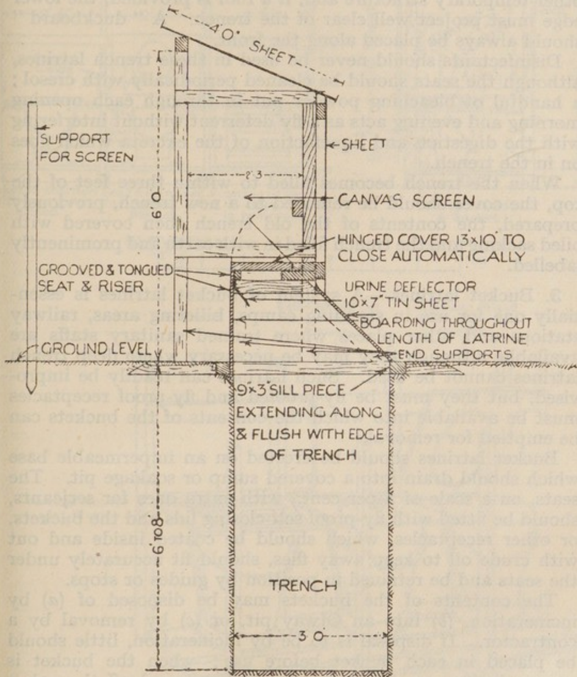
FIG. 24.—Deep trench latrine.
