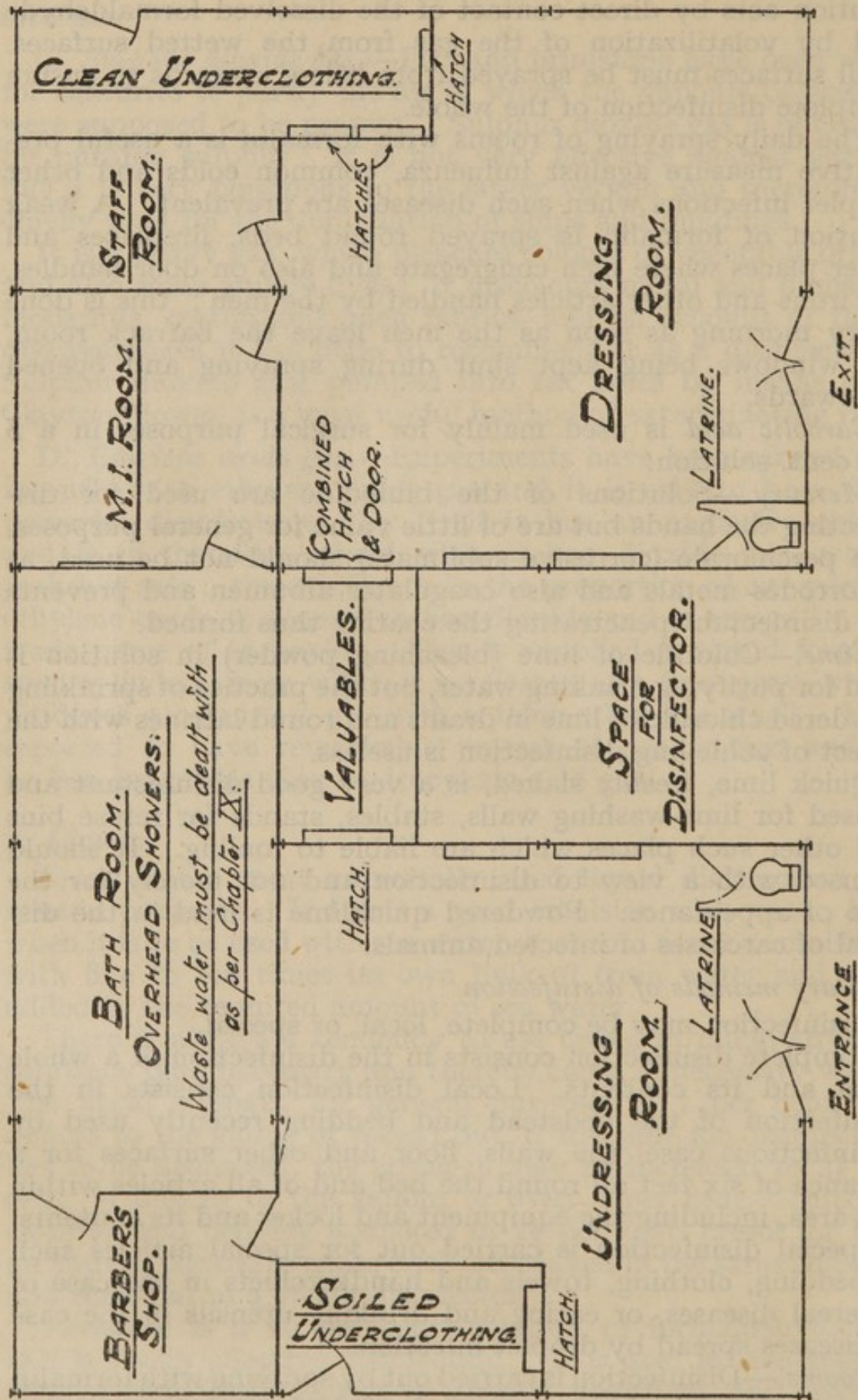
FIG. 67.—Disinfection centre
