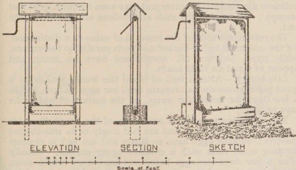
FIG. 50.—Roller-towel pattern fly trap.
