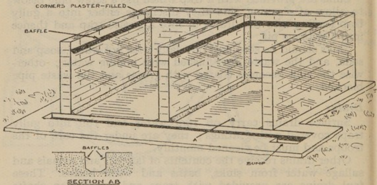
FIG. 18.—Double Collecting Manure Pit.
