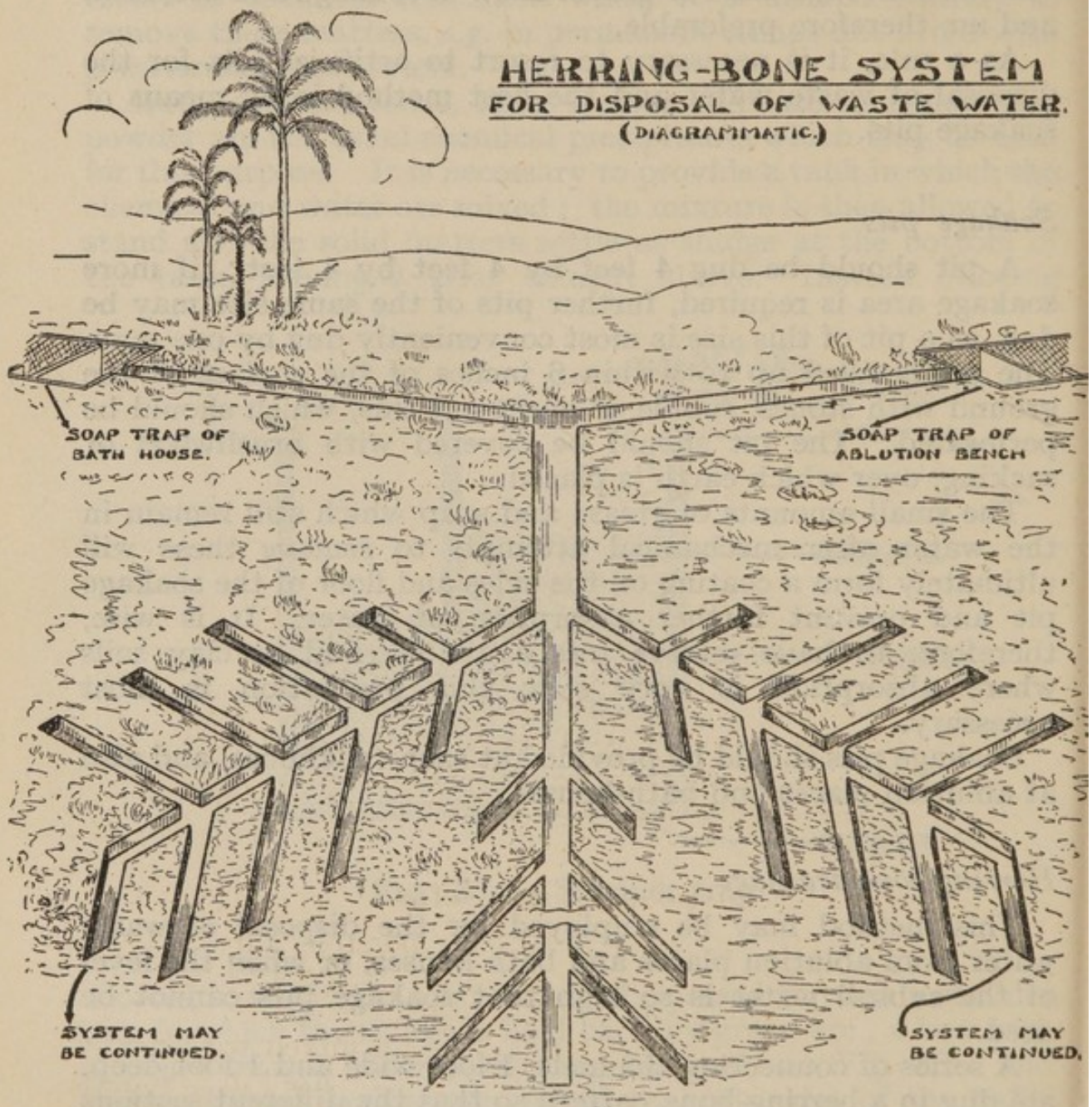
FIG. 34. Herring-Bone System for Disposal of Waste Water (Diagrammatic).
