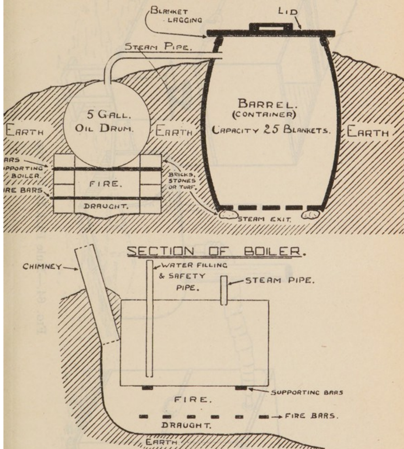
FIG. 63.—Serbian Barrel Disinfector.
