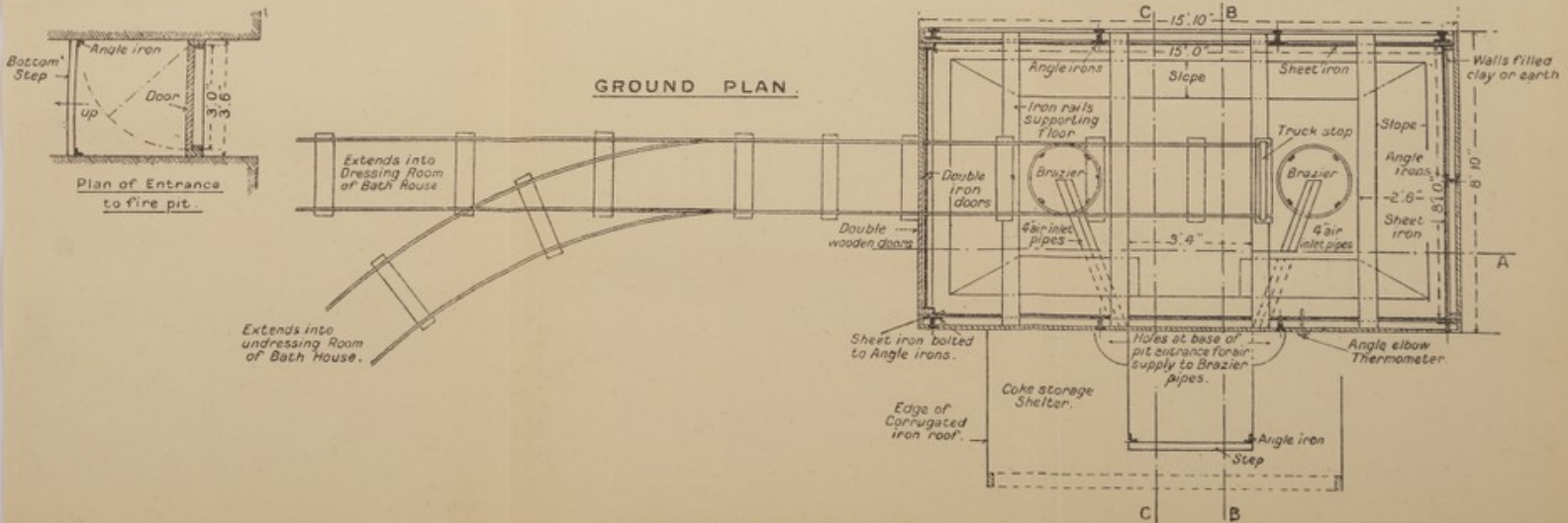
FIG. 60.—Orr's hut. Hot air disinfestor.
