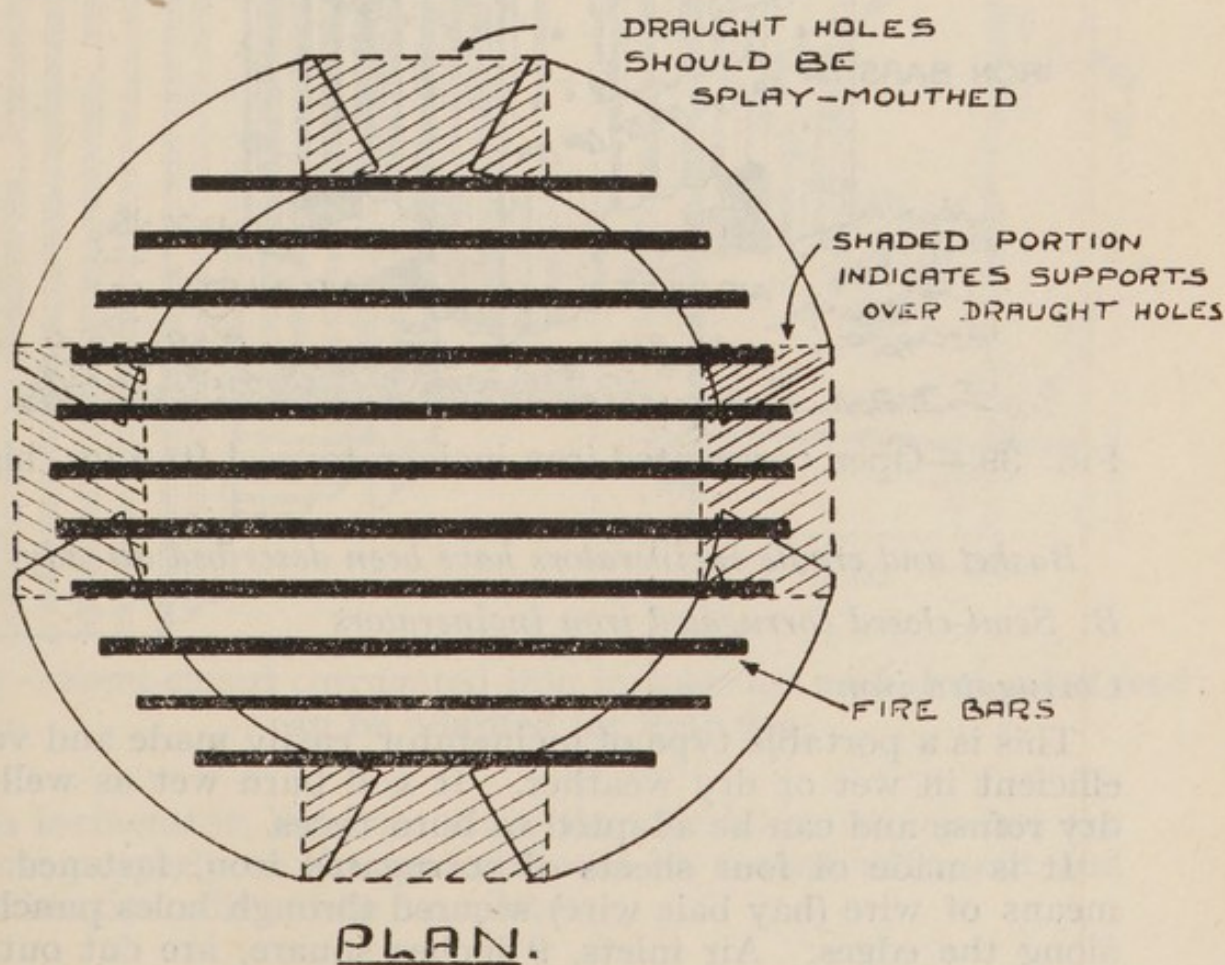
FIG. 38.—Open circular turf incinerator.
