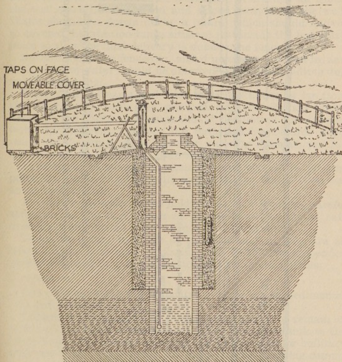
FIG. 7.—Protection of a well.
