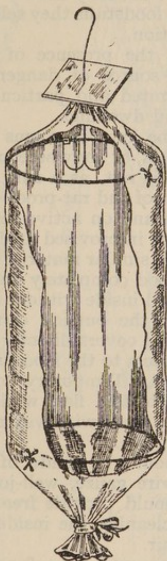
FIG. 13.—Improvised fly-proof larder.
