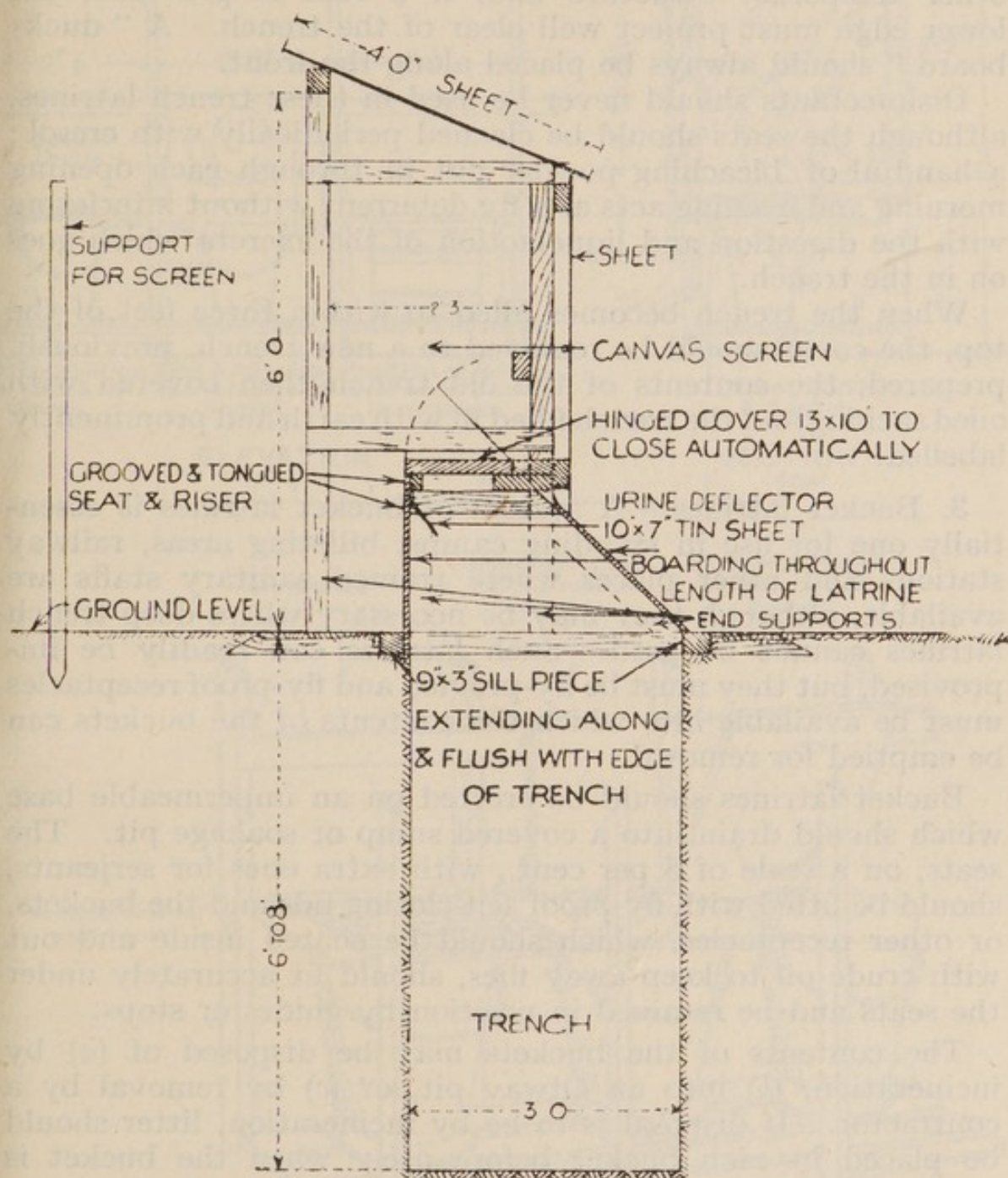
FIG. 24.—Deep trench latrine.
