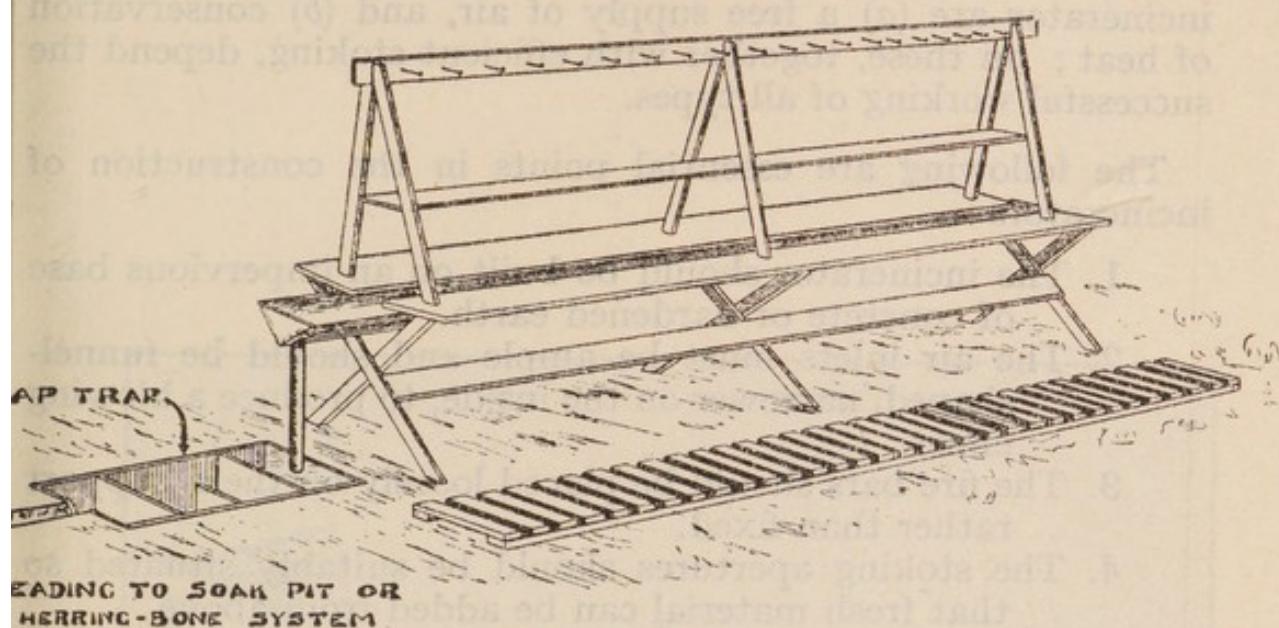
FIG. 35.—Ablution bench.
