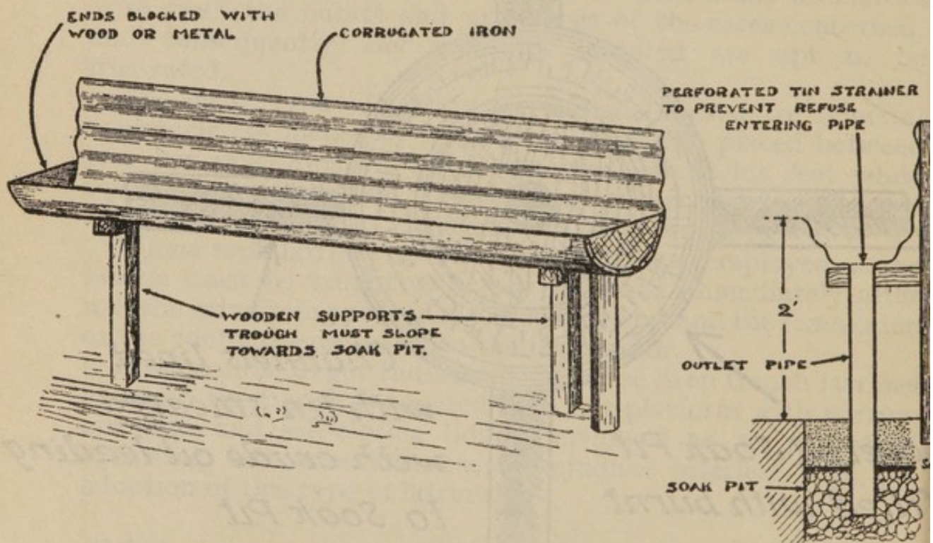
FIG. 27.—Trough urinal.
