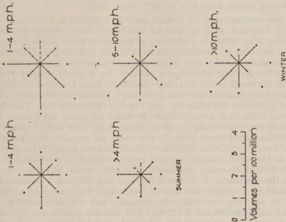
FIG. 3.47(b) SULPHUR DIOXIDE.
