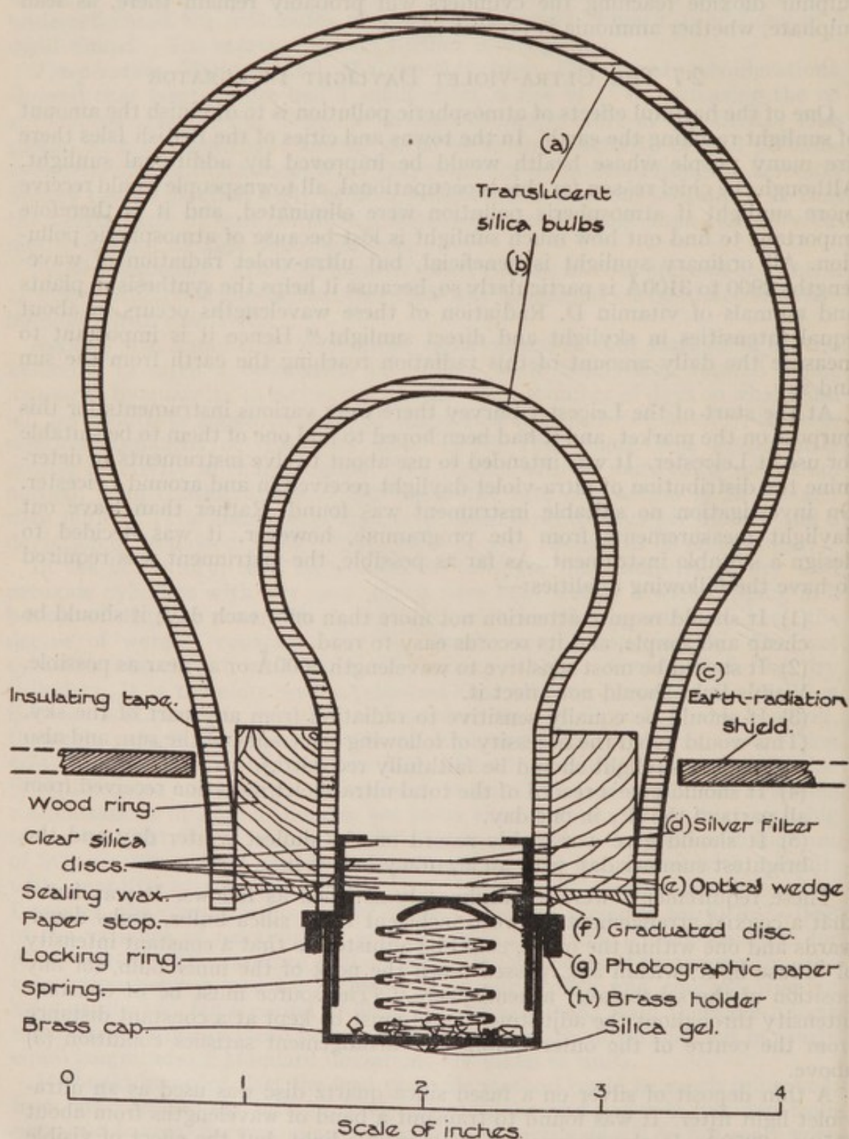
FIG. 2.7 ULTRA-VIOLET DAYLIGHT INTEGRATOR.
