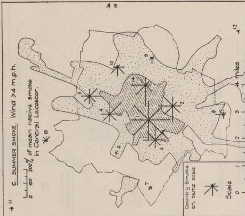
FIG. 3-48(c) NATIVE LEICESTER SMOKE—MODERATE WINDS > 4 M.P.H.—SUMMER.
