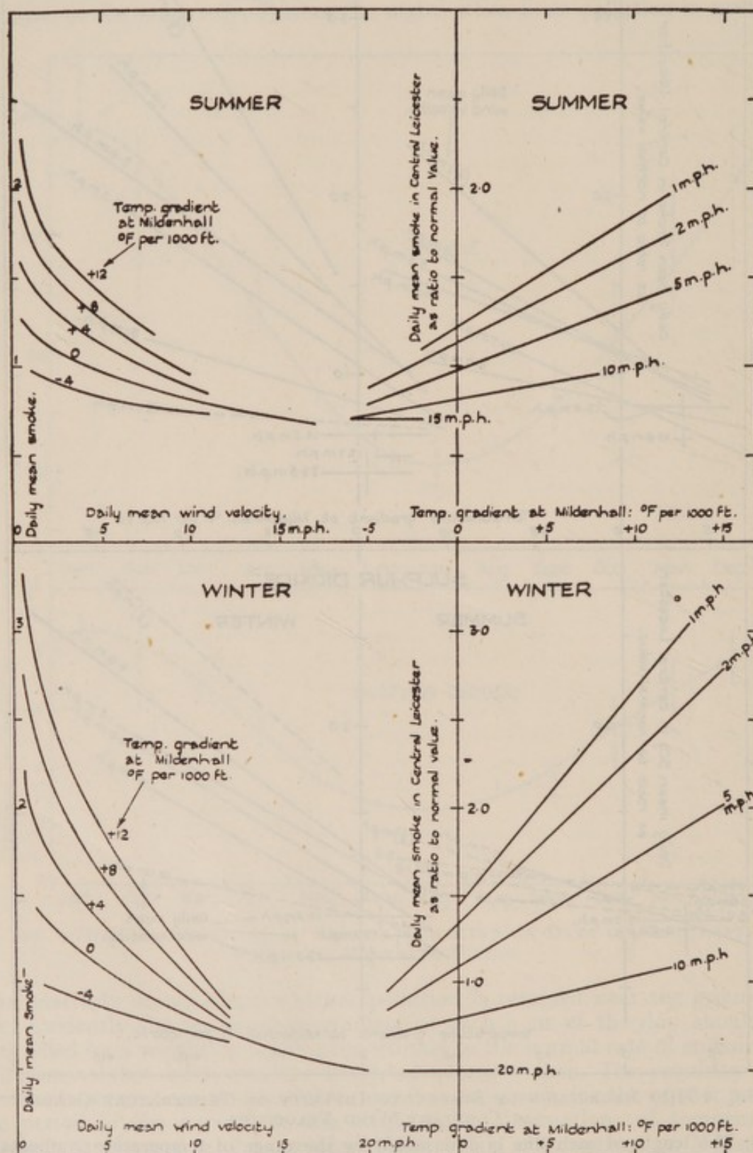
FIG. 4-71(c) DEPENDENCE OF SMOKE ON WIND VELOCITY AND TEMPERATURE GRADIENT.
