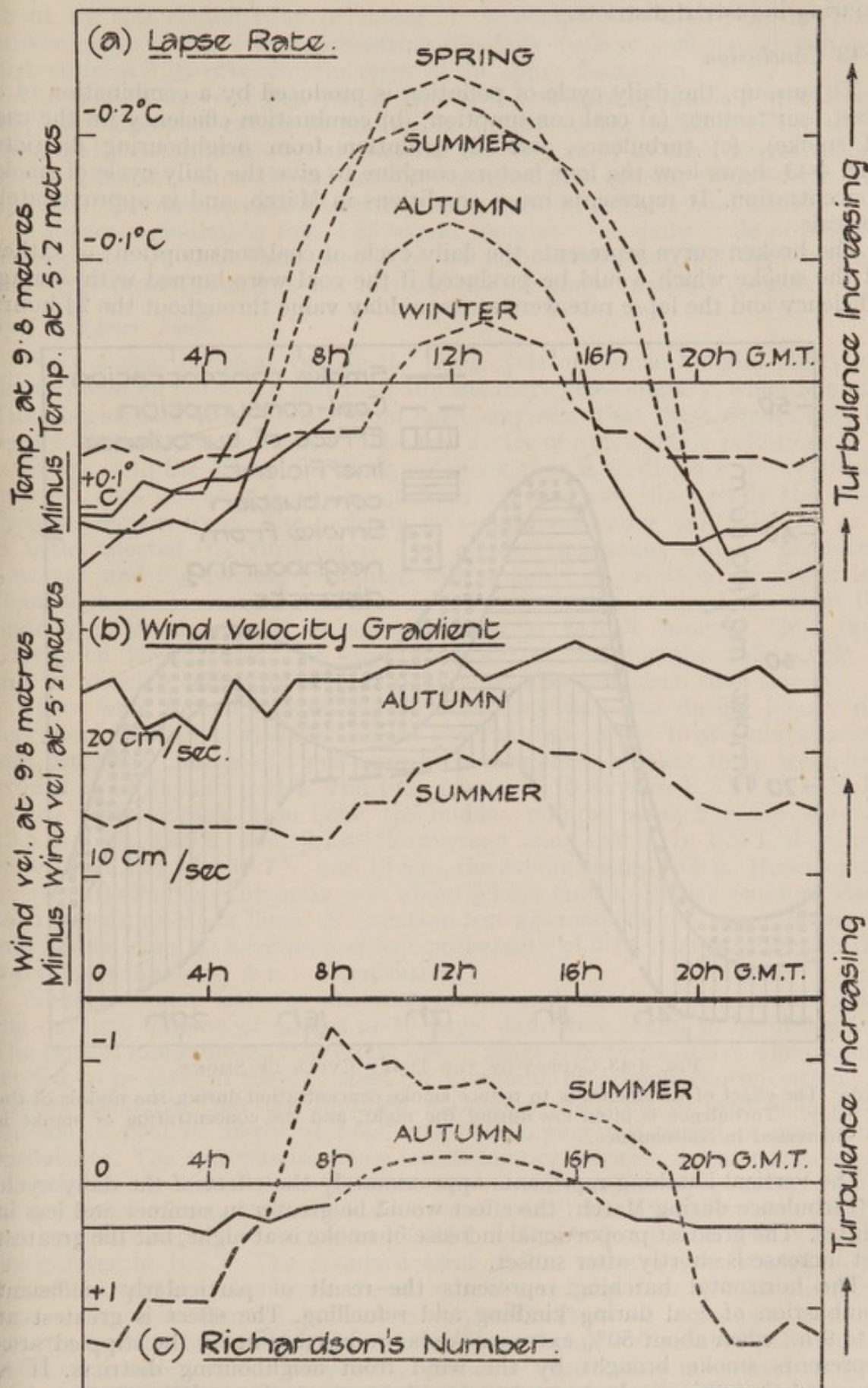
FIG. 4.42 DAILY CYCLE OF ATMOSPHERIC TURBULENCE.
