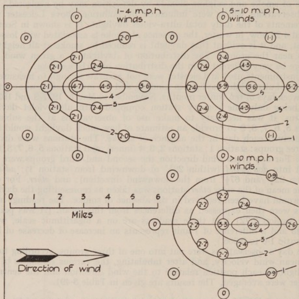
FIG. 3.491 EFFECT OF WIND VELOCITY ON ULTRA-VIOLET DAYLIGHT.
