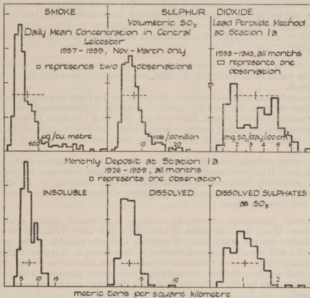
FIG. 4.5 FREQUENCY DISTRIBUTION OF POLLUTION.
