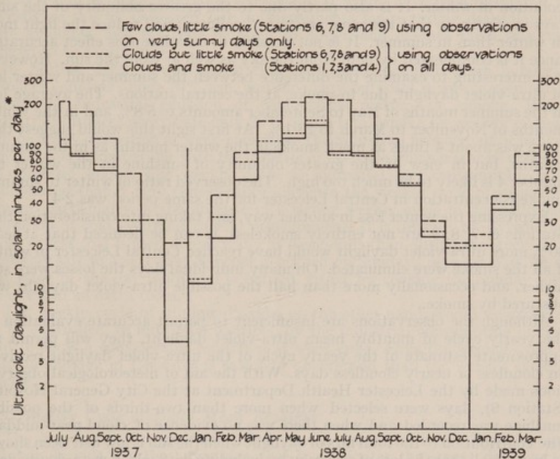
FIG. 4.23 THE MARCH OF ULTRA-VIOLET DAYLIGHT AT LEICESTER.
