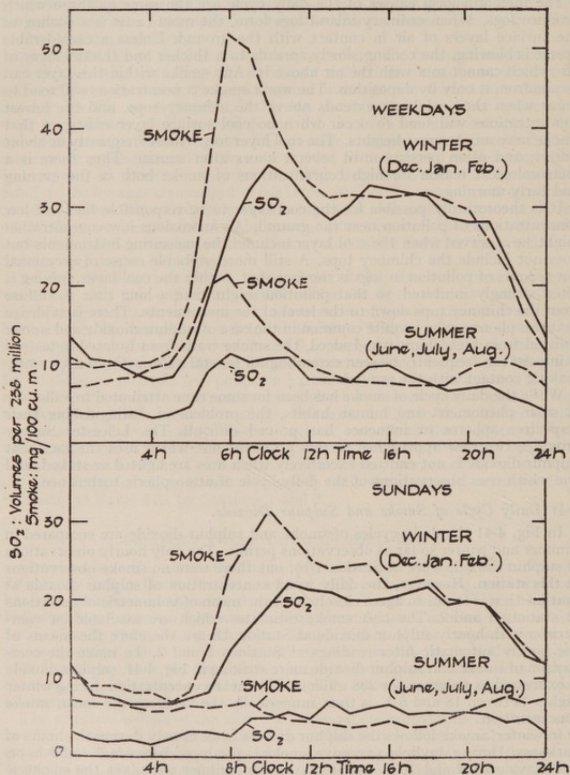
FIG. 4.41 DAILY CYCLE OF SMOKE AND SULPHUR DIOXIDE.
