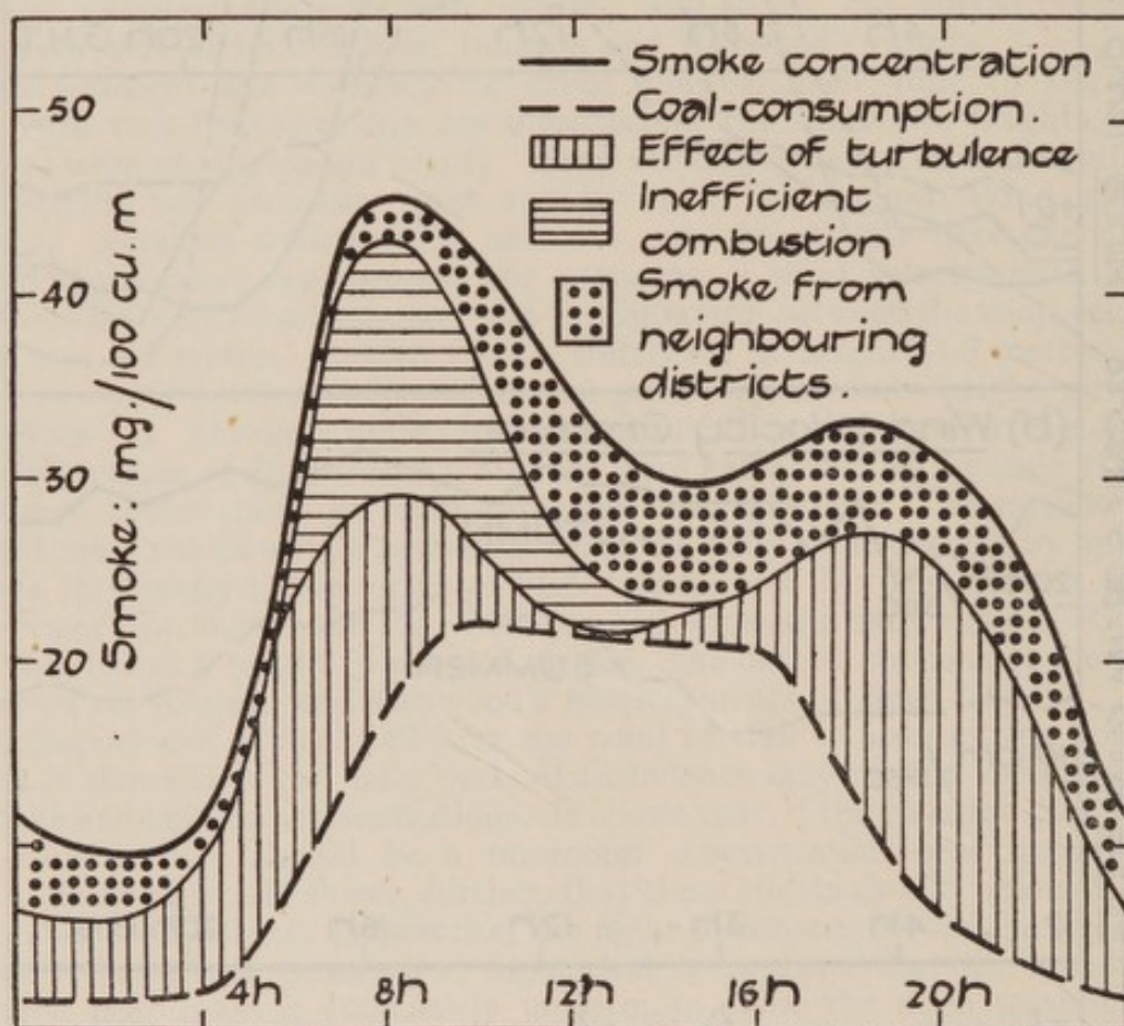
FIG. 4.43 CAUSES OF THE DAILY CYCLE OF SMOKE.
