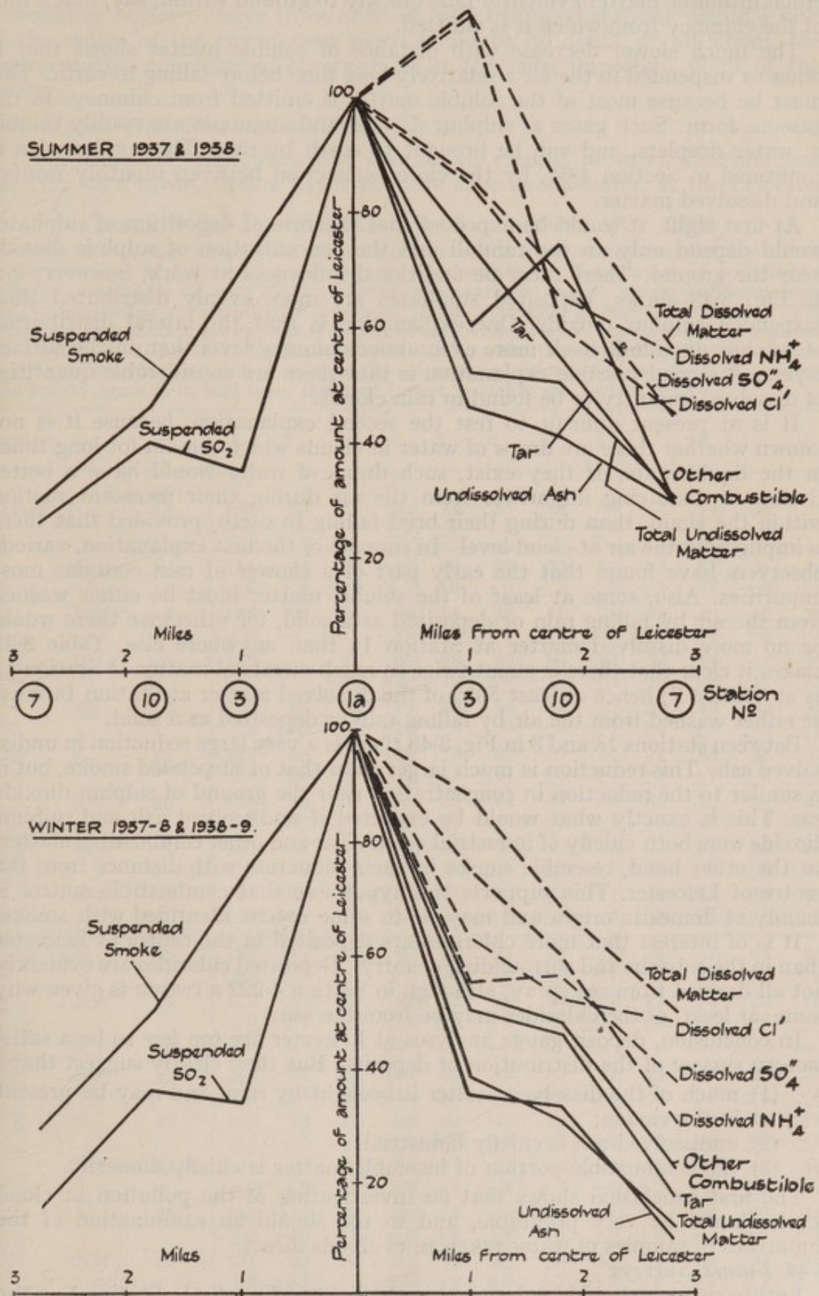
FIG. 3.43 VARIATION OF DEPOSITED MATTER ACROSS LEICESTER.
