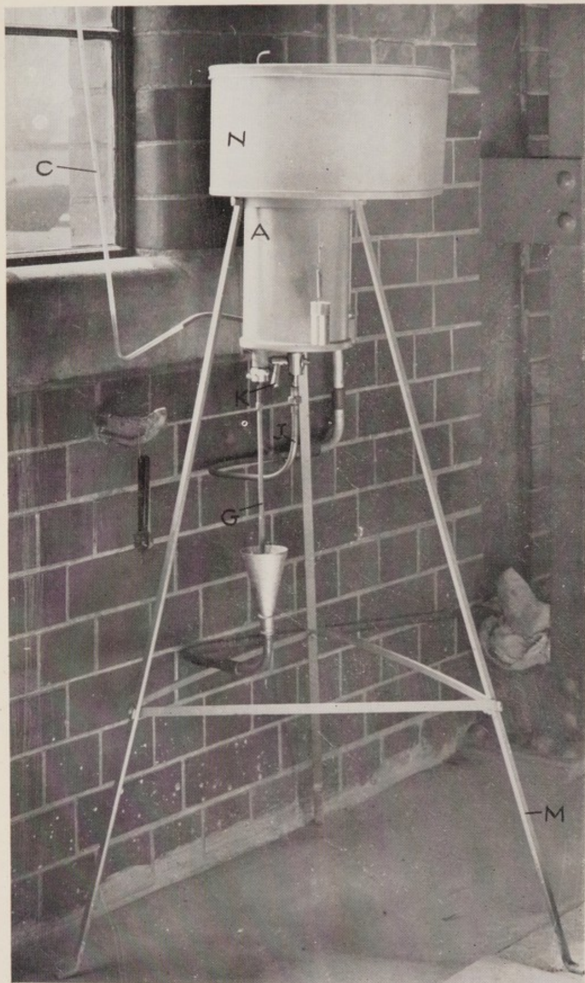
AUTOMATIC FILTER.
