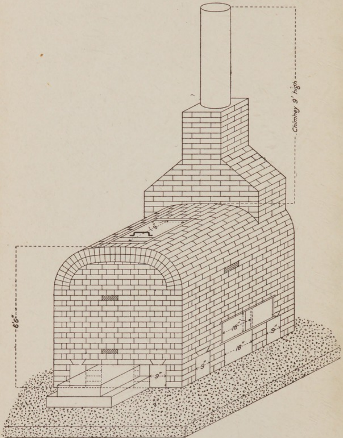
FIG. 32.—Perspective Elevation of Brick Destructor.
