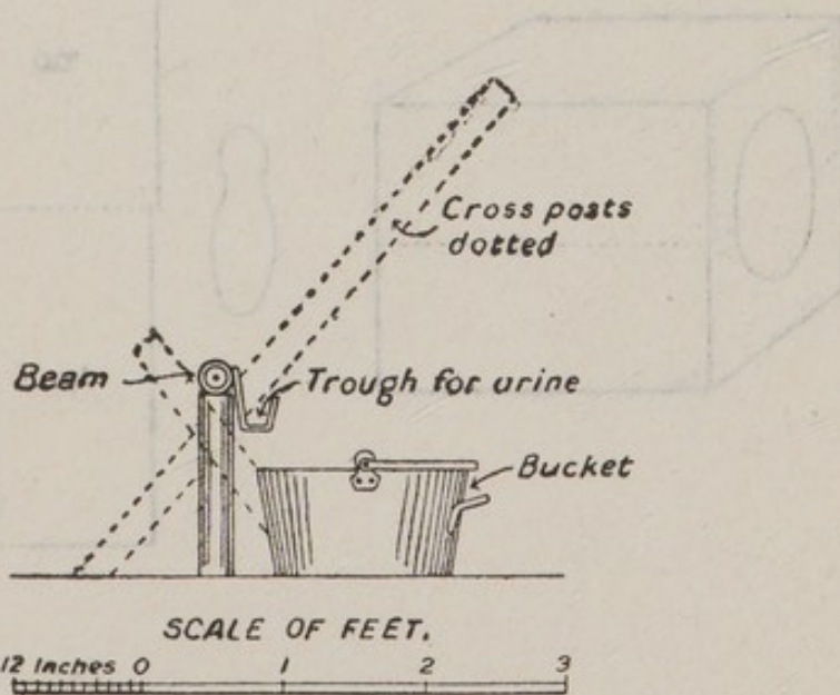
Detail section through urine trough.
