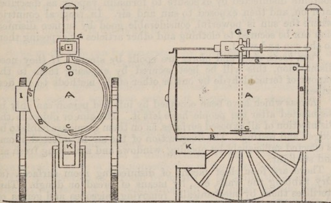
FIG. 63.—PORTABLE STEAM DISINFECTING APPARATUS.
