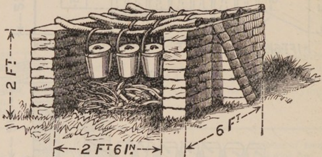
FIG. 33.—WALL KITCHEN WITH KETTLES, TO SHOW DIMENSIONS.
