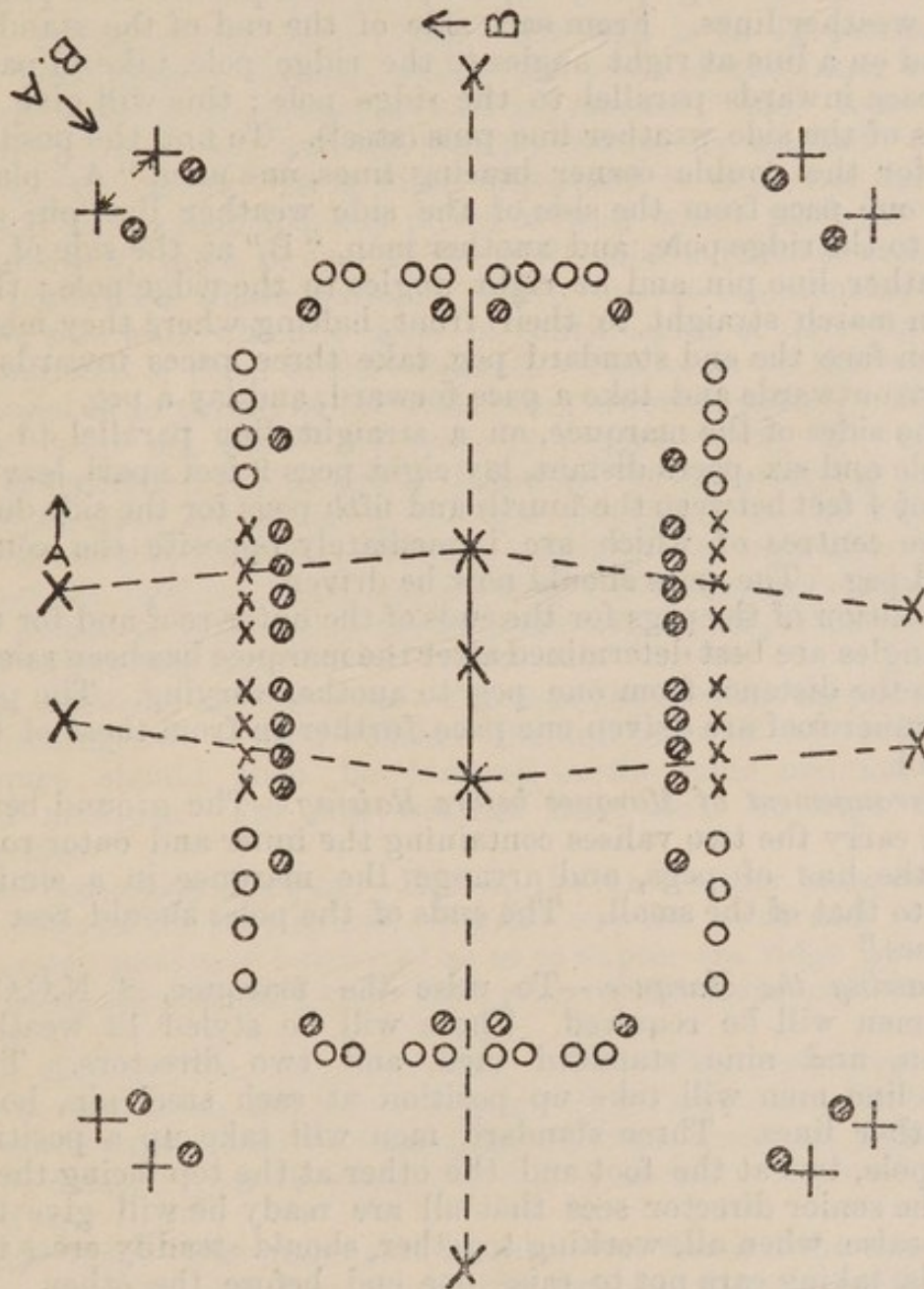
FIG. 31.—GROUND PLAN OF PEGS OF MARQUEE (LARGE).
