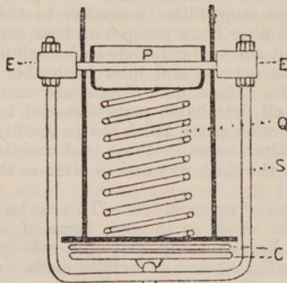
FIG. 62—VALVE OF GRIFFITH WATER STERILIZER.
