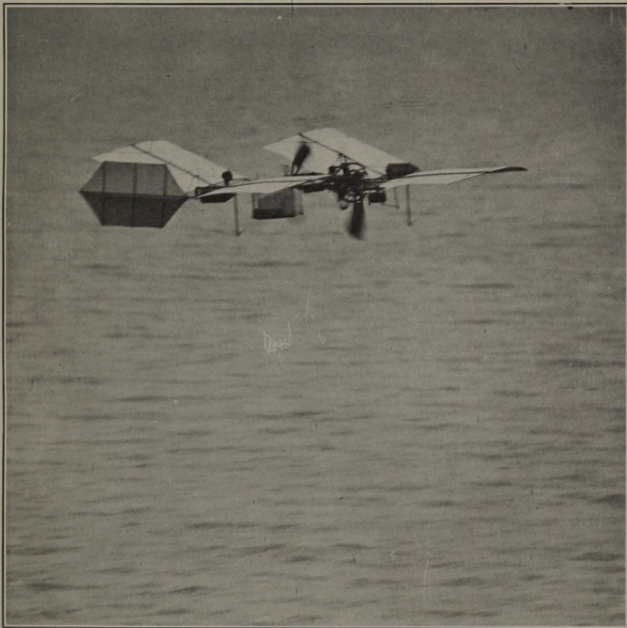
QUARTER-SIZE GASOLINE MODEL, LANGLEY AERODROME, IN ONE OF ITS FLIGHTS OF AUGUST 8, 1903, ON THE POTOMAC RIVER.
