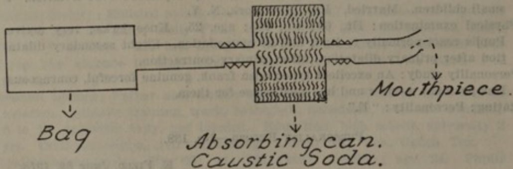
SIMPLE FORM OF REBREATHING APPARATUS.
