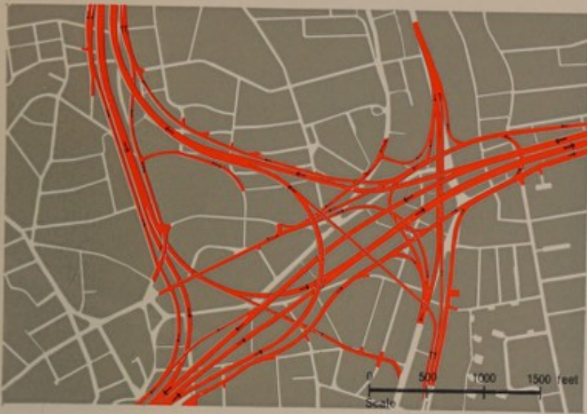
242 An interchange planned for the Inner Loop at Boston. It occupies about 100 acres. Compared with this, the interchanges shown in the examples worked out in Chapter III seem quite modest, yet they may be as much as British cities can stand of this space-taking engineering.
