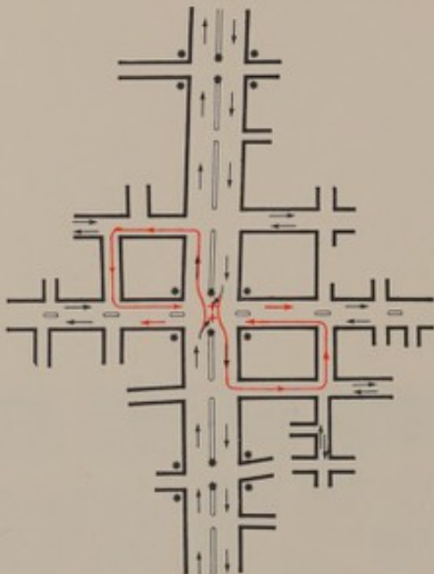
52 A typical traffic management measure. The difficult right-hand turns out of the main route are prohibited at the points marked by red crosses, and are replaced by left-hand turns which take traffic round the block (as shown in red) to a straight cross-over of the main route.
