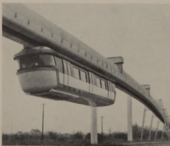
34 The experimental monorail track of S.A.F.E.G.E. TRANSPORT near Paris. The car is suspended from rubber tyred bogies running inside the duct, and operation is thus silent and impervious to weather.
