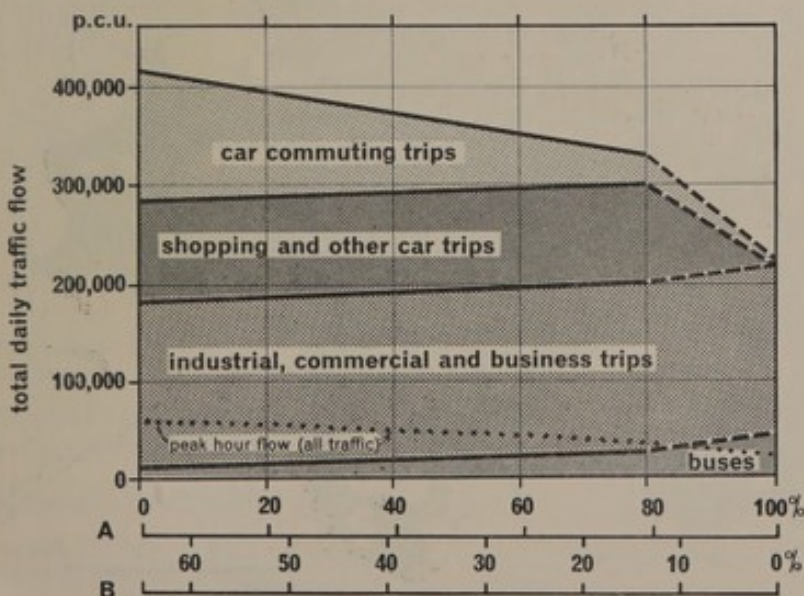
A degree of restriction on use of car B proportion of all persons travelling to work who go by car
