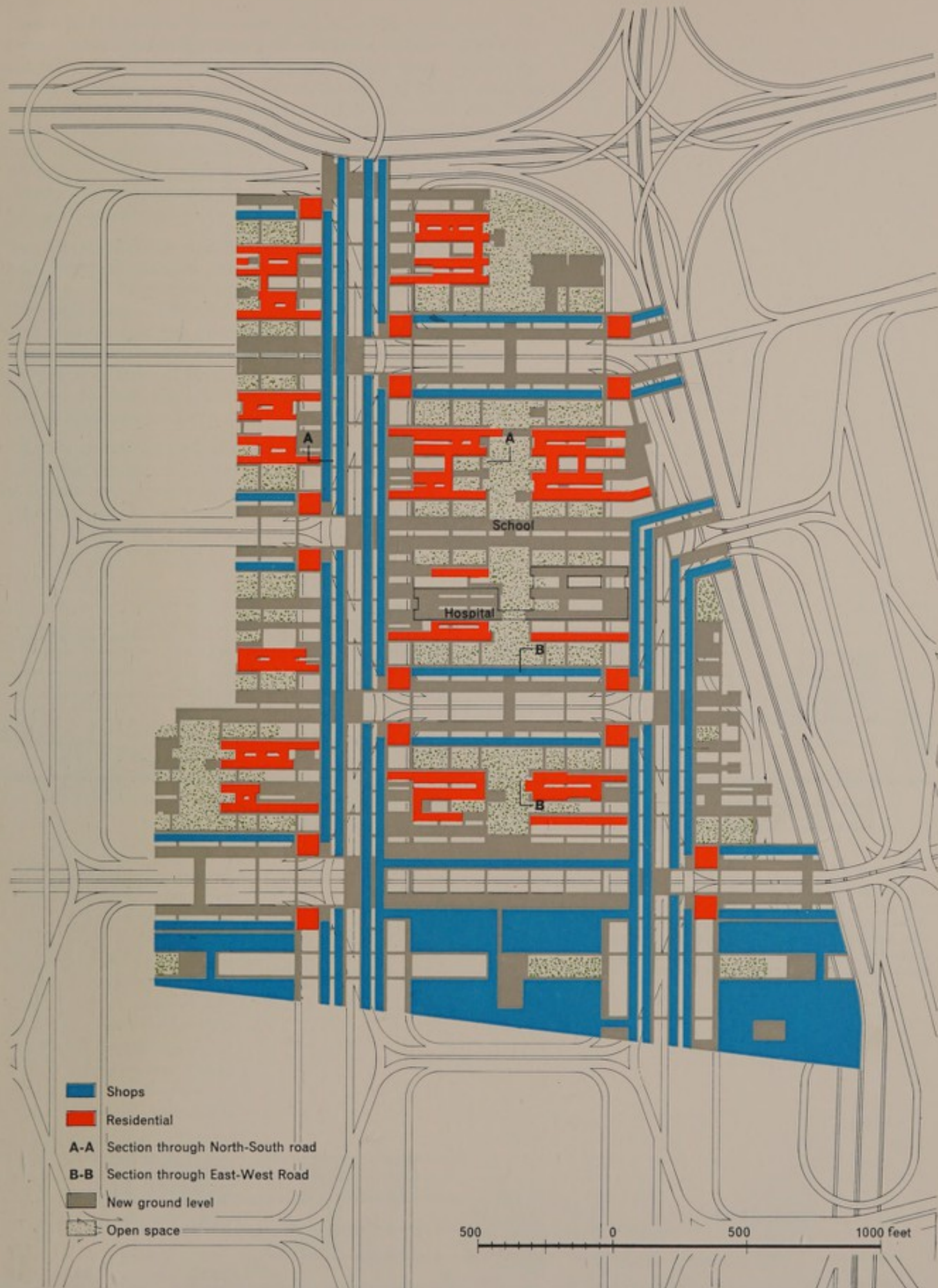
182 The design for complete redevelopment—plan showing the broad disposition of uses at deck level. Sections A-A and B-B refer to Figures 183 and 184. Areas on the new ground level which are not indicated for shops or residential use are for office, commercial and industrial purposes.
