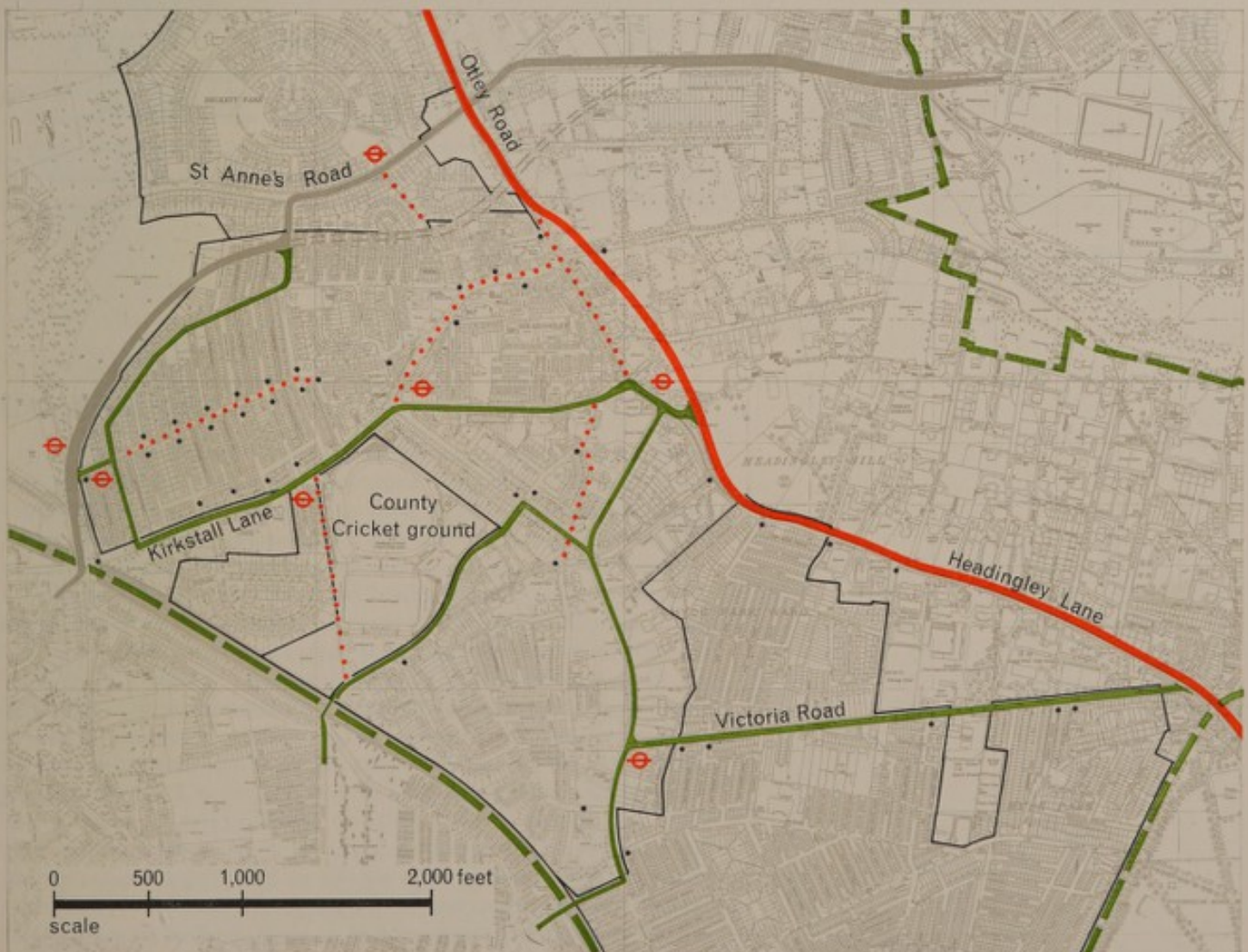
142 Some possible immediate steps in environmental management for the Headingley area, including a by-pass to the shopping centre. Otley Road and Headingley Lane are retained for the time being as a primary distributor.
