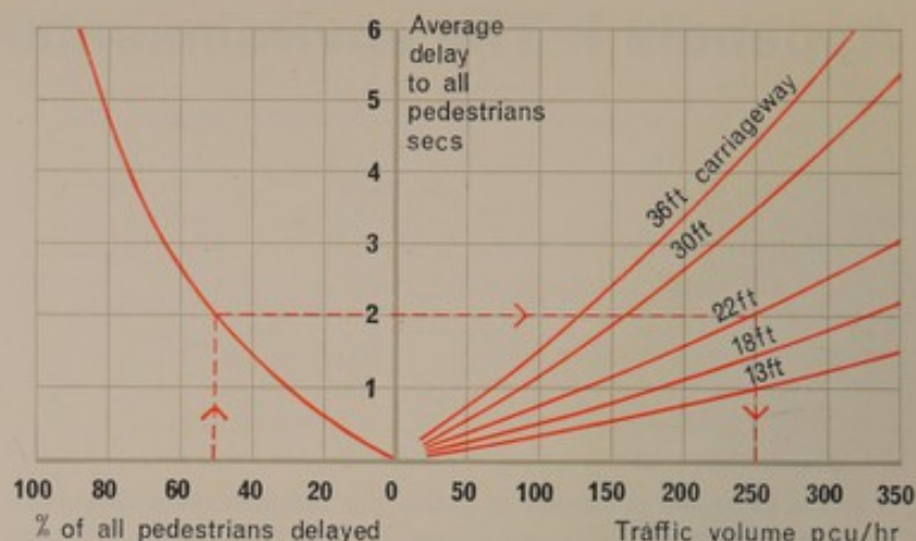
1 These two graphs show the relationship between traffic volume, average delay to all pedestrians and the proportion of all pedestrians delayed. The dotted line picks out the case referred to in paragraph 7.
