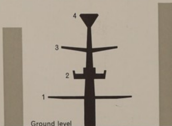
206 The proposal by Mr Rigby Childs for a free-standing pedestrian walk in Oxford Street. This is a cross-sectional view with existing buildings on either side. The ground level would be wholly available for two carriageways of traffic. Level 1 is the pedestrian platform. Level 2 is the two-way travelator with canopy over at 3. At level 4 there is a longitudinal structural member for stability.
