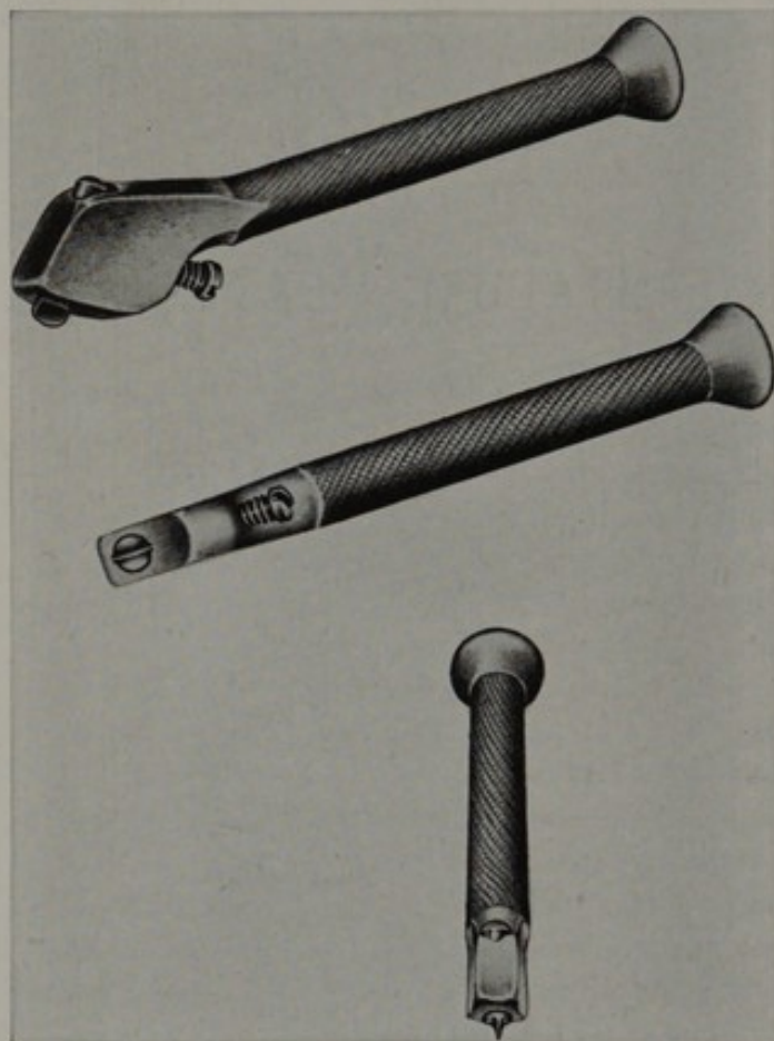
FIGURE 111.—An adjustable lineator devised by the author.
