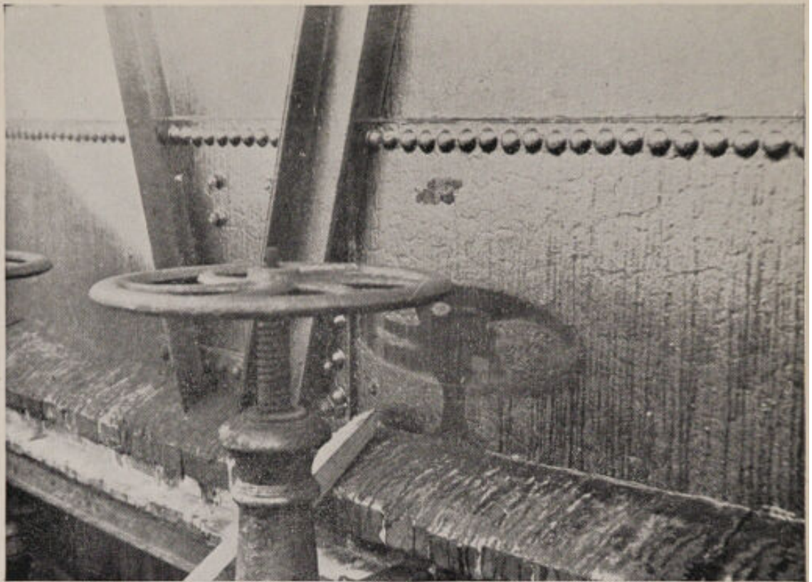
Photo No. 23. HIROSHIMA. Shadow cast by valve-wheel on side of gasholder 1\frac{1}{4} miles from the centre of damage. The bituminous coating on the steel plates was affected by heat radiation except where shielded by the wheel and spindle. See paragraph 53.
