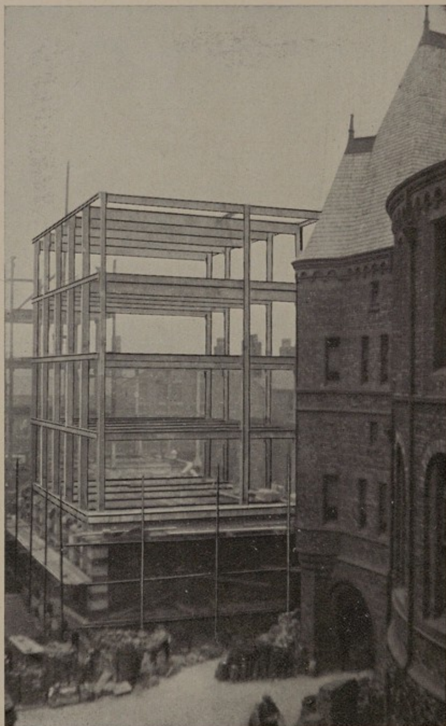
FIRST WING OF THE NEW NURSES' HOME, IN COURSE OF CONSTRUCTION.
