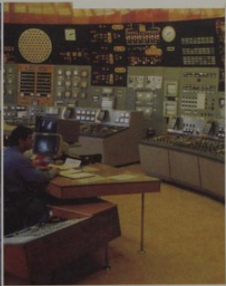
Paks MTR, training on main cooling pump
