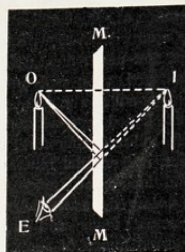
FIG. 230.—FORMATION OF IMAGE BY A PLANE MIRROR.
