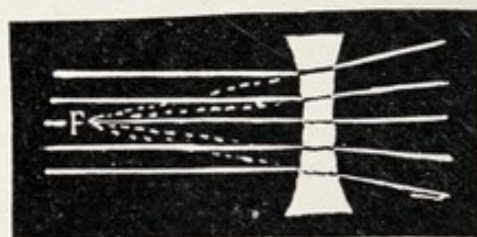
FIG. 242.—THE ACTION OF A CONCAVE LENS ON PARALLEL RAYS.
