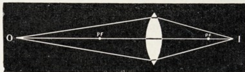
FIG. 245.—CONJUGATE FOCI OF A CONVEX LENS.
