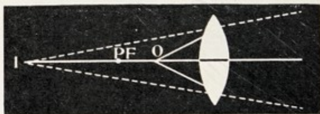
FIG. 246.—VIRTUAL FOCUS OF A CONVEX LENS.
