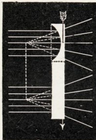
FIG. 253.—THE ACTION OF A CONCAVE CYLINDRICAL LENS UPON PARALLEL RAYS.
