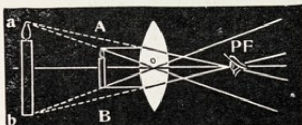
FIG. 249.—VIRTUAL IMAGE FORMED BY A CONVEX LENS.
