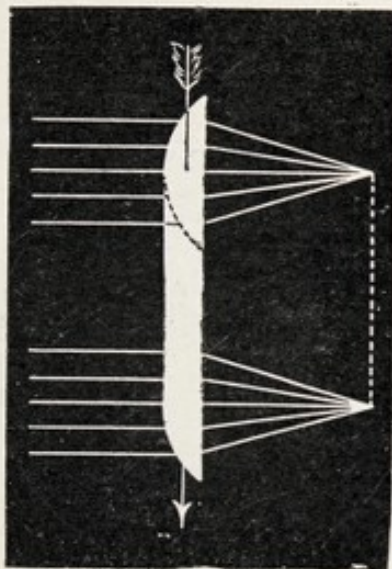
FIG. 252.—THE ACTION OF A CONVEX CYLINDRICAL LENS UPON PARALLEL RAYS.
