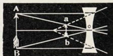
FIG. 250.—VIRTUAL IMAGE FORMED BY A CONCAVE LENS.
