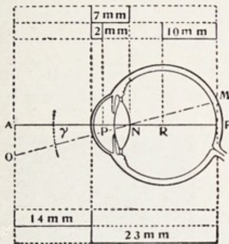
FIG. 258. — CARDINAL POINTS OF THE EYE.
