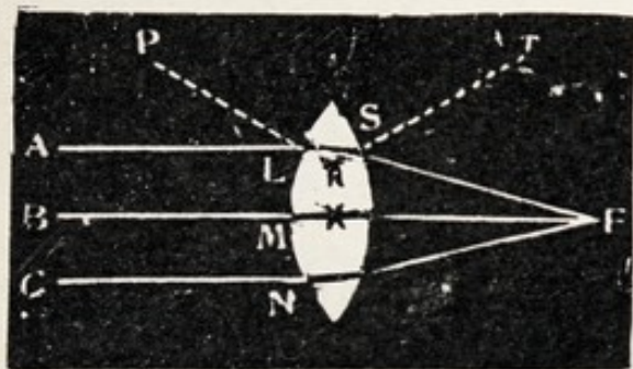
FIG. 244.—THE PRINCIPAL FOCUS OF A CONVEX LENS.
