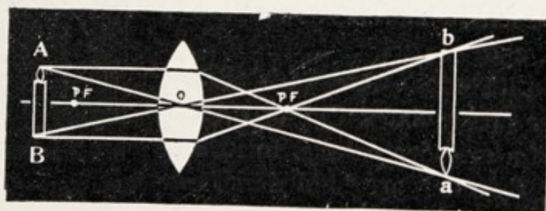
FIG. 248.—REAL, INVERTED, AND ENLARGED IMAGE FORMED BY A CONVEX LENS.
