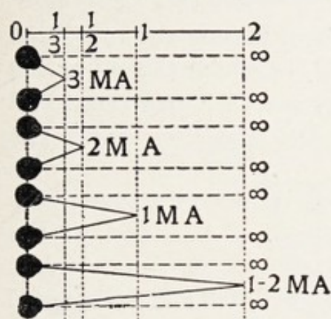
FIG. 263.—DIAGRAM ILLUSTRATING THE UNIT OF CONVERGENCE, THE METRE ANGLE.
