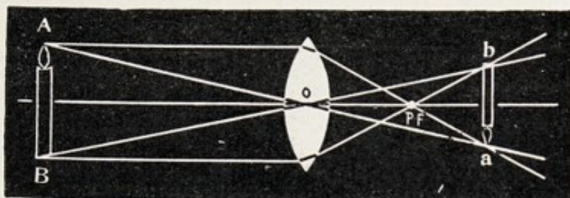
FIG. 247.—REAL, INVERTED, AND REDUCED IMAGE FORMED BY A CONVEX LENS.
