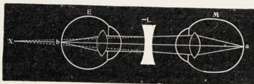
FIG. 267.—THE ESTIMATION OF MYOPIA BY THE DIRECT METHOD OF OPHTHALMOSCOPY.
