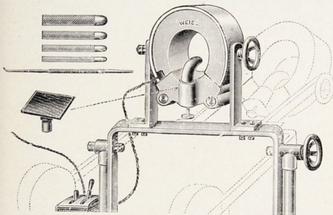
FIG. 193.—MELLINGER'S RING MAGNET.
