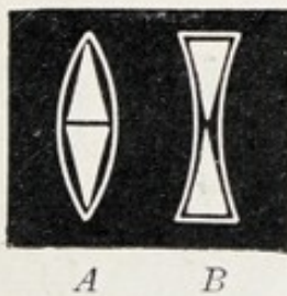
FIG. 238.—THE FORMATION OF LENSES BY PRISMS.
