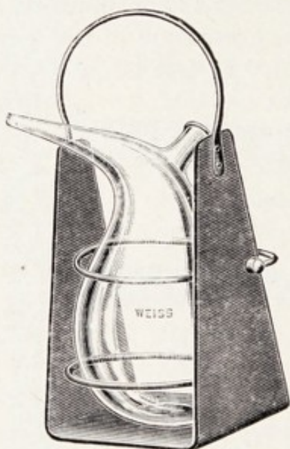
FIG. 202.—UNDINE IN STAND.
