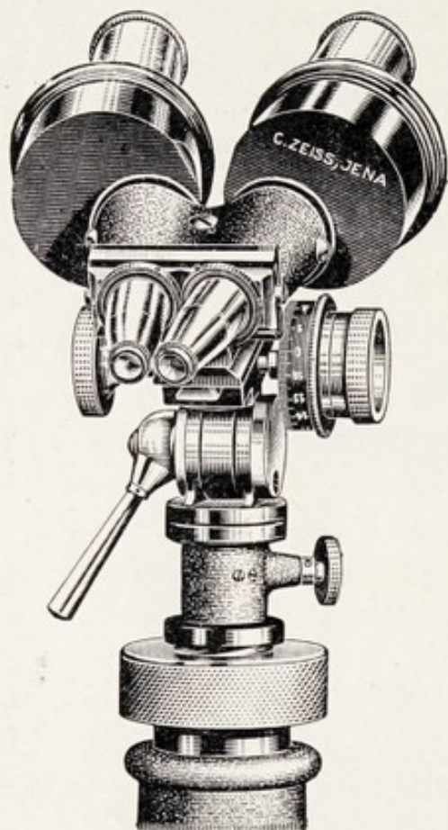
FIG. 48B. — MICROSCOPE HEAD WITH DR. ULBRICH'S GRADUATED DRUM ATTACHED.
