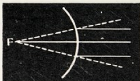
FIG. 232.—REFLECTION BY A CONVEX MIRROR.
