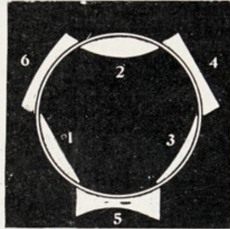
FIG. 237.—THE RELATION OF THE SURFACES OF LENSES TO SPHERES.
