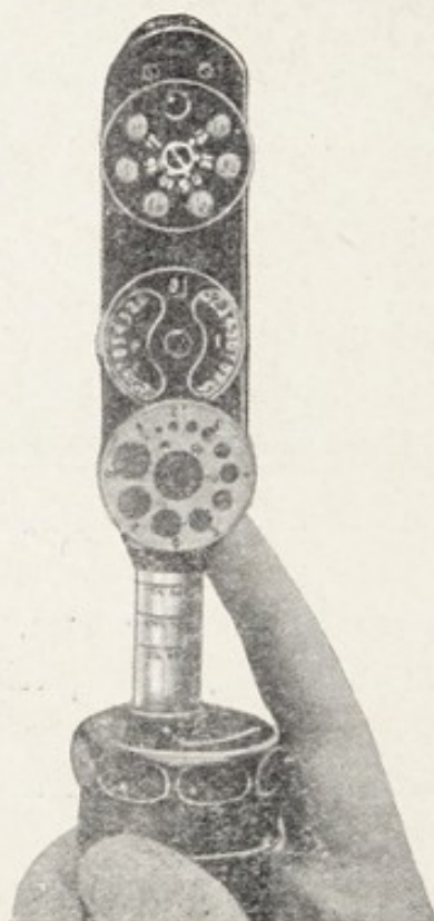
FIG. 23.—OPHTHALMOSCOPE OF MORTON TYPE, SELF LUMINOUS.
