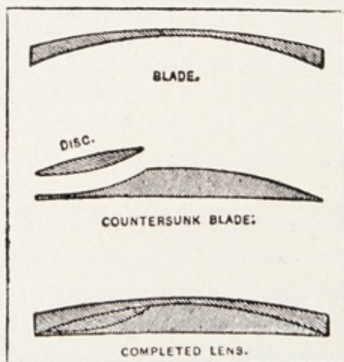
FIG. 297.—SECTION SHOWING THE CONSTRUCTION OF THE INVISIBLE BIFOCAL LENS.
