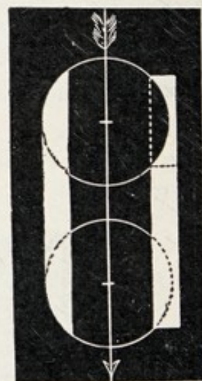
FIG. 251.—THE CONSTRUCTION OF A CONVEX AND A CONCAVE CYLINDRICAL LENS FROM A CYLINDER.
