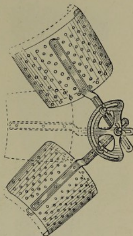
FIG. 16.—STILLMANN'S SECTOR JOINT.
