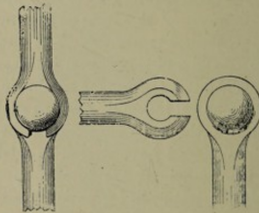
FIG. 10.—KEYHOLE CATCH JOINT. (AFTER HOFFA.)
