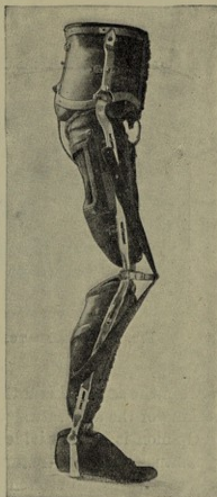
FIG. 22.—ARTIFICIAL QUADRICEPS.
