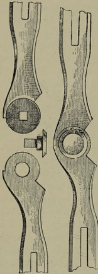
FIG. 9.—DOUBLE RULE JOINT. (AFTER HOFFA.)
