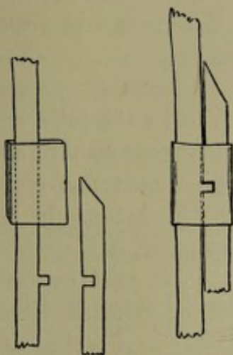
FIG. 11.—MORTICE JOINT.
