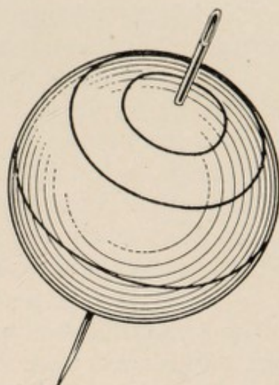
FIG. 28.—The Earth turning upon its Axis.
