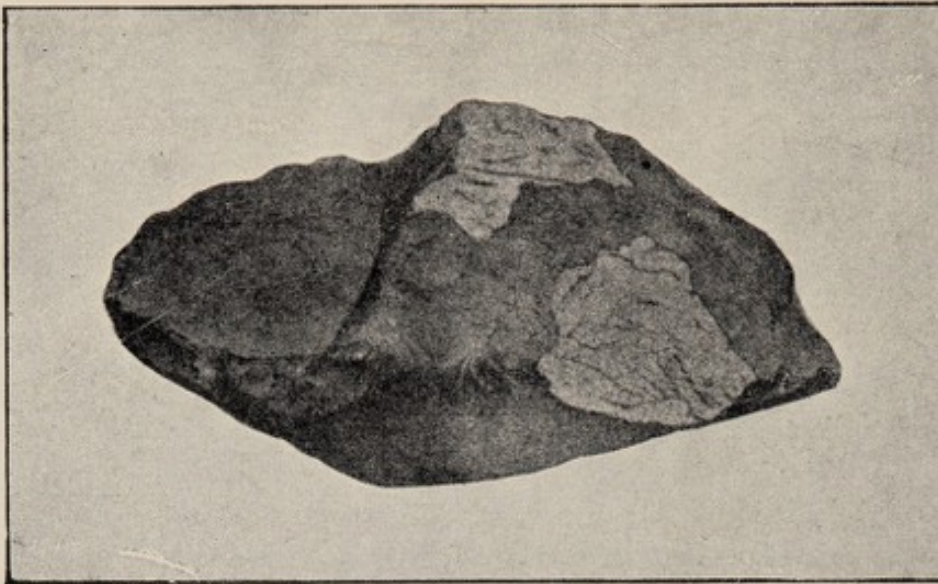
FIG. 40.—A Meteorite.
