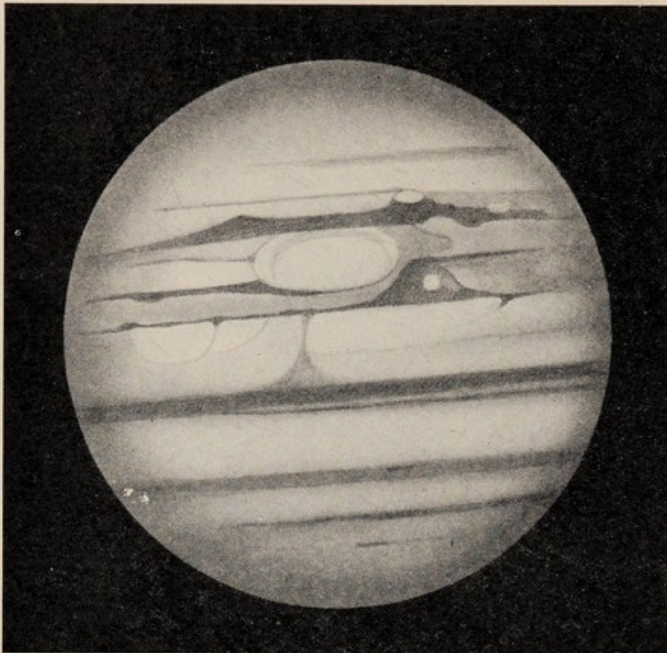
FIG. 22.—The Planet Jupiter, showing his belts and one of his eleven Satellites.
