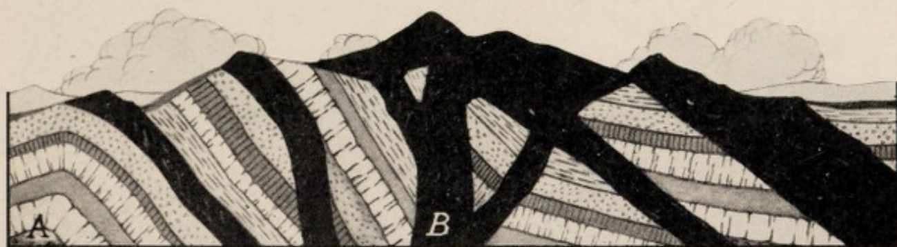
FIG. 51.—A, Stratified; B, Unstratified Rocks.
