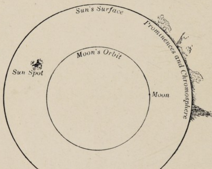
FIG. 37.—Dimensions of the Sun compared with the Moon's Orbit.
