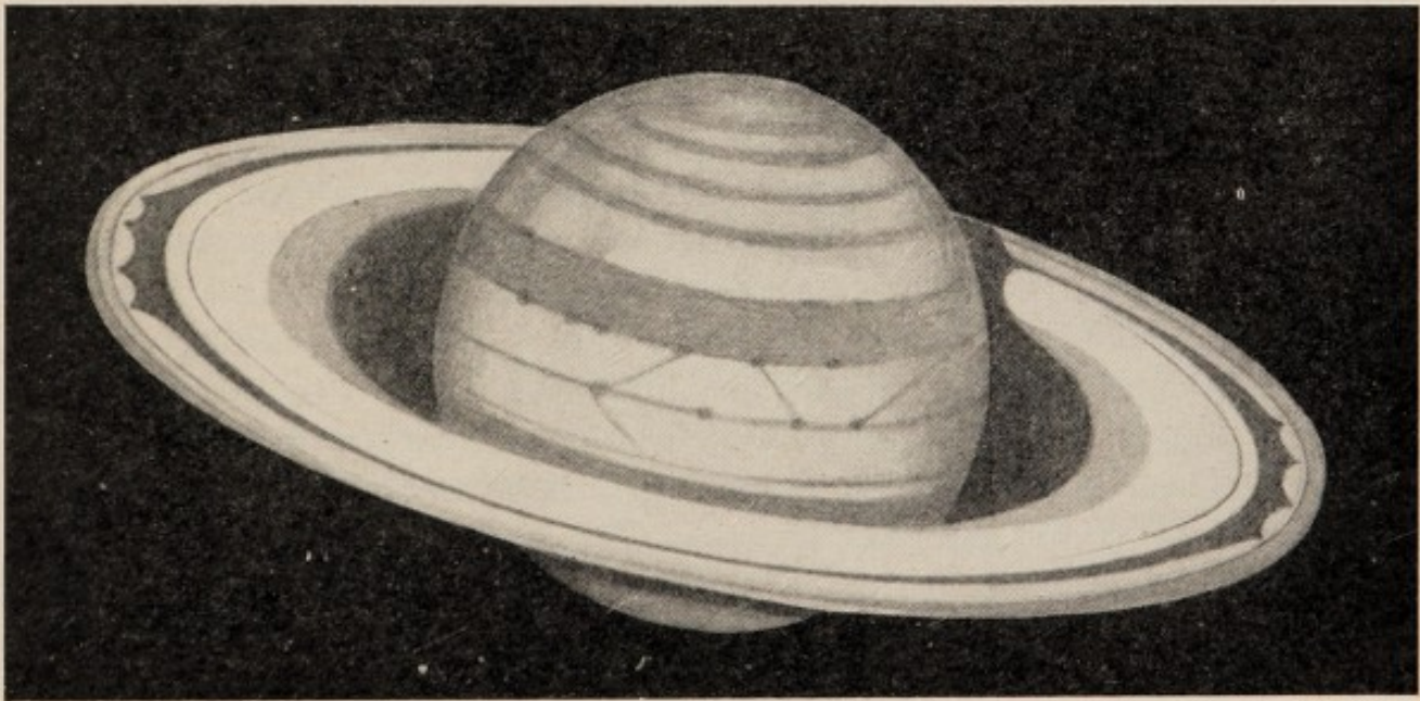
FIG. 23.—The Planet Saturn and his Rings.
