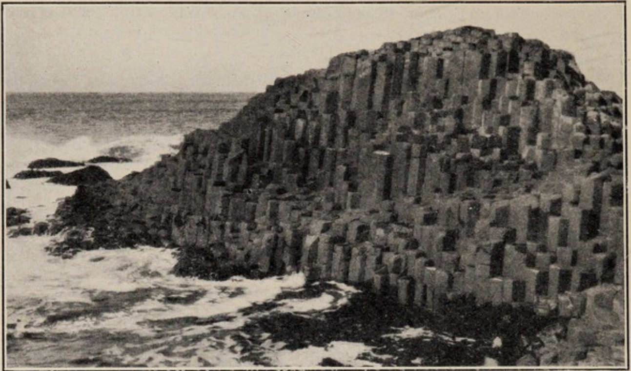
FIG. 52.—Basalt (the Giants' Causeway).
