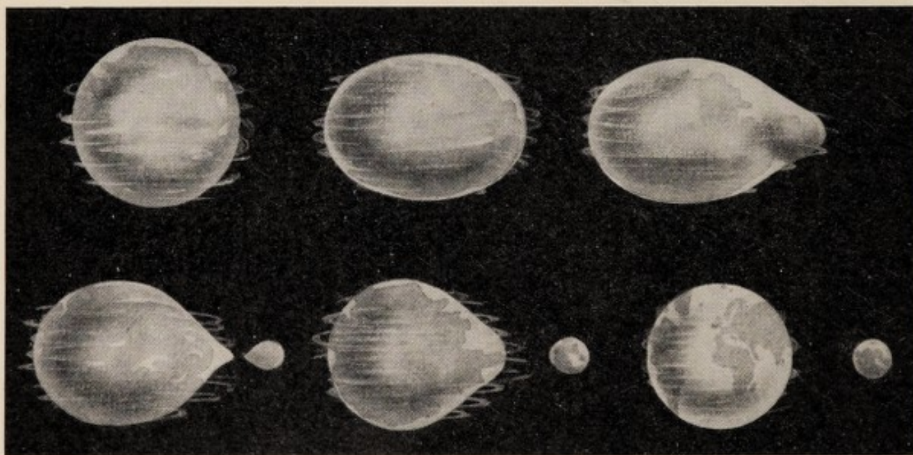
FIG. 30.—The Birth of the Moon.
