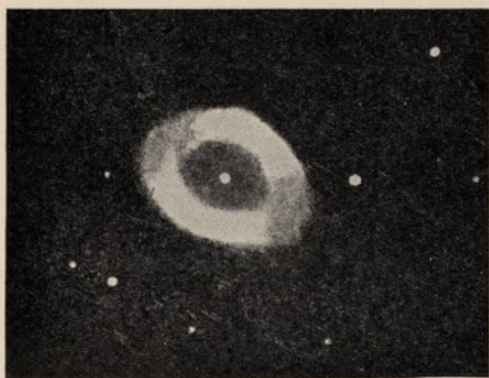
FIG. 46.—The Ring Nebula in Lyra. (Lick Observatory.)
