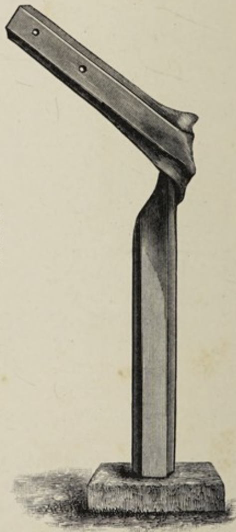
A T-iron (eight feet long, eight inches wide, and a quarter inch thick), used as a pedestal for a telegraph post. It was twisted by an elephant.
