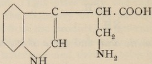
Indol-amino-methyl-acetic acid.
