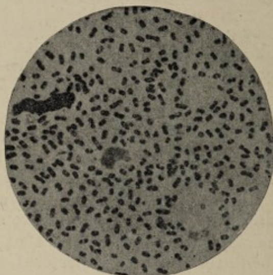
Fig. 138.—Bacillus of bubonic plague (Yersin).
