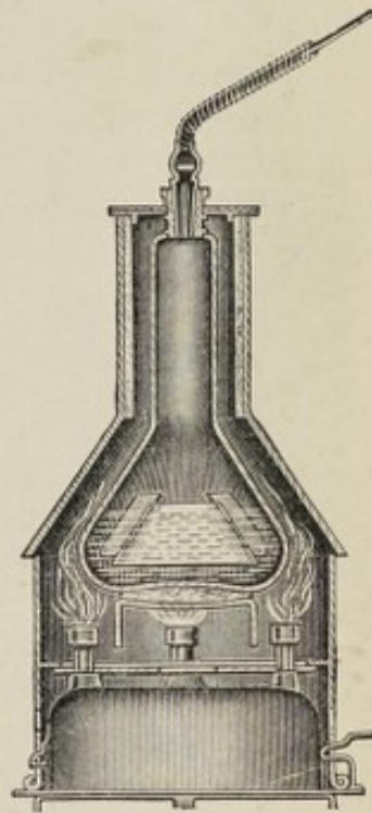
Fig. 19.—Trenner's formaldehyd gas regenerator.
