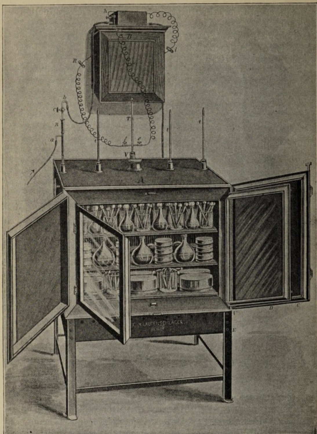
Fig. 36.—New model incubating oven with electro-regulator.
