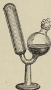
Fig. 5. — Smith's fermentation-tube.
