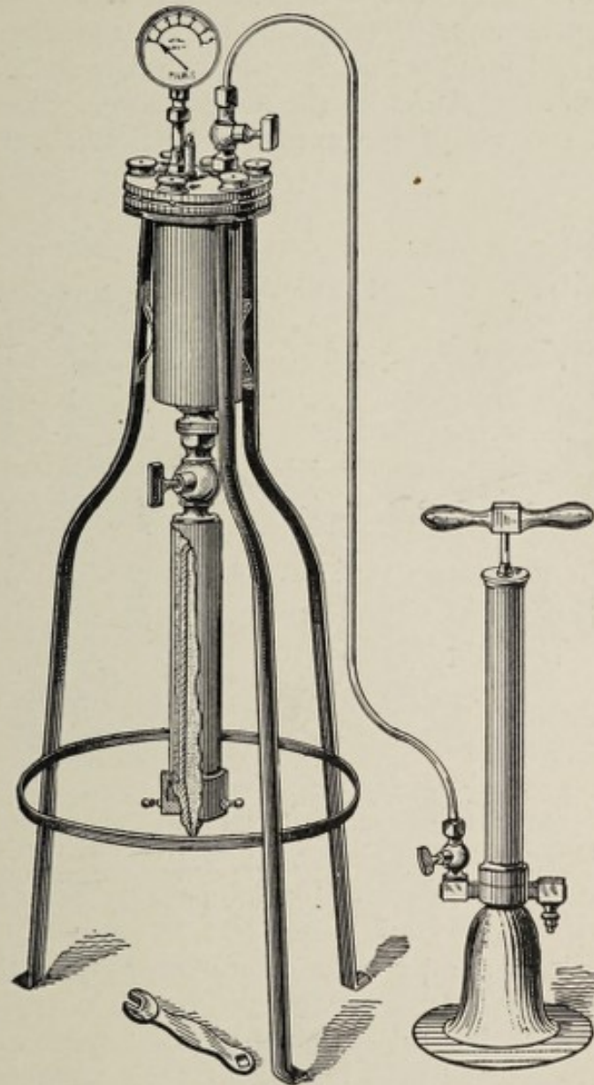
Fig. 15.—Pasteur-Chamberland filter arranged to filter under pressure.
