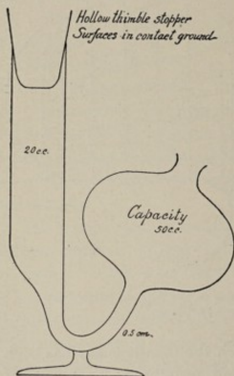
Fig. 7.—The Hill fermentation tube (Gorham).
