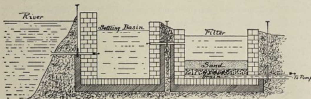
Fig. 168.—Cross-section of filter plant (after Hazen).
