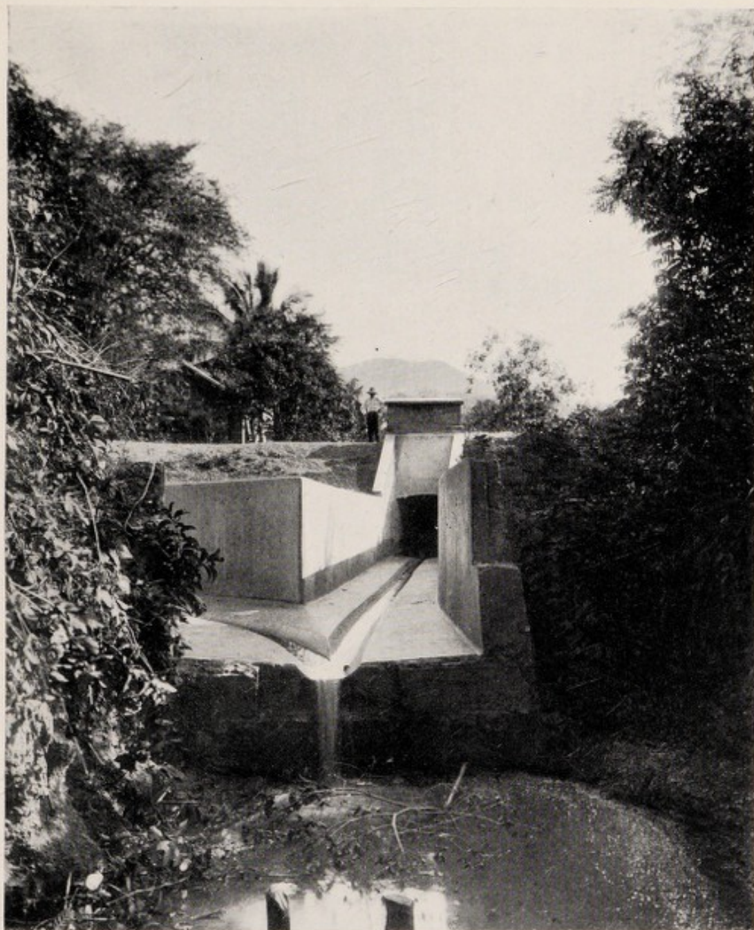
FIG. 28.—LARGE CONCRETE DRAINS, PORT OF SPAIN, TRINIDAD.
