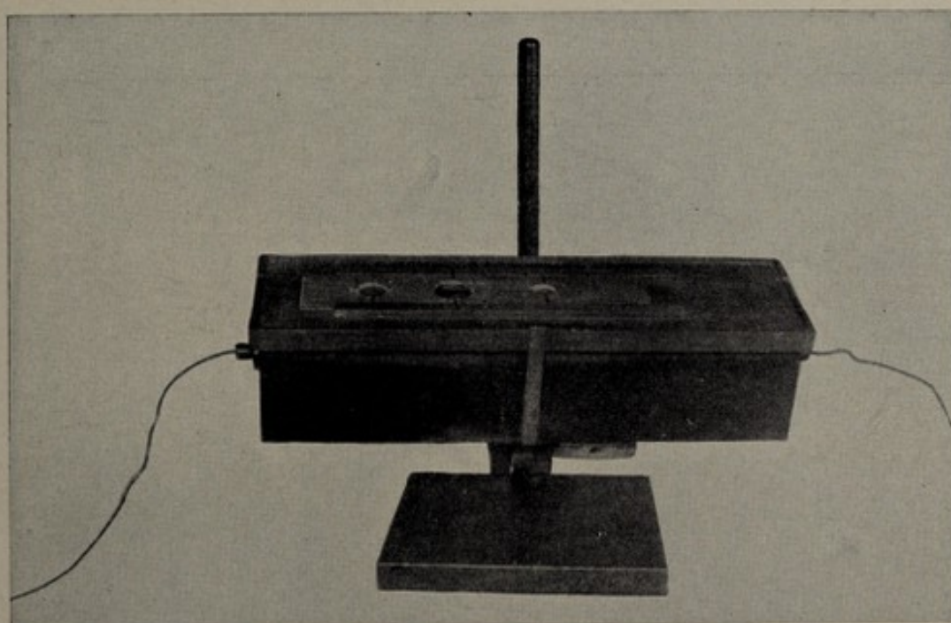
FIG. 45. The same box as shown in Fig. 43, with cover closed. The thin aluminum screen 15 cm. wide which fits across and close to the cover over the circular opening is not shown.
