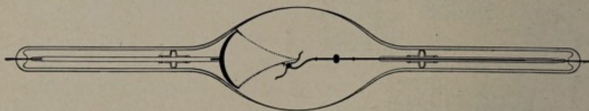
FIG. 24. A. W. L. rotary target tube with movable target. (Rollins.)
