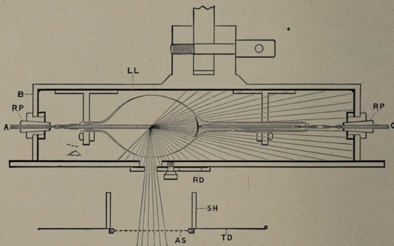
FIG. 31. Illustrates the formation of the cathode stream and X-rays. (Rollins.)
