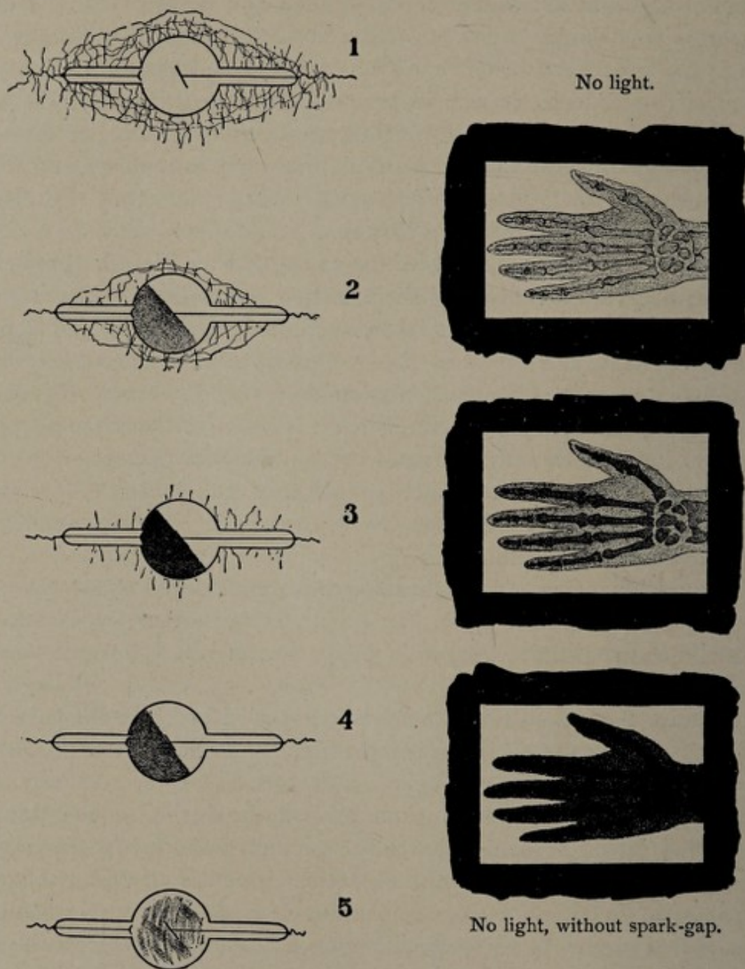
FIG. 39. Diagram showing the effect of the resistance of the tube on the X-ray picture thrown on the screen and the advantage of the multiple spark-gap. The direction of the light is downwards and to the left.
