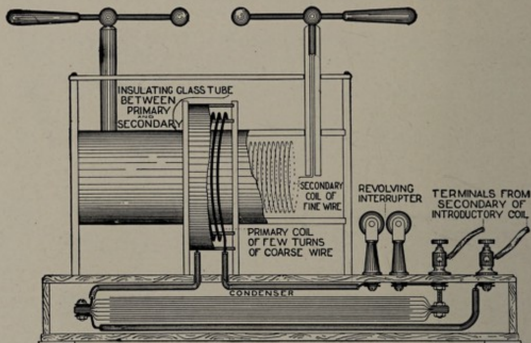
FIG. 20. Diagram of high frequency coil. (Rollins.)
