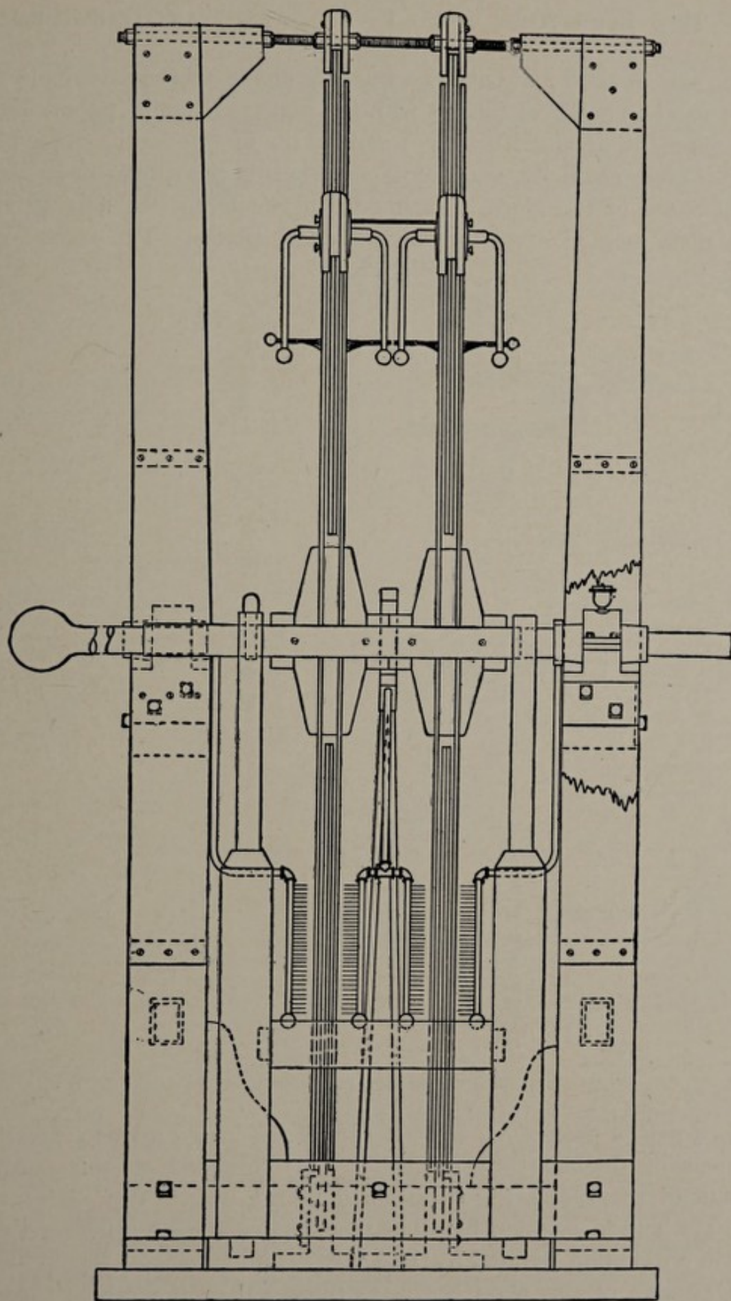
FIG. 4. End view of static machine. Cut also shows some details of shaft and attachment of plates.
