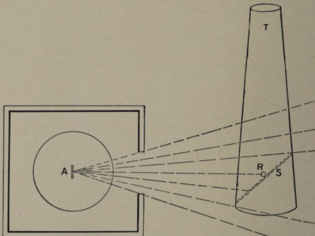
FIG. 410. Fluorometer. Instrument for determining the amount of fluorescence produced by different vacuum tubes on the tungstate of calcium screen, and also for determining the quality of different tungstate of calcium screens. The cut shows the section of a Rollins box, and of a vacuum tube, the anode of which is at A . The broken lines originating at A represent the cone of rays issuing from the box. At the right of the cut is shown a cardboard tube T the interior of which is black and in the lower end of which is a small oval screen S of tungstate of calcium; across this screen is fastened a sealed glass tube R eight centimetres long, containing some radium (Currie). This screen has been put at an angle in the tube in order that the instrument may be used without exposing the eye and the hand to the X-rays. To determine the amount of fluorescence produced on the tungstate of calcium screen by a given tube the room should be darkened; the tube T should be grasped near the top, and its opening, the rim of which is made soft by a covering of velvet, placed close to the eye; the tube T should be held at such a distance from the anode of the vacuum tube that the radium appears as a bright band on the less bright screen; then the cardboard tube should be brought gradually nearer the anode until a point is reached at which the amount of light from the radium R and the screen S is about equal (or the point when the band of light from the radium is just disappearing may be chosen). The distance between the radium and the anode should then be measured and noted. Vacuum tubes may thus be tested and the differences between them determined. By using a tube, the brilliancy of which has been thus determined, tungstate of calcium screens can also be thus tested and their different degrees of brightness measured. The brightness of the radium can be measured in terms of a known standard by a photometer, and then by means of a fluorometer the tube and the screen can be referred to the same standard.
