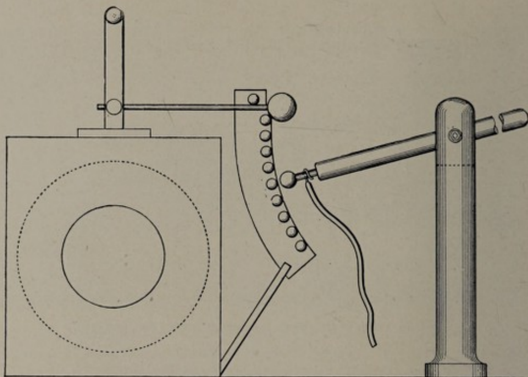
FIG. 18. Adjustable multiple spark-gap for coil.
