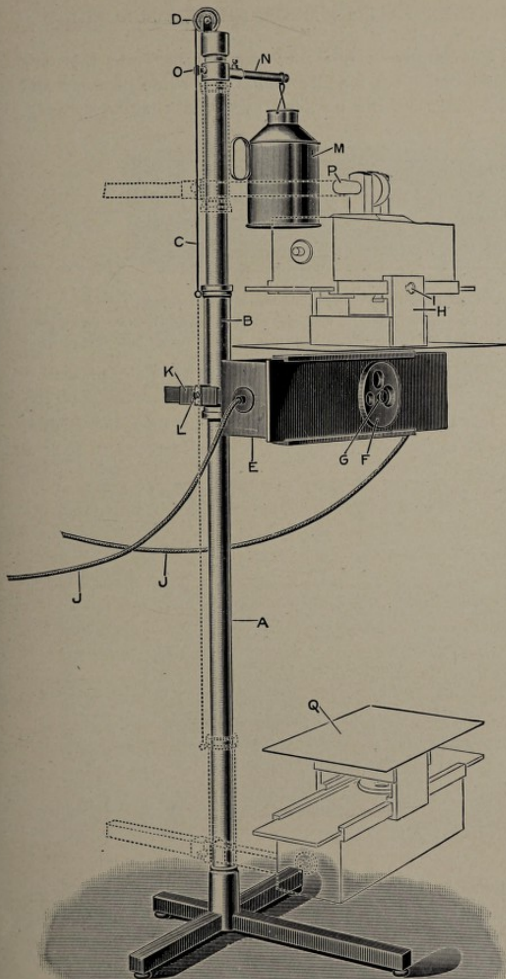
FIG. 41. Tube holder. A , brass tube 7 feet high. B , sleeve with ball bearings sliding on tube A , and supporting a box E containing the tube. The front of this box can be removed by sliding it sideways in the grooves shown. This movement also allows any opening of the diaphragm plate F to be brought opposite the radiant area of the target of the tube. G is a screw which acts as a pivot and clamp for diaphragm plate. The distance of the tube box from the upright A can be changed by sliding the bar to which it is attached by the pivot and clamp screw P in the metal sleeve K . L is a clamping screw. H , sliding holder for Tesla screen. I , clamp. Q , screen. C , cord attached to sleeve B . It passes over a pulley D . To the other end is attached a lead weight sliding inside the tube A , and serving to balance the tube box E , which therefore remains in any position without fastening it. M , water-can for cooling the water for hollow target tube. N , insulating supporting rod. O , clamp to collar which allows the height of can to be changed. The tube holder moves in altitude about the axis of the clamping screw P . It can be brought above or below the patient, as shown in the outlines. J , terminals from generator, insulated from tube box by heavy rubber disks. (Rollins.)
