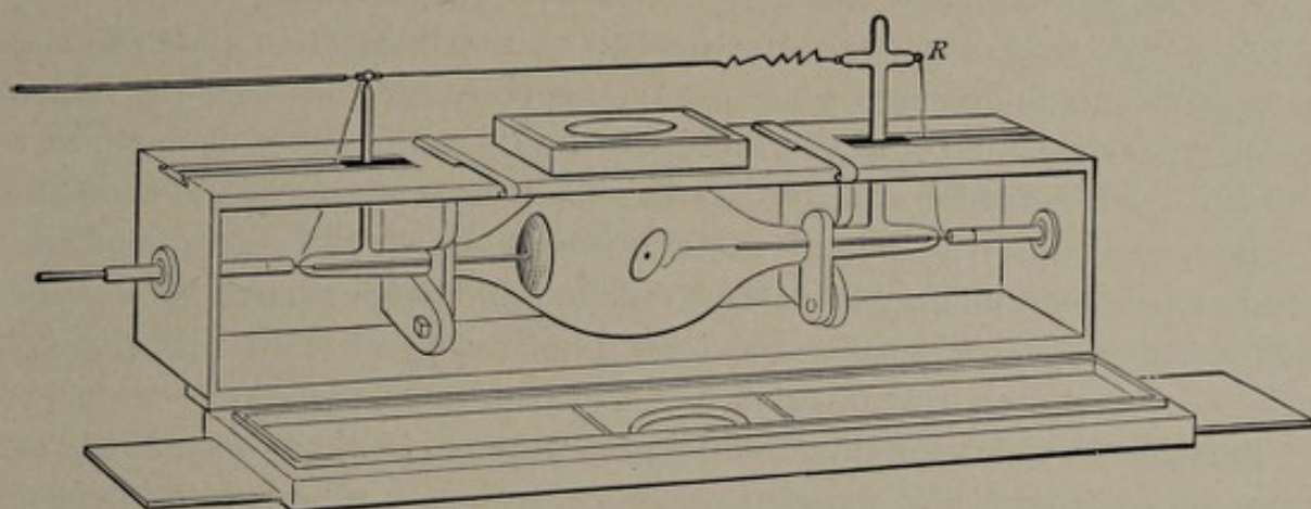
FIG. 38. A. W. L. X-light tube with a rotary, sliding target and an automatic regulator (Rollins).
