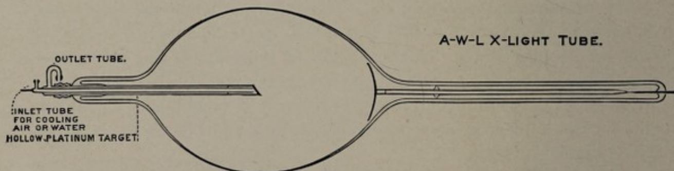
FIG. 27. Section of cooled target tube. (Rollins.)
