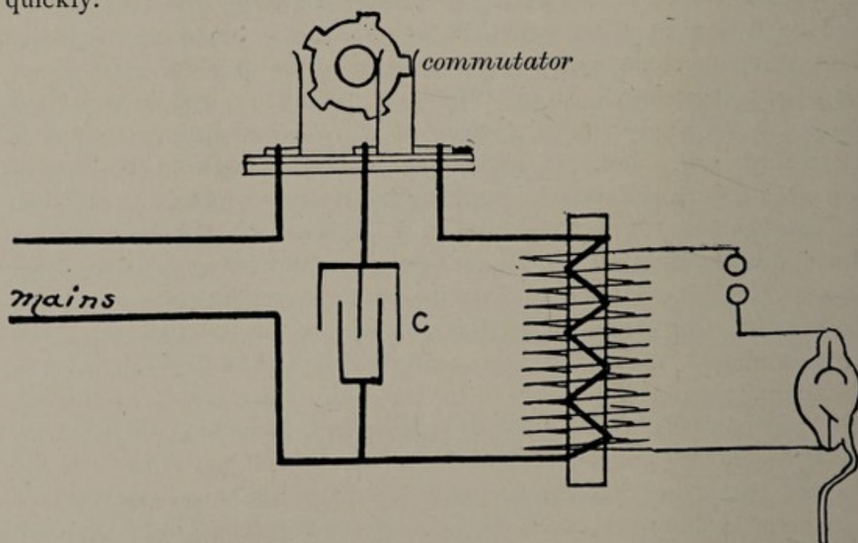
FIG. 391. Norton and Lawrence apparatus. This cut is taken from the Electrical Engineer , March 24, 1897. The direct current of 220 volts is taken from the street main; by means of the commutator the condensers ( C ) are charged with this current and then discharged through the primary of the coil.
