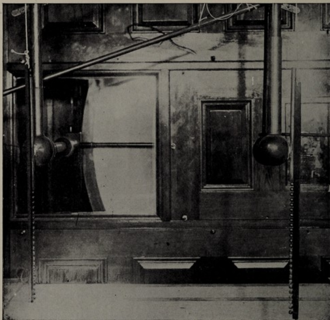
FIG. 8. Adjustable multiple spark-gap.
