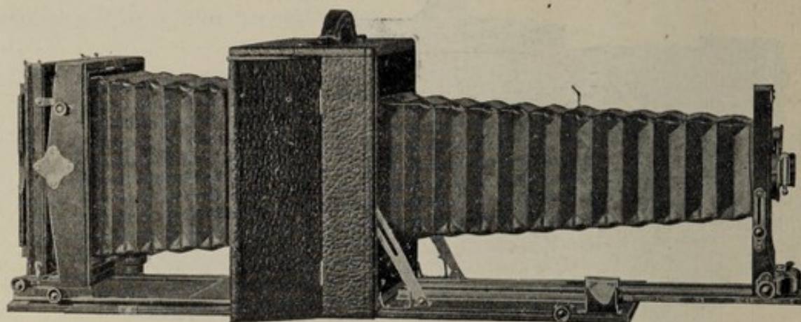
Fig. 58. 5 x 7 "Korona" Royal camera.
