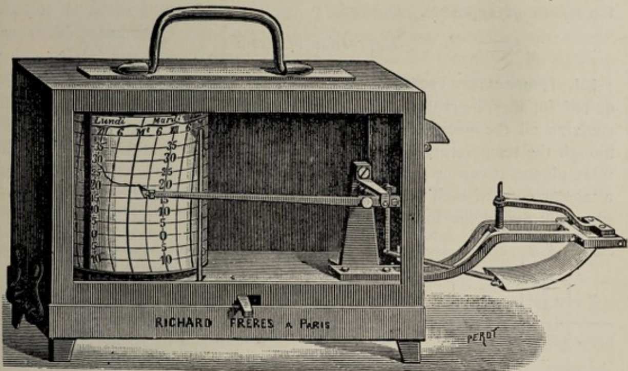
Fig. 21. Richard thermograph.
