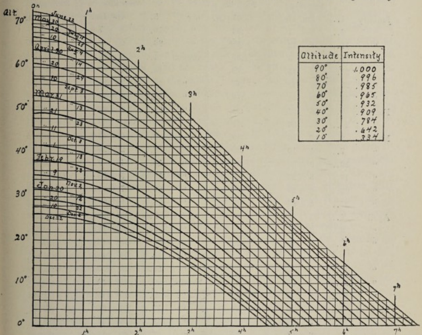
Fig. 13. Chart for the determination of the sun's altitude, and the corresponding light intensity.
