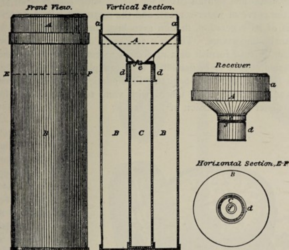
Fig. 22. Rain gauge showing construction.
