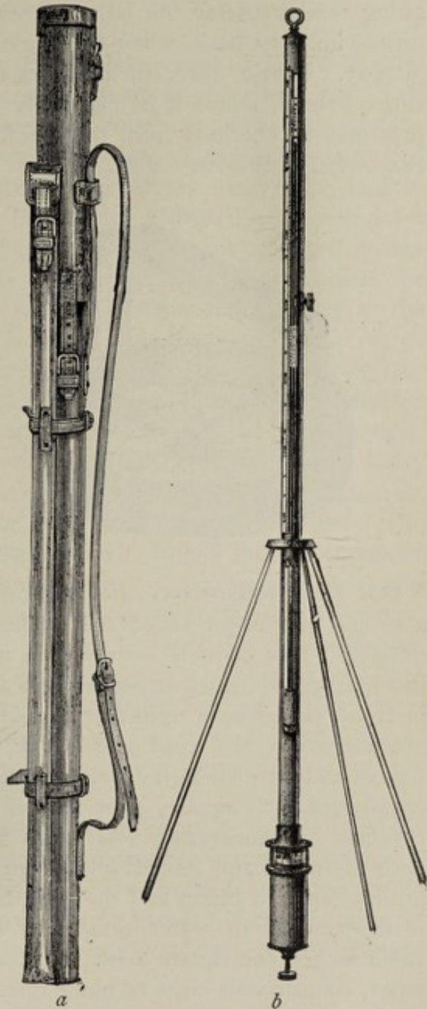
Fig. 27. Mountain barometer: (a) in carrying case; (b) set up for use.
