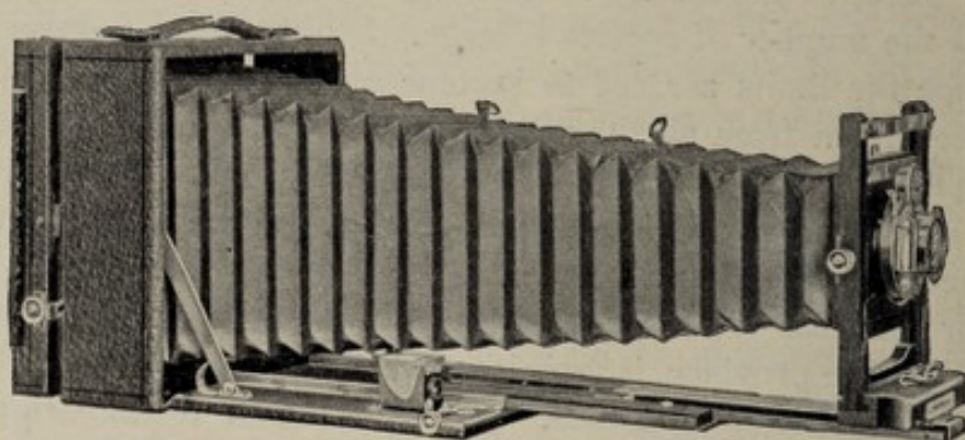
Fig. 56. 4 x 5 long focus "Korona" camera (series V).
