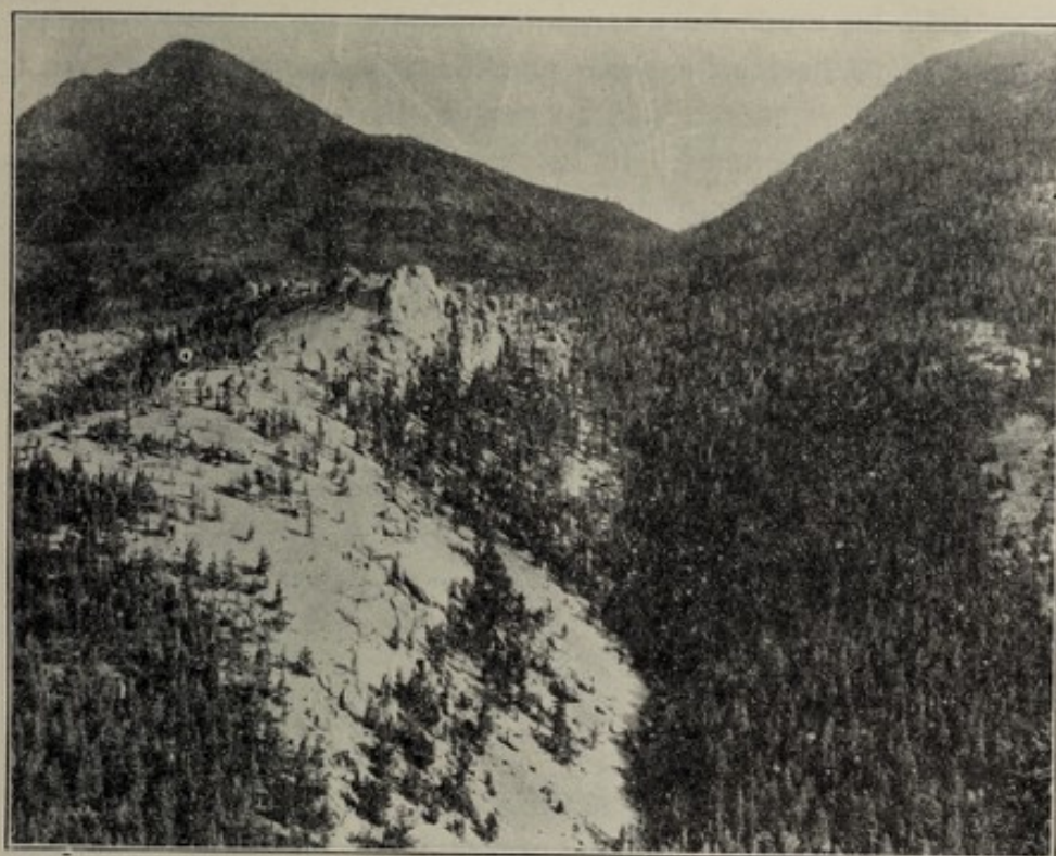
Fig. 70. Alternating gravel slides on Mounts Cameron and Palsgrove, from the comparison of which the initial development of the talus succession has been reconstructed.
