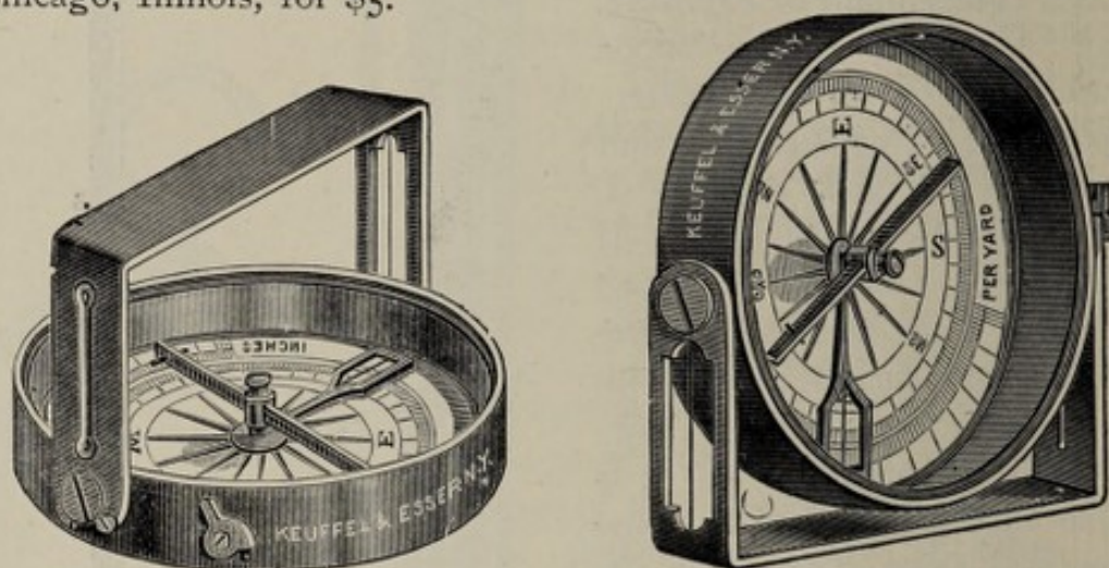
Fig. 28. Combined clinometer and compass.
