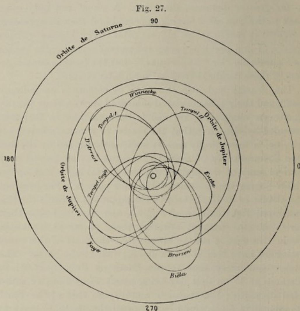
DIAGRAM ILLUSTRATING THE INFLUENCE OF JUPITER ON COMETS.
