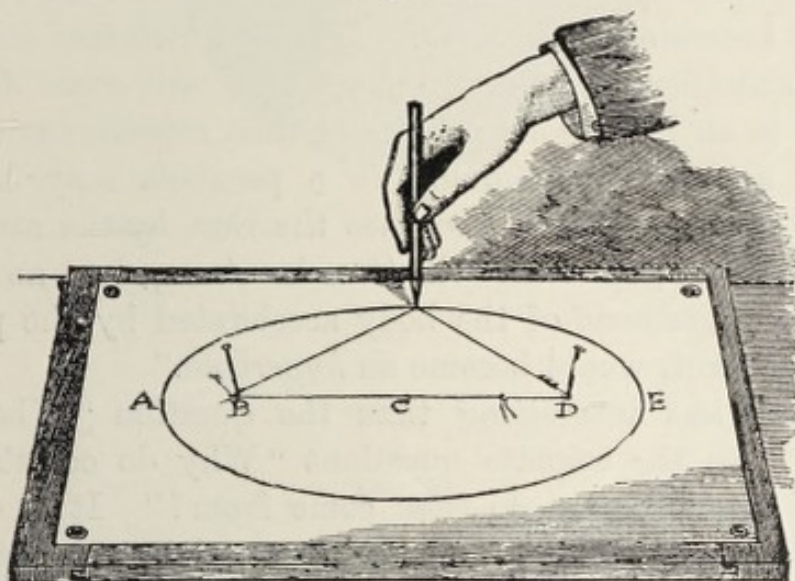
THE CONSTRUCTION OF AN ELLIPSE.
