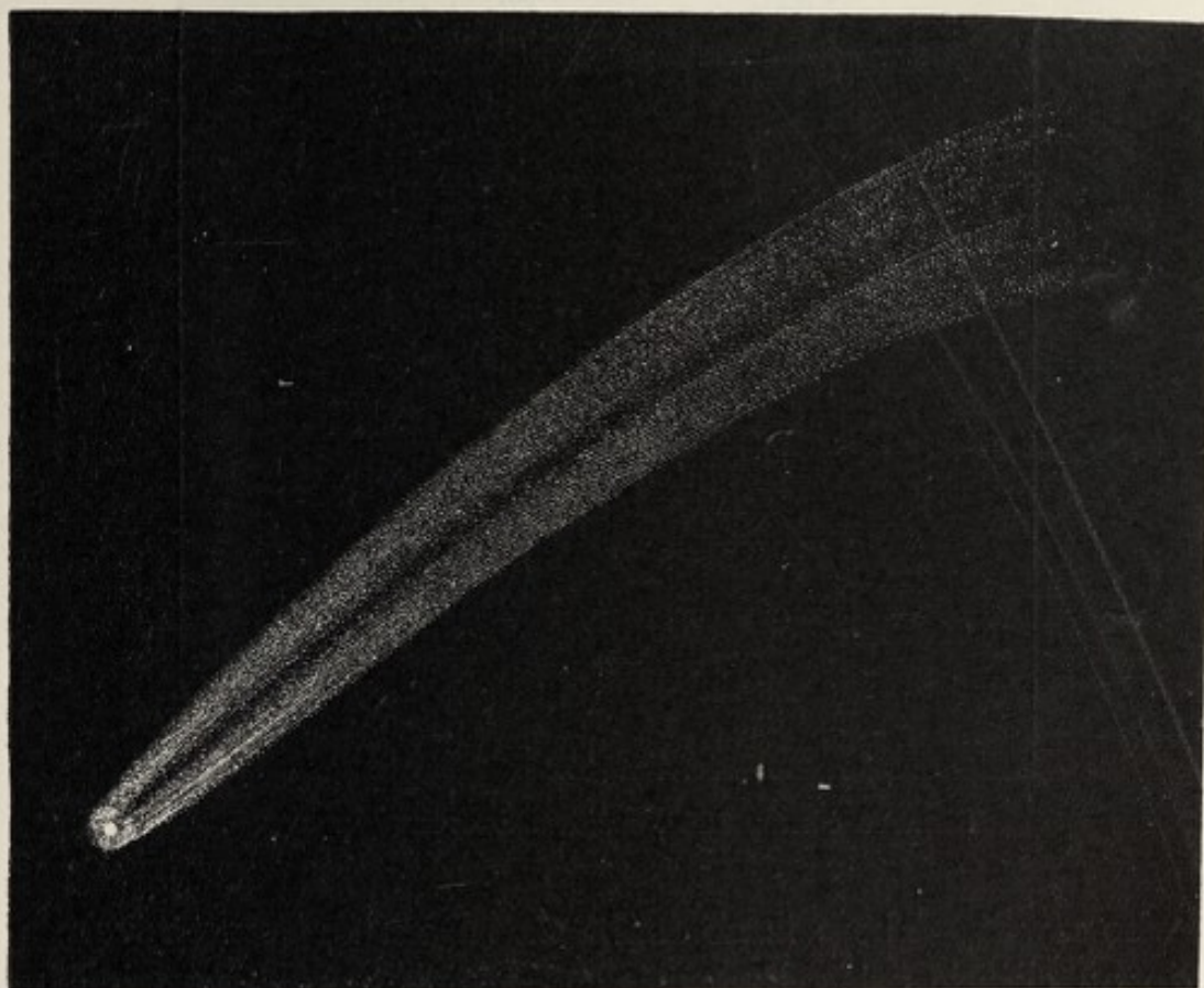
DONATI'S COMET, 1858, SEPT. 30. ( Smyth. )
