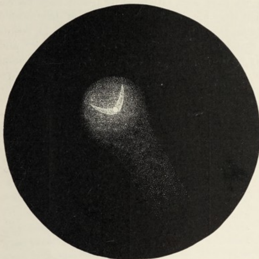
HALLEY'S COMET, 1835, OCT. 11. ( Smyth. )
