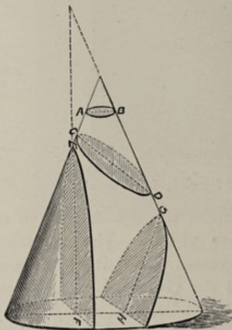
THE VARIOUS SECTIONS OF A CONE.
