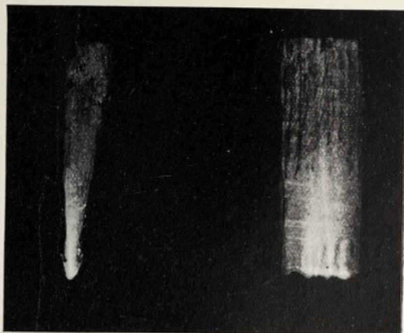
PHOTOGRAPH AND SPECTROGRAPH OF MOREHOUSE'S COMET (1908, iii.).
