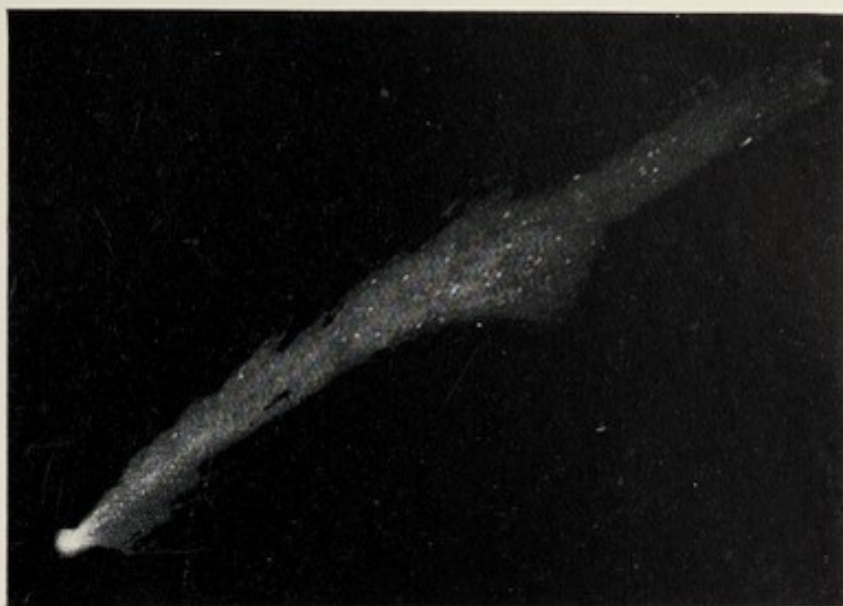
MOREHOUSE'S COMET (1908, iii.). December 11.
