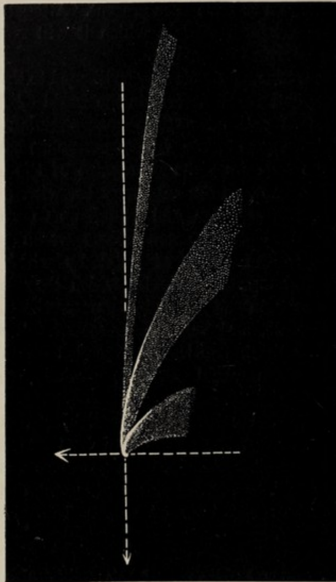
BREDICHIN'S THREE TYPES OF COMET TAILS.
