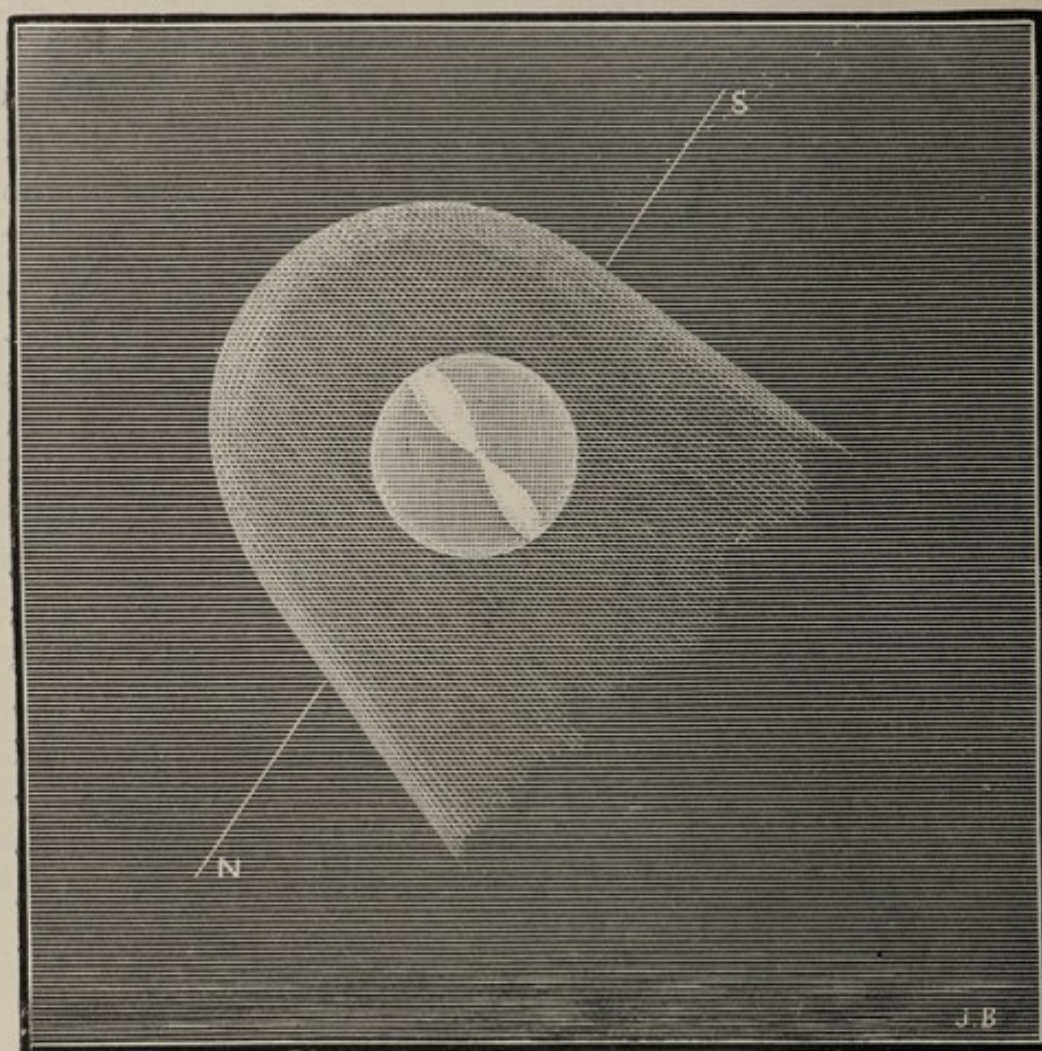
PONS'S COMET : JAN. 19, 1884. ( Trépied. )
