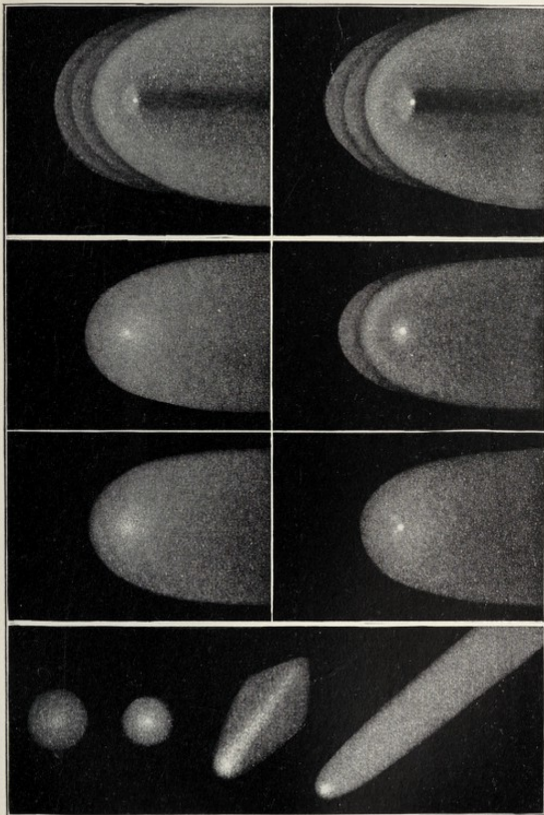
COGGIA'S COMET OF 1874 (iv.).
