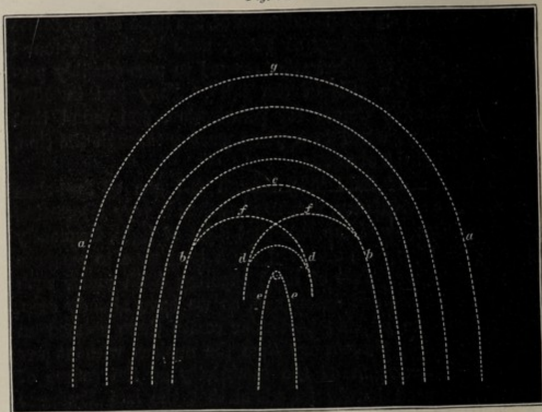
COGGIA'S COMET OF 1874.
