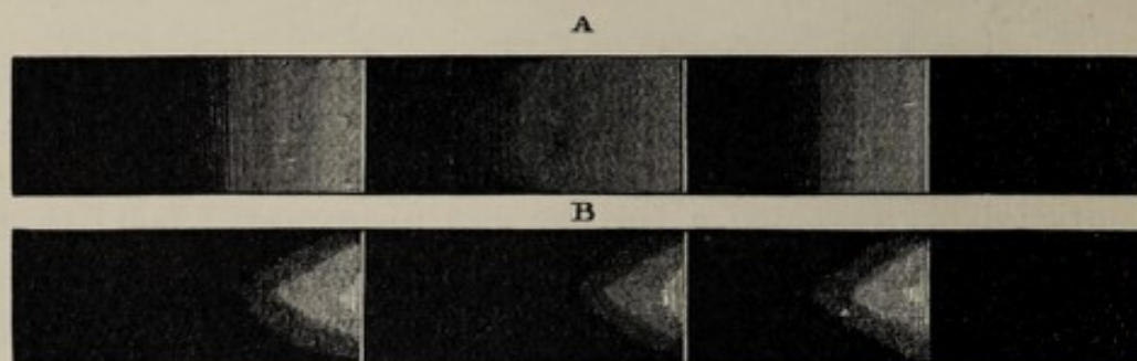
SPECTRA OF OLEFIANT GAS AND WINNECKE'S COMET, 1868.
