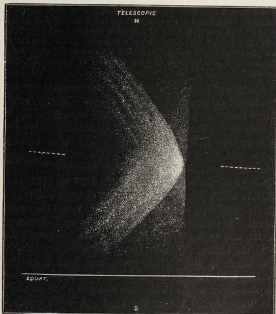
ENCKE'S COMET: NOV. 9, 1871. ( J. Carpenter. )
