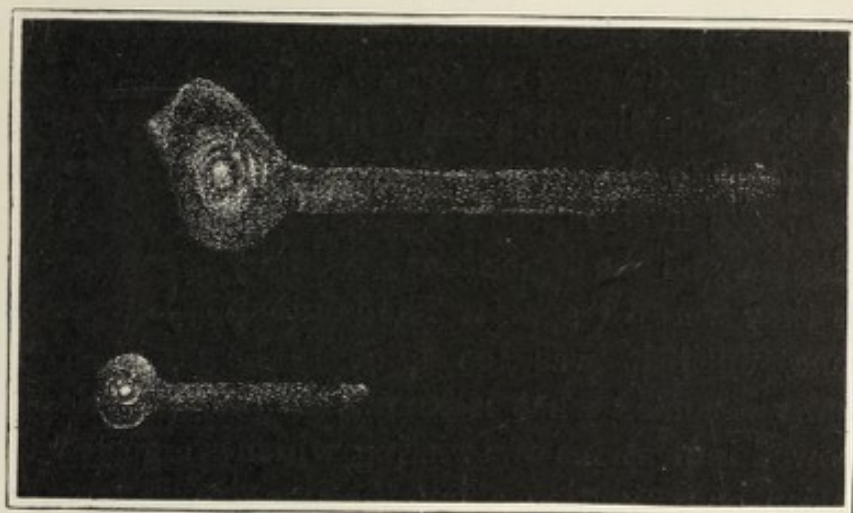
BIELA'S COMET, FEB. 19, 1846. ( O. Struve. )
