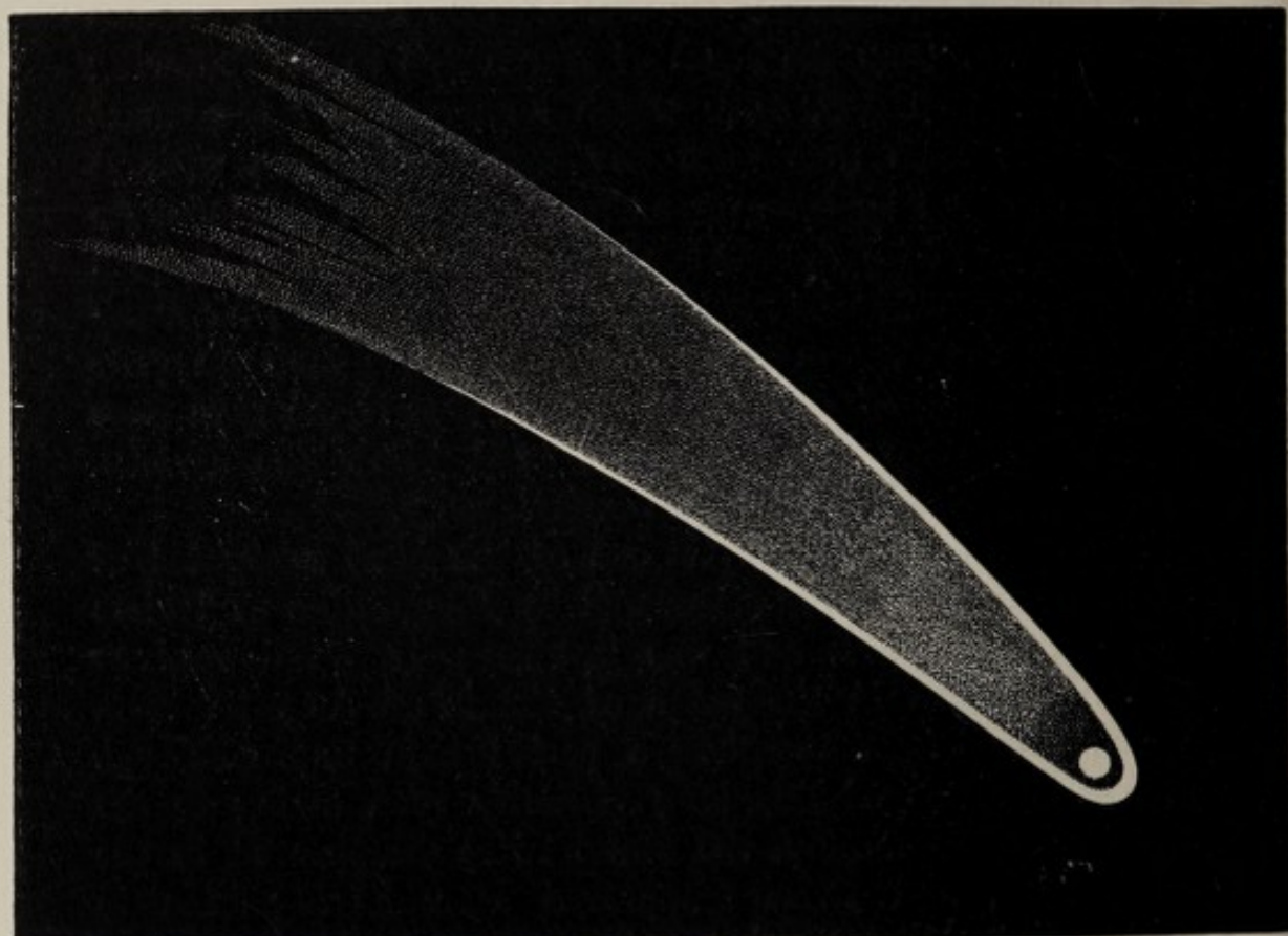
THE GREAT COMET OF 1811.
