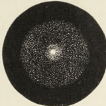
TELESCOPIC COMET WITH A NUCLEUS.
