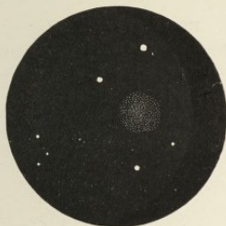
DISCOVERY FIELD OF BROOKS'S COMET OF 1895 (iii.).
