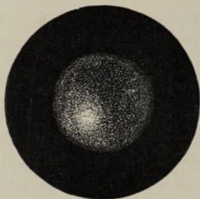
ENCKE'S COMET: NOV. 30, 1828. ( W. Struve. )
