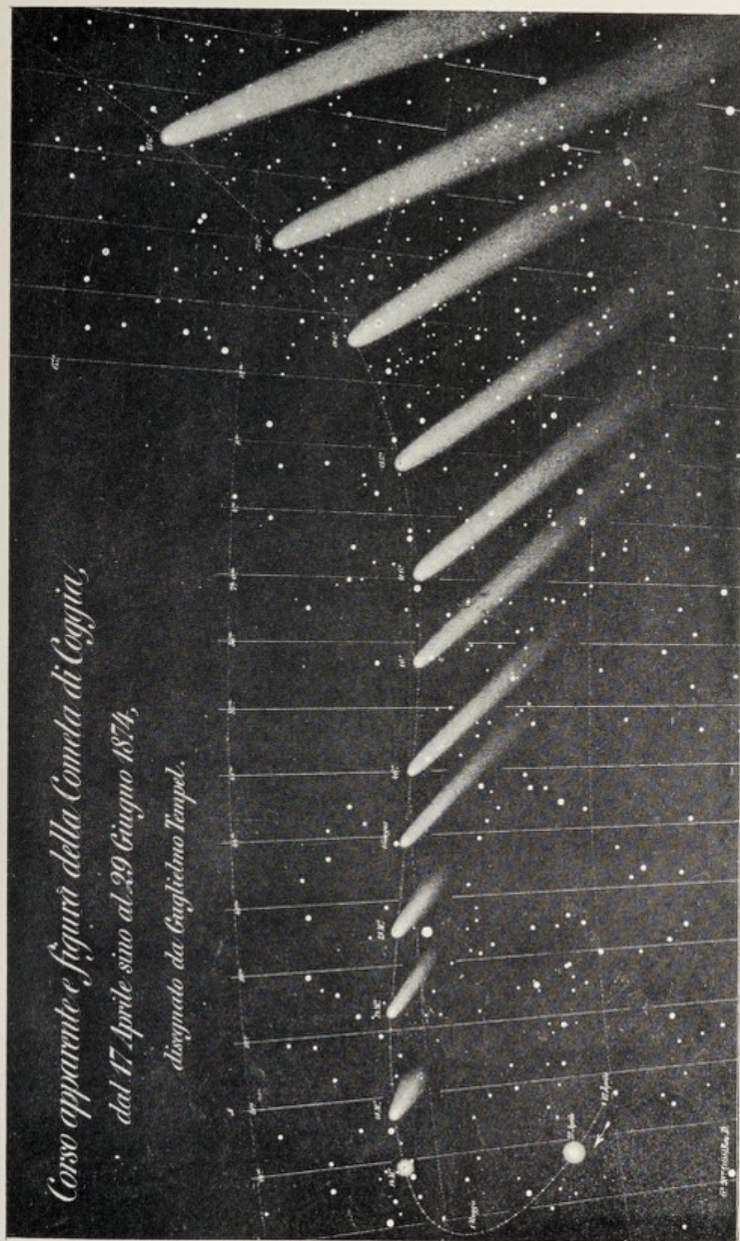
COGGIA'S COMET OF 1874 (iv.).
