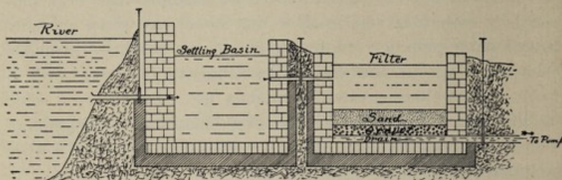
Fig. 151.—Cross-section of filter plant (after Hazen).
