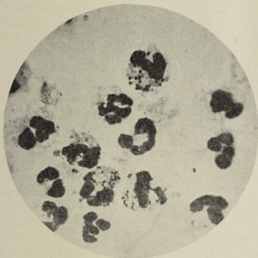
Fig. 42.—Meningococci in pus from brain abscess (Flexner).
