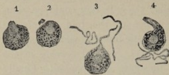
Fig. 133.—Fertilization, tertian parasite: 1, Extrusion of nuclear substance by macrogamete; 2, macrogamete with divided nucleus; 3, entrance of microgamete into the macrogamete; 4, zygote (Schaudinn).
