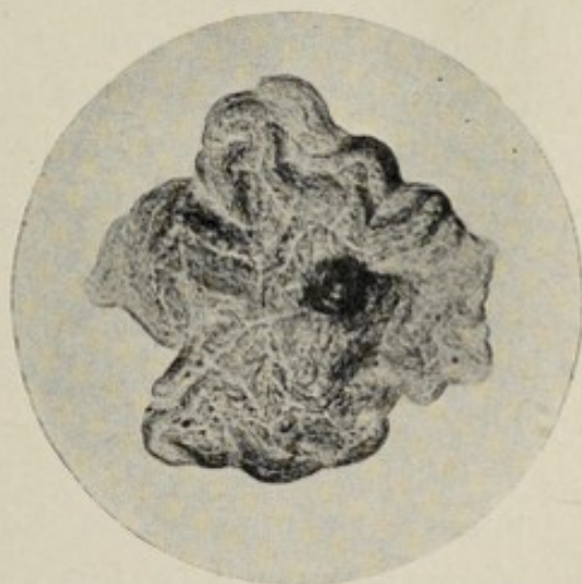
Fig. 62.— Bacillus typhosus colony on gelatin, seventy-two hours old; unstained; Neufeld prep. (Kolle and Wassermann).
