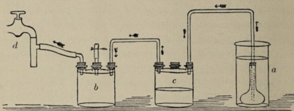
Fig. 9.—Apparatus for the rapid filtration of toxins, etc.: a , Filter flask; b , Woulfe bottle to guard against regurgitation of water from the pump; c , reservoir for the filtrate; d , water vacuum pump (McFarland).
