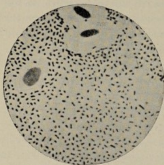
Fig. 77.—Bacillus of hemorrhagic septicemia in blood of a bird. Fuchsin stain (Kitt prep.) (Kolle and Wassermann).
