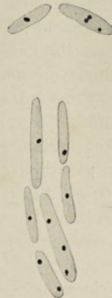
Fig. 15.—Chromatin granules in Bacillus megatherium (after Zettnow).
