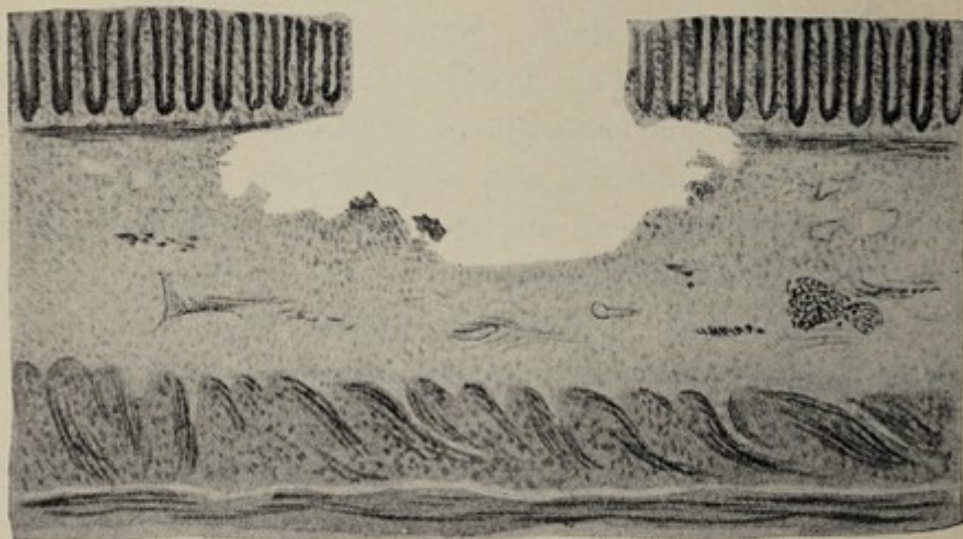
Fig. 126.—Section of an intestinal ulcer (Kartulis, in Kolle and Wassermann).
