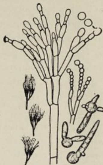
Fig. 144.— Penicillium of Camembert cheese, showing method of forming spores (Thom).
