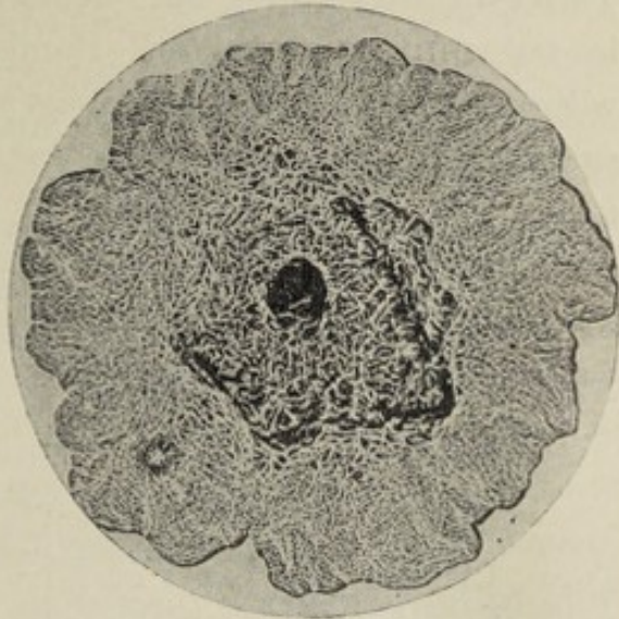
Fig. 75.— Bacillus dysenteriae . Colony on gelatin, four days; \times 20 (Doerr).
