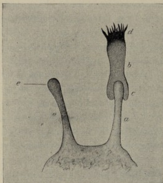
Fig. 22.—Graphic representation of receptors of the first order and of toxin uniting with the cell-receptor: a , Cell-receptor; b , toxin molecule; c , haptophore of toxin molecule; d , toxophore of toxin molecule; e , haptophore of the cell-receptor (Ehrlich).
