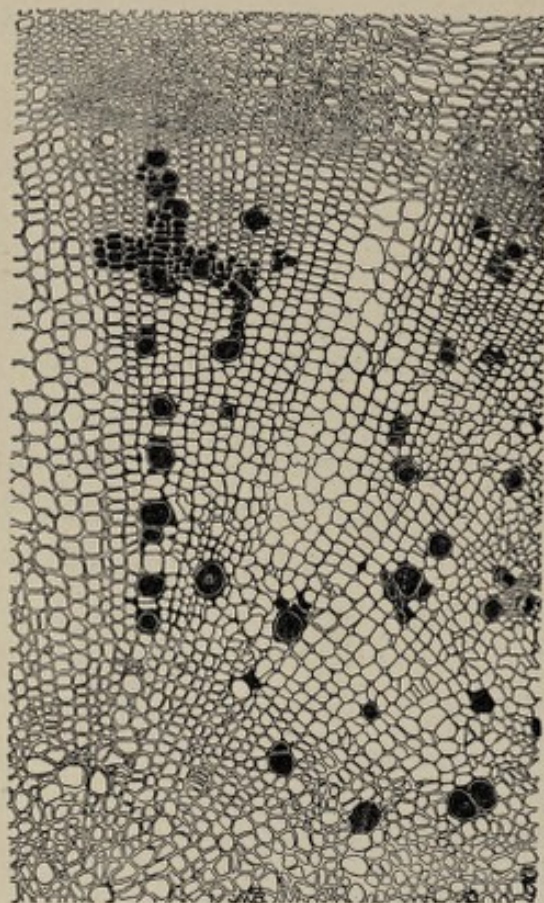
Fig. 154.—Cross-section of a turnip root, showing vessels occupied by Bacillus campestris as the result of a pure culture inoculation by means of needle pricks on the leaves. The bacteria are confined to the vessels and their immediate vicinity. They do not occur in the phloem, a small portion of which is shown at the top of the picture. Drawn from a micro-photograph. \times 57 (Erwin Smith).
