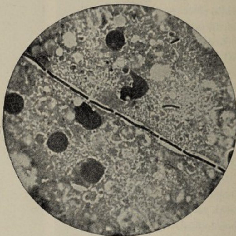
Fig. 90.— Bacillus welchii , smear preparation from rabbit's liver; \times 1000 (Williams).
