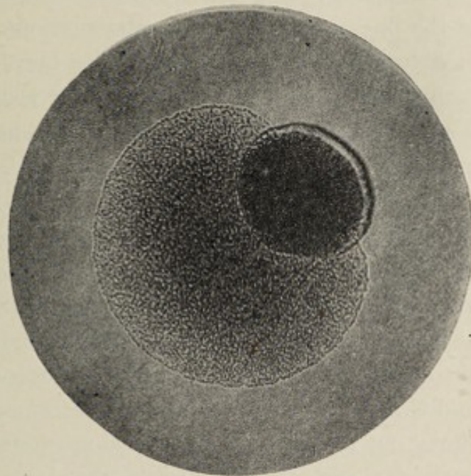
Fig. 40.— Streptococcus pneumoniae ; colony in agar twenty-four hours old; \times 100 (Fränkel and Pfeiffer).
