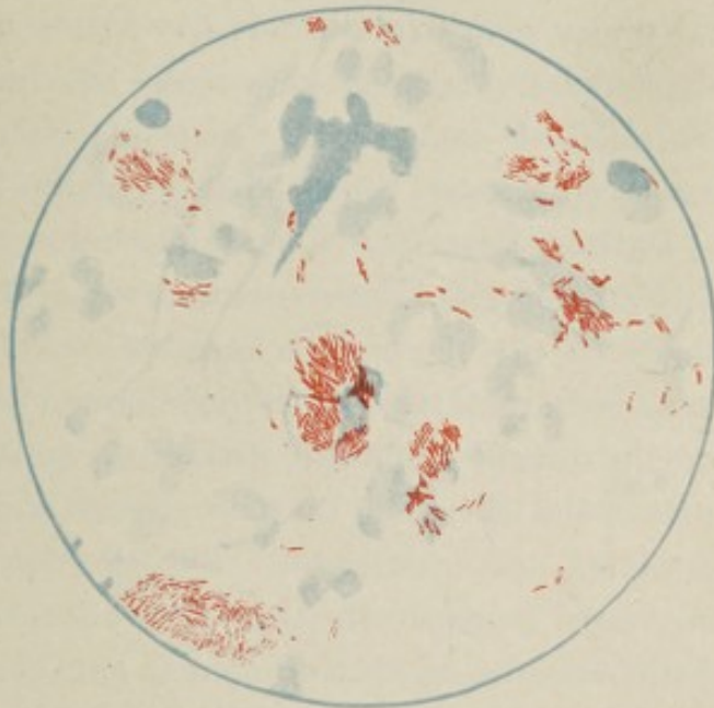
Fig. 96.— Bacillus lepræ . Smear preparation from nasal mucosa (Hansen, Kolle and Wassermann).
