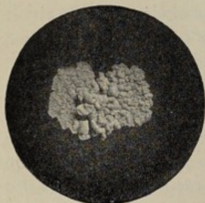
Fig. 95.— Bacillus tuberculosis , source human. Mature colony on glycerin agar. Actual size (Swithinbank and Newman).
