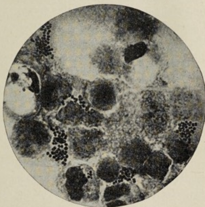
Fig. 31.— Staphylococcus aureus in pus from human abscess. Fuchsin stain; \times 1000 (Fränkel and Pfeiffer).
