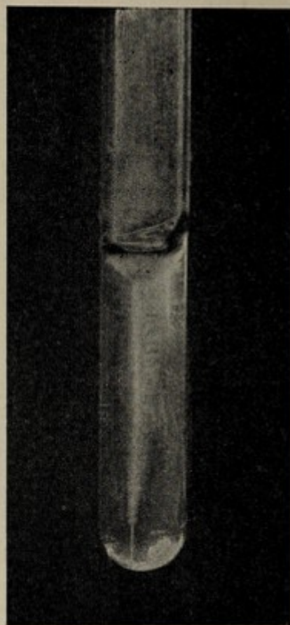
Fig. 51.— Bacillus anthracis , gelatin stab-culture (Crookshank).
