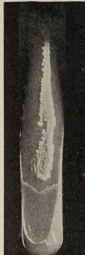
Fig. 59.—True diphtheria bacillus. Natural size. From photograph taken by Dr. Henry Koplik, Carnegie Laboratory, New York.
