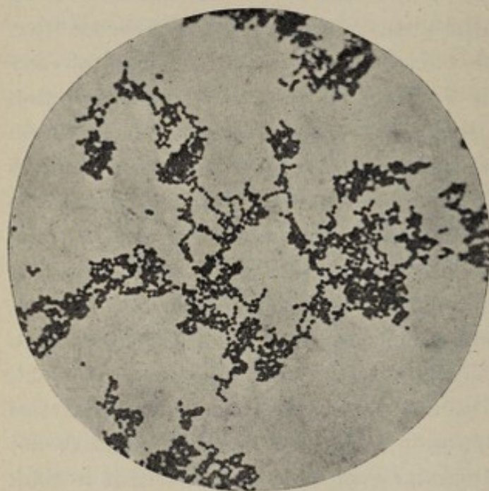
Fig. 37.—Streptococcus agglutinated by immune horse serum (Moser and v. Pirquet).
