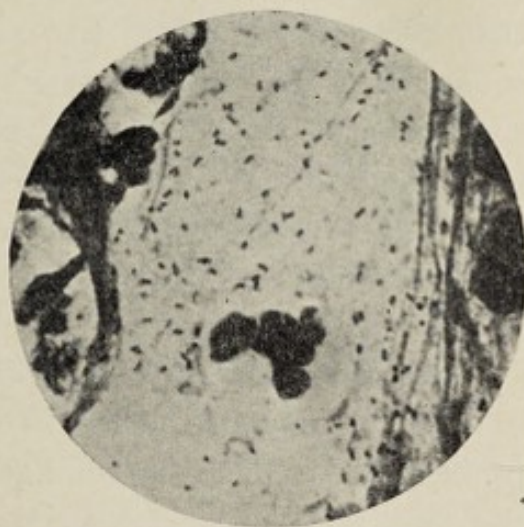
Fig. 83.— Bacillus influenzae in sputum. Fuchsin stain. Beck prep. (Kolle and Wassermann).
