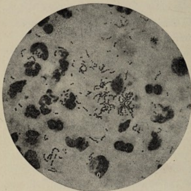
Fig. 36.— Streptococcus pyogenes in pus from a human abscess; gentian-violet (Fränkel and Pfeiffer).
