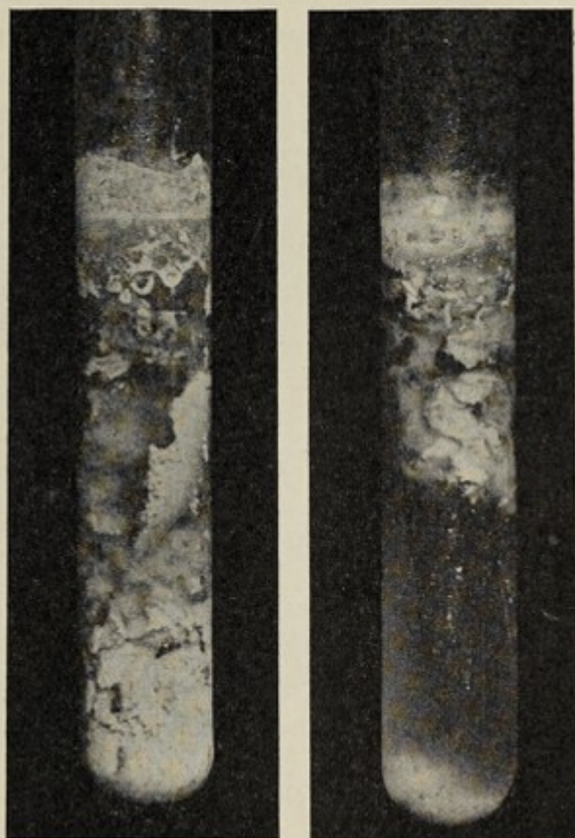
Fig. 89.—Typical reactions of bacillus welchii in milk, forty-eight hours old.
