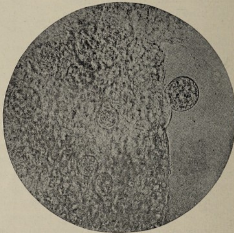
Fig. 134.—Malarial zygotes in stomach wall of the mosquito. High power (Manson).
