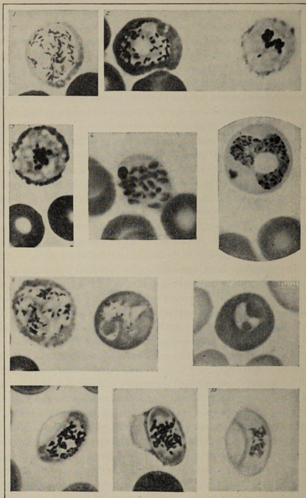
Fig. 131.—Malarial parasites: 1 to 5, Various stages in the life-cycle of the tertian parasite; 6, on the left, an adult tertian parasite in a red blood-corpuscle; on the right, a young tertian parasite and a hyaline form of the estivo-autumnal parasite in a red blood-corpuscle; 7, hyaline form of the estivo-autumnal parasite in a corpuscle; 8, 9, 10, crescentic and ovoid forms of the estivo-autumnal parasite in red blood-corpuscles (Wright and Brown).
