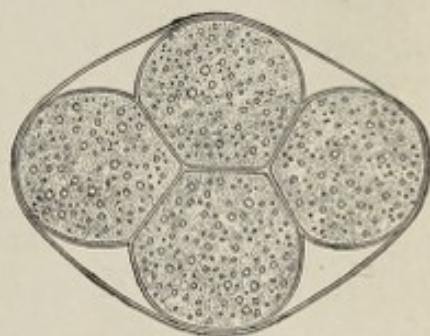
Fig. 119.—Spores of yeast (ascospores). Four spores in a cell of brewer's yeast ( Saccharomyces cerevisiæ ) (Sedgwick and Wilson).
