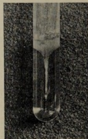
Fig. 30.— Staphylococcus pyogenes aureus , gelatin stab-culture; four days.
