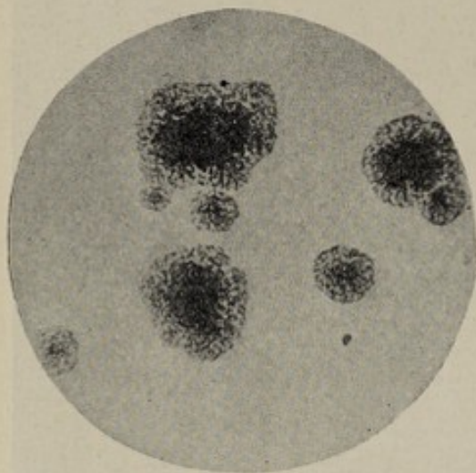
Fig. 60. — Bacillus diphtheriae colonies on glycerin-agar, twenty-two hours old; \times 39 (Heim).
