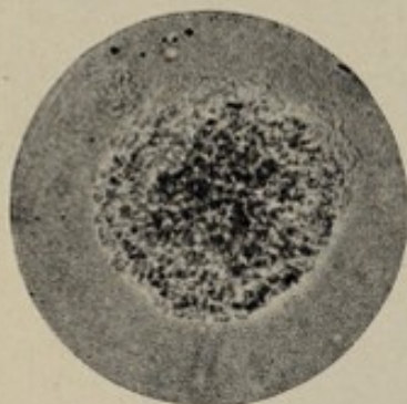
Fig. 80.—Colony of bacillus pestis. Gelatin, forty-eight hours; \times 150 (Wilson).
