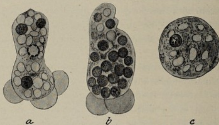
Fig. 128.— Entameba histolytica (Kruse and Pasquale): a and b , Amebæ as seen in the fresh stools, showing blunt ameboid processes of ectoplasm. The endoplasm of a shows a nucleus, three red corpuscles, and numerous vacuoles; that of b , numerous red corpuscles and a few vacuoles; c , an ameba as seen in a fixed film preparation, showing a small rounded nucleus; \times 600 .
