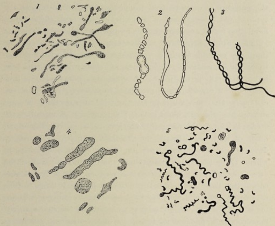
Fig. 14.—Involution forms of bacteria (enlarged about 1000): 1, Bacillus proteus mirabilis (Hauser); 2, Bac. aceticus (Hauser); 3, spirilla form of Bacillus anthracis (Petruschky); 4, involution forms of Bac. halophilus (Russell); 5, Spirillum cholerae (van Ermengem).
