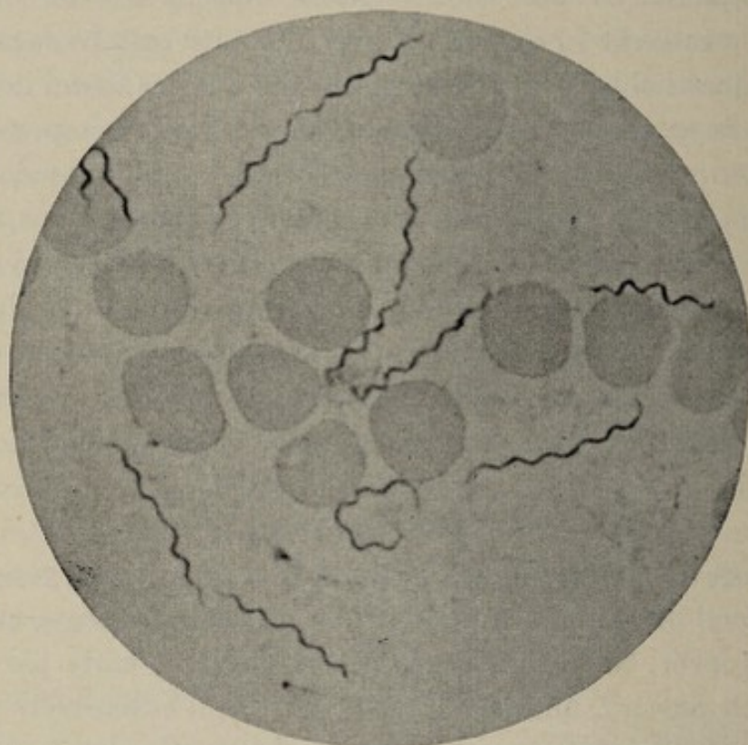
Fig. 107.— Spirillum obermeieri in blood of rat, showing divisional forms. A group showing spirilla of different lengths. The two long ones above show transverse division; \times 1500 (Novy and Knapp).
