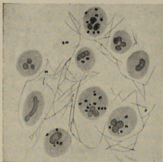
Fig. 41.—Meningococcus in pus cells (Councilman): Pus cells containing diplococci from the meninges. A few diplococci are in the exudate outside of the pus cells. Between the pus cells there are delicate fibrillae of fibrin. The illustration is an accurate representation of a group of cells in the field of the microscope.
