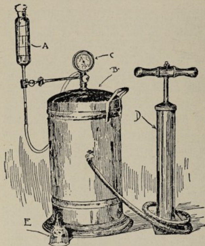
Fig. 150.—Apparatus for the quantitative determination of micro-organisms in air: A, Aërobioscope; B, air-cylinder; C, vacuum gauge; D, air-pump; E, glass shield (Tucker).
