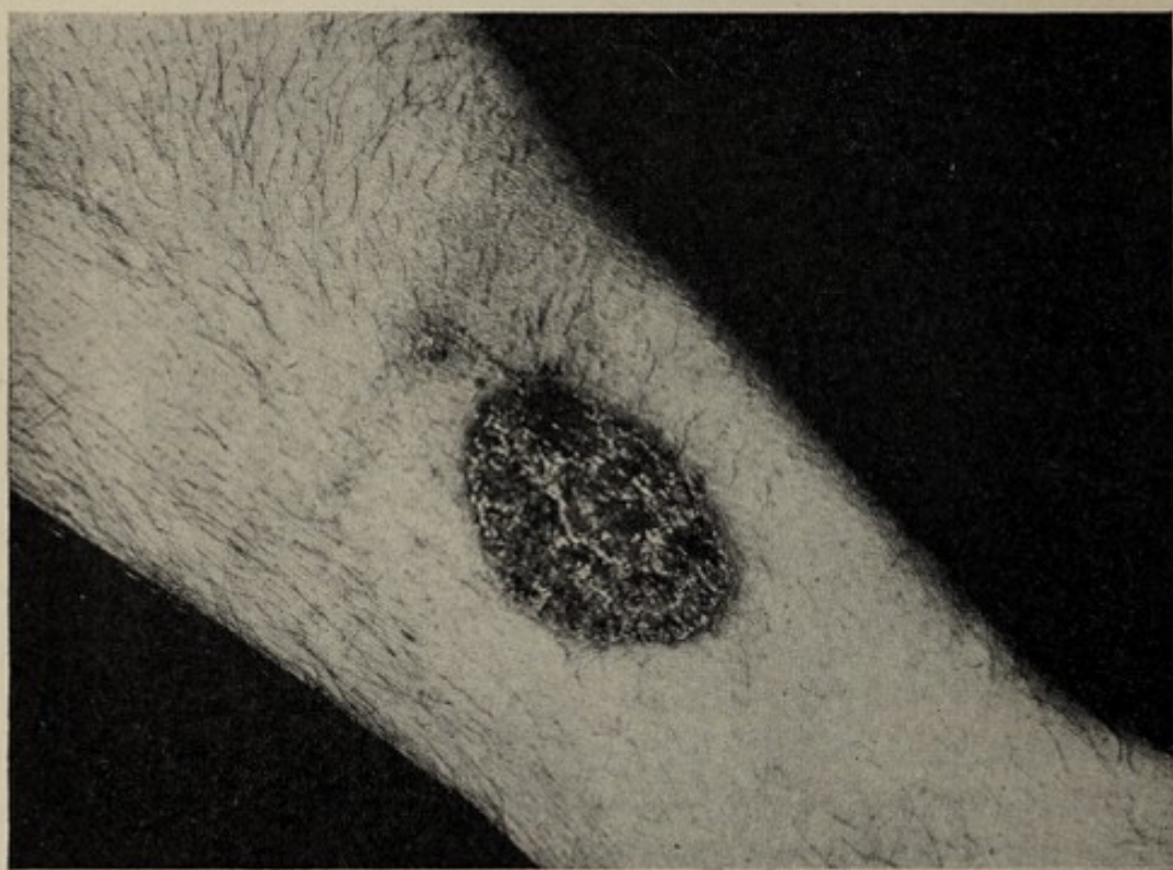
Fig. 121.—Blastomycosis. Old partially healed ulcer of the leg (Irons and Graham).
