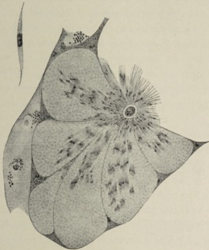
Fig. 135.—Section of salivary gland of a mosquito, Anopheles . Sporozoites (Grassi).
