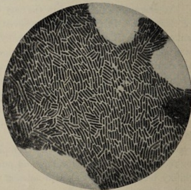
Fig. 69.— Bacillus typhosus . Colony on gelatin smear preparation stained with fuchsin; \times 1000 (Fränkel and Pfeiffer).
