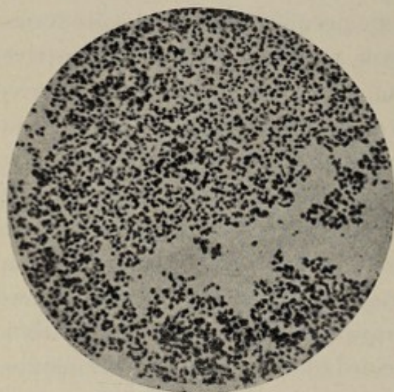
Fig. 149.—Nitrate-former from St. Petersburg nitrate. Agar. Fuchsin. \times 1000 (Lafar).
