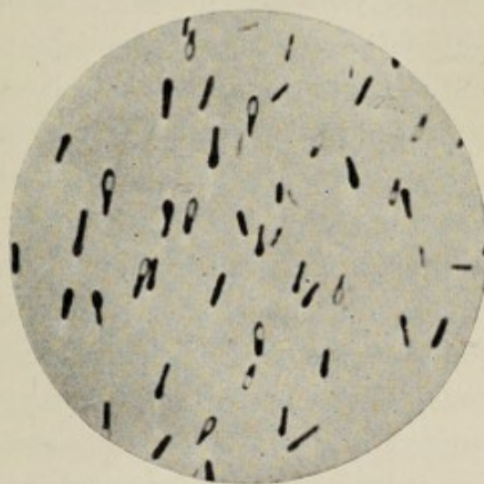
Fig. 17.—Spores, bacillus of symptomatic anthrax. Methylene - blue stain (Kolle and Wassermann).
