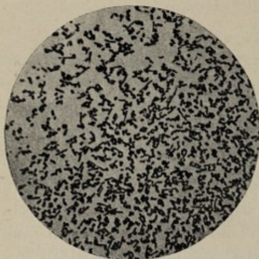
Fig. 63.— Bacillus coli ; twenty-four-hour agar culture; \times 650 (Heim).
