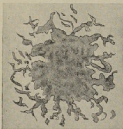
Fig. 100.— Bacillus proteus colony (Lehmann and Neumann).
