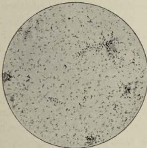
Fig. 26.—Typhoid bacilli partially agglutinated.
