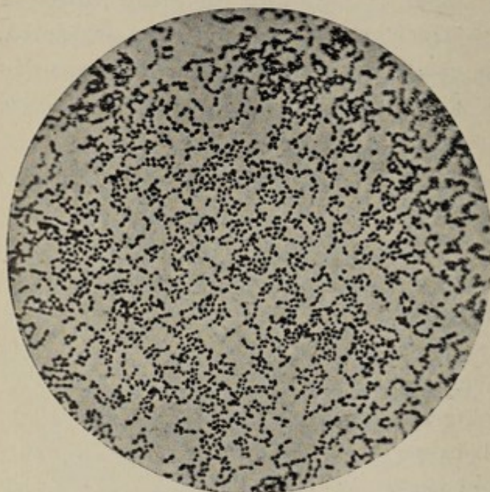
Fig. 33.—Streptococcus, pure culture (Moser and v. Pirquet).
