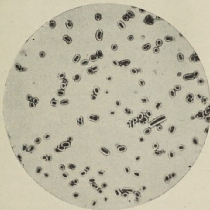
Fig. 79.— Bacillus pestis from agar culture, twenty-four hours, showing capsule; \times 700 (Wherry).
