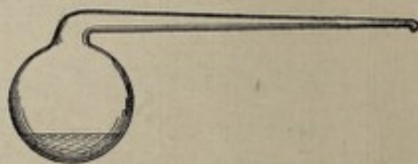
Fig. 8.—Sternberg's bulb for testing thermal death-point.
