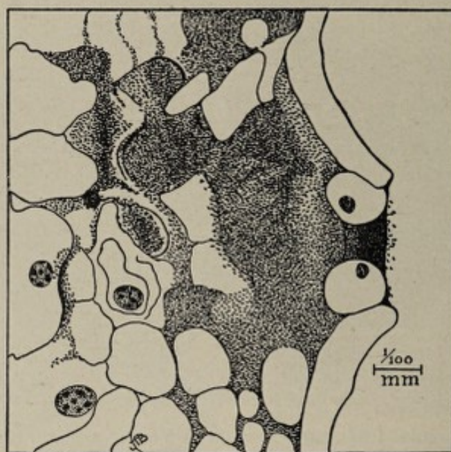
Fig. 156.— Bacterium stewarti filling the substomatic chamber and pushing out into the deeper tissues of a maize leaf. The result of an inoculation made by placing a small quantity of a pure culture on the tip of a sweet-corn leaf in the seedling stage. The globose bodies are nuclei (Erwin Smith).
