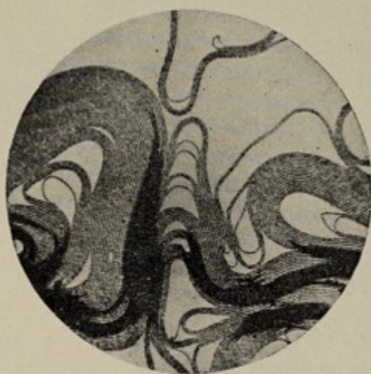
Fig. 50.— Bacillus anthracis , impression preparation, edge of colony; Zettnow prep. (Kolle and Wassermann).
