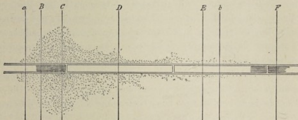
Fig. 20.—Bacteria gathered around alga, evolving oxygen (from Engelmann). Piece of cladophora with swarming bacteria in the microspectrum (gaslight). The chlorophyll grains which fill the cells very uniformly are omitted, and, instead, the absorption band between B and C and the tolerably pronounced band at the violet end between E and F , are indicated by shading.
