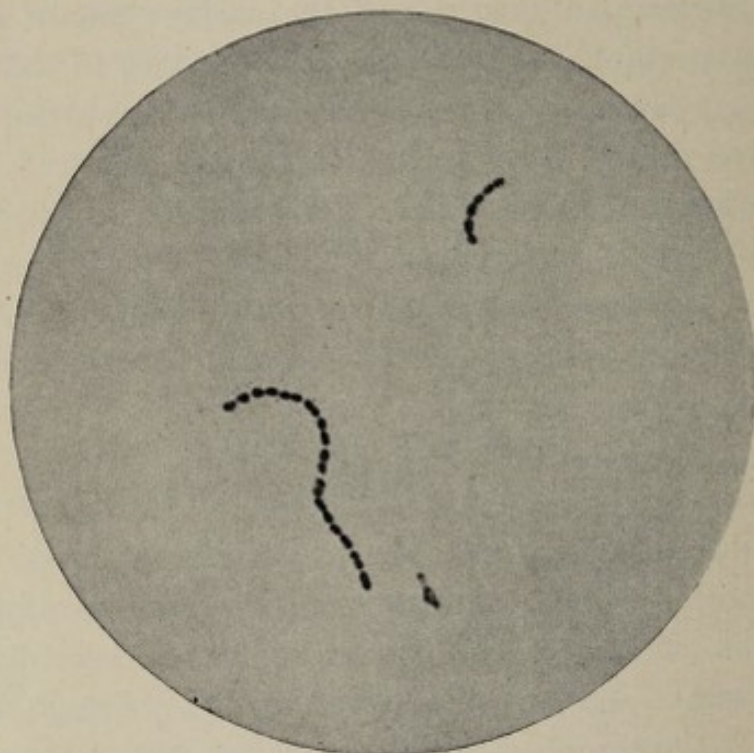
Fig. 142.— Streptococcus lacticus from serum broth (Heinemann).
