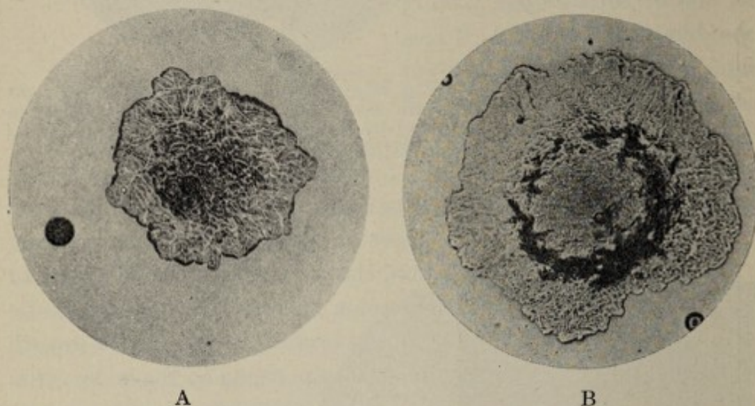
Fig. 72.—Gelatin colonies two days old of (A) bacillus typhosus , and (B) bacillus coli ; \times 21 (Heim).
