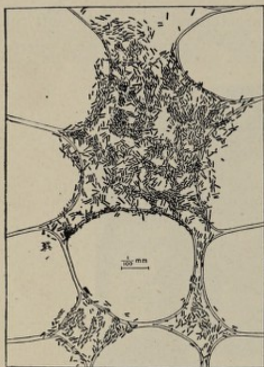
Fig. 158.— B. carotovorus wedging apart cells of the carrot. Drawn mostly from one plane. In placing the cover-glass a few of the bacteria have been crowded out of the intercellular spaces into parts they did not originally occupy. \times 500 (Erwin Smith).
