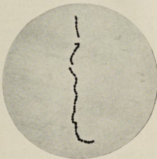
Fig. 32.— Streptococcus pyogenes . Pure culture in bouillon. Fuchsin stain; \times 1000 (Kolle and Wassermann).
