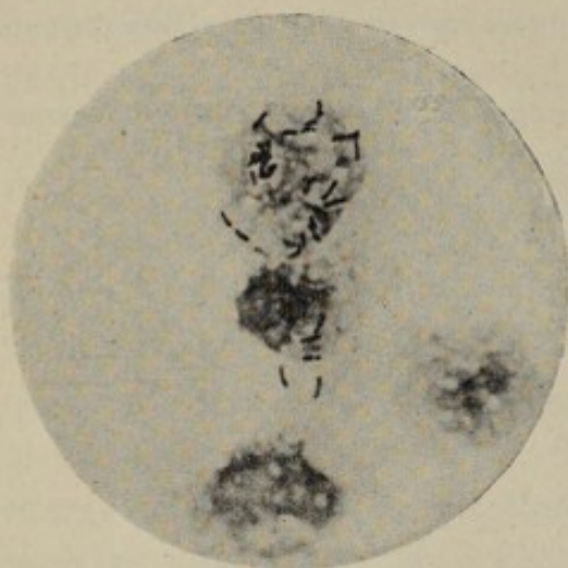
Fig. 92.— Bacillus tuberculosis , human, in pus from lung. Zettinow prep. (Kolle and Wassermann).
