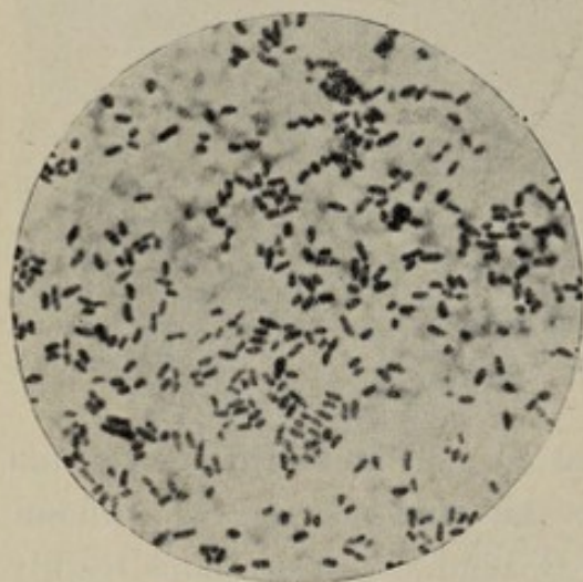
Fig. 67.— Bacillus enteritidis , Gärtner; pure culture; van Ermenegem prep. (Kolle and Wassermann).
