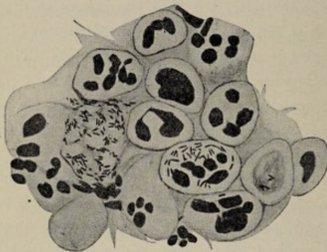
Fig. 84.—Koch-Weeks bacillus in conjunctivitis; \times 900 (Axenfeld, Kolle and Wassermann).
