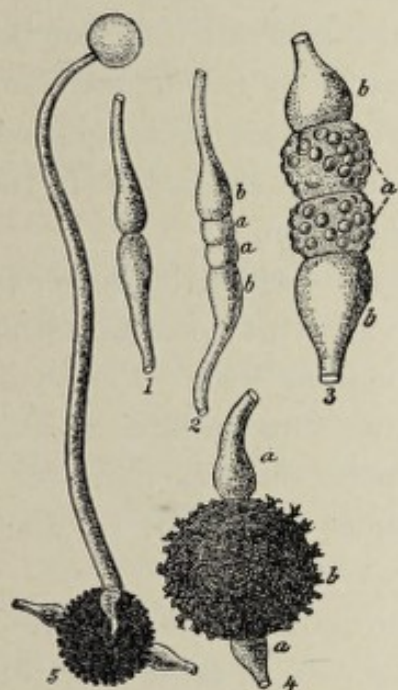
Fig. 123.— Mucor mucedo . Different stages in the formation and germination of the zygospore: 1, Two conjugating branches in contact; 2, septation of the conjugating cells ( a ) from the suspensors ( b ); 3, more advanced stage in the development of the conjugating cells ( a ); 4, ripe zygospore ( b ) between the suspensors ( a ); 5, germinating zygospore with a germ-tube bearing a sporangium (after Brefeld).
