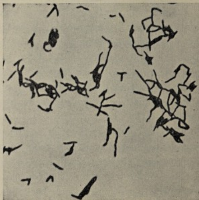
Fig. 113.—Smear preparations of actinomyces from broth culture. \times 1500 (Wright).
