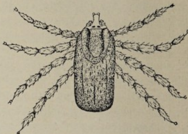
Fig. 139.—Cattle tick, Boophilus bovis . Sexually mature female after last moult (Smith).
