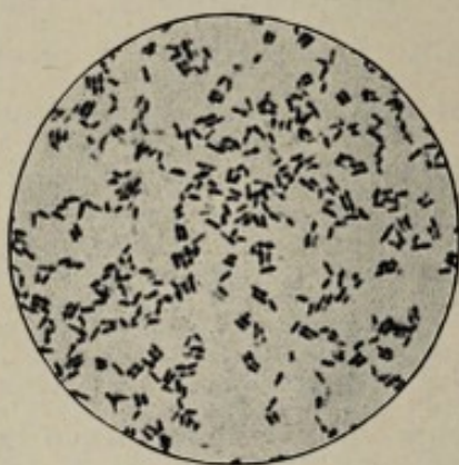
Fig. 61.—Pseudodiphtheria bacillus, methylene-blue; \times 1000 (Park).
