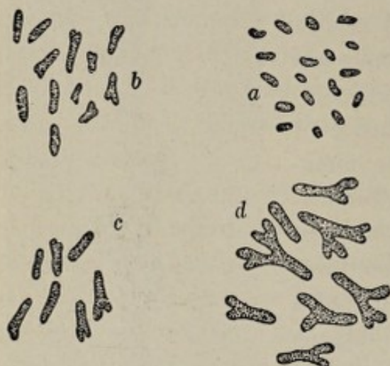
Fig. 148.—Development of root bacteria: a , root-bacteroids; b-d , forms in nodules of Vicia sativa (Beijerinck).
