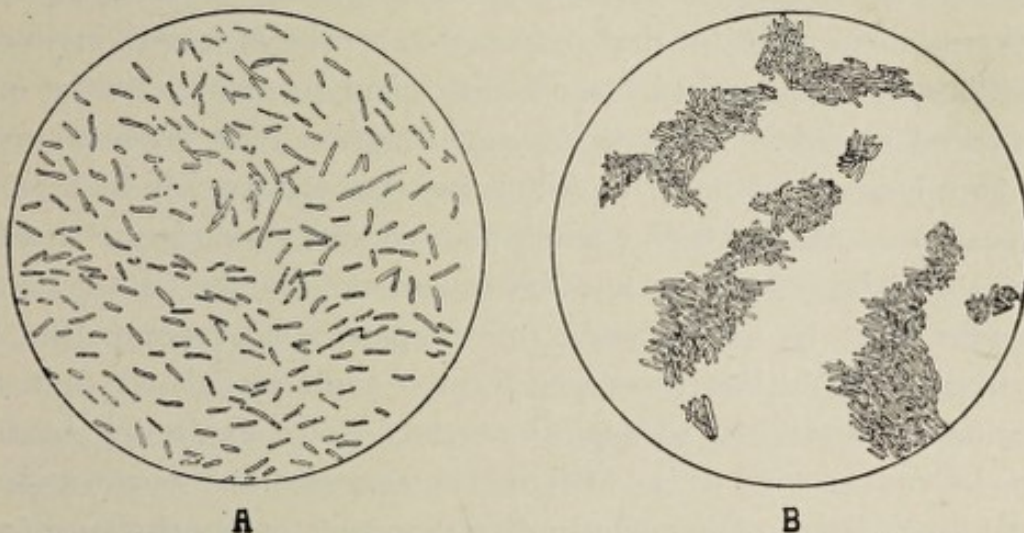
Fig. 74.—Application of the serum-reaction to typhoid bacilli (Williams). A shows the distribution of the bacilli before the reaction. B shows clumping of the motionless bacilli after mixture with the serum of a case of typhoid fever. (Diagrammatic.)
