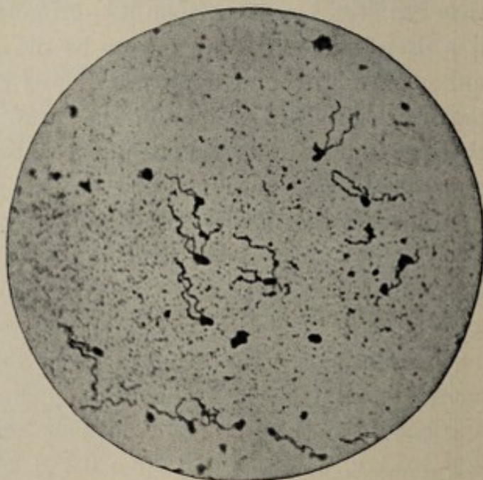
Fig. 64.— Bacillus coli with flagella stained by van Ermengem's method; \times 1000 (Williams).
