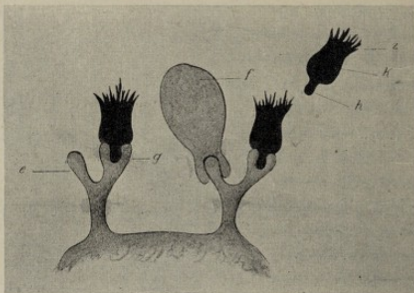
Fig. 24.—Graphic representation of receptors of the third order, and of some substance uniting with one of them: c , Cell-receptor of the third order, amboceptor; e , one of the haptophores of the amboceptor with which some food substance or product of bacterial disintegration, f , may unite; g , the other haptophore of the amboceptor with which complement may unite; k , complement; h , the haptophore, and z , the zymotoxigenic group of the complement (Ehrlich).
