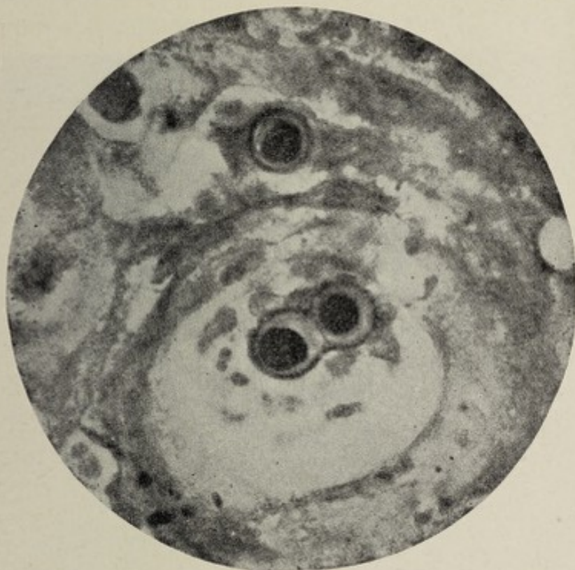
Fig. 120.—Blastomyces. A pair of organisms in an incipient intraepithelial abscess, also a single mature form between epithelial cells. \times about 1200 (Ricketts).
