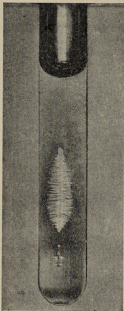
Fig. 86.— Bacillus tetani , gelatin stab-culture, six days (Fränkel and Pfeiffer).
