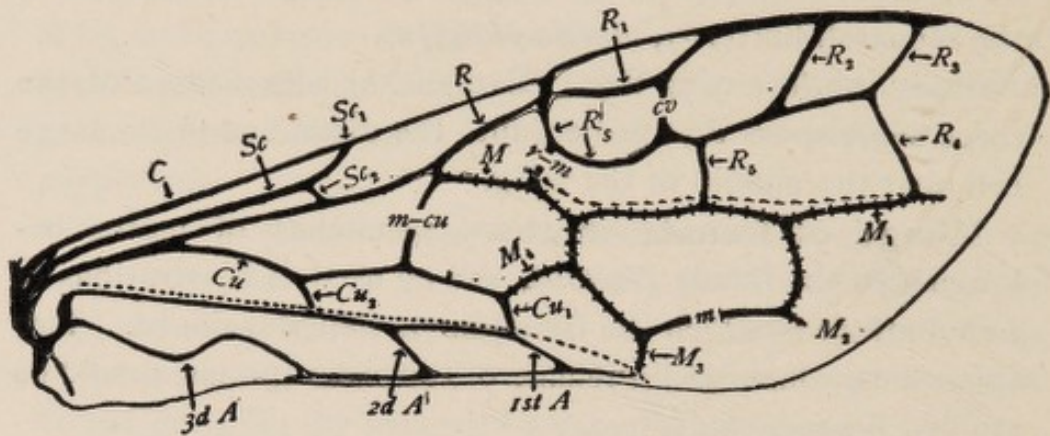
FIG. 6.—The veins of a typical hymenopterous wing.
