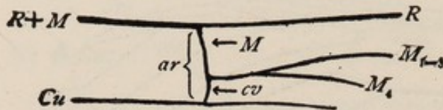
FIG. 4.—The arculus, diagrammatic.
