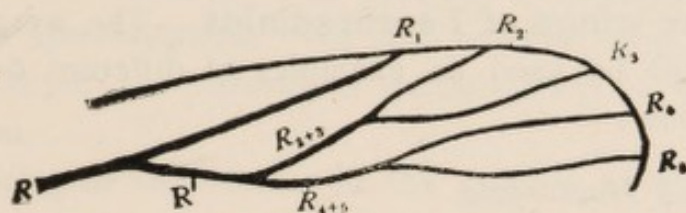
FIG. 8.—The typical radius.
