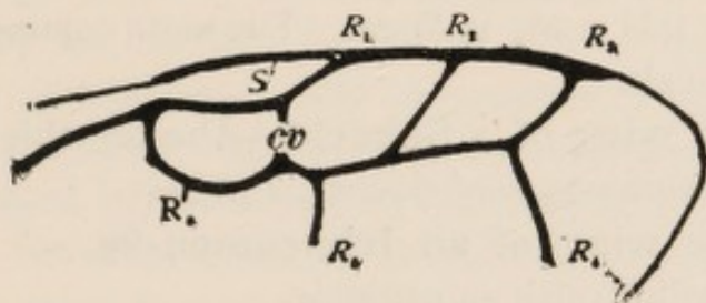
FIG. 9.—The radius in Hymenoptera.
