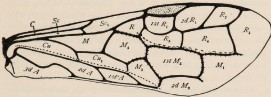
FIG. 7.—The cells of a typical hymenopterous wing.*
