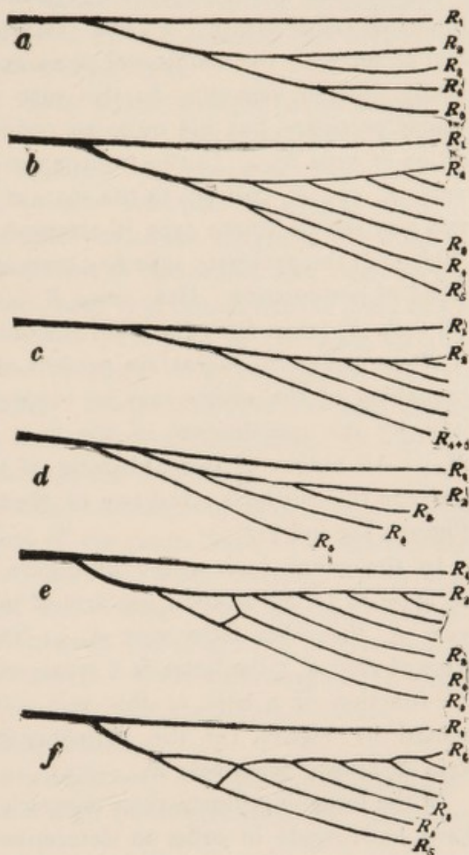
FIG. 11.—Diagrams of several types of radius.
