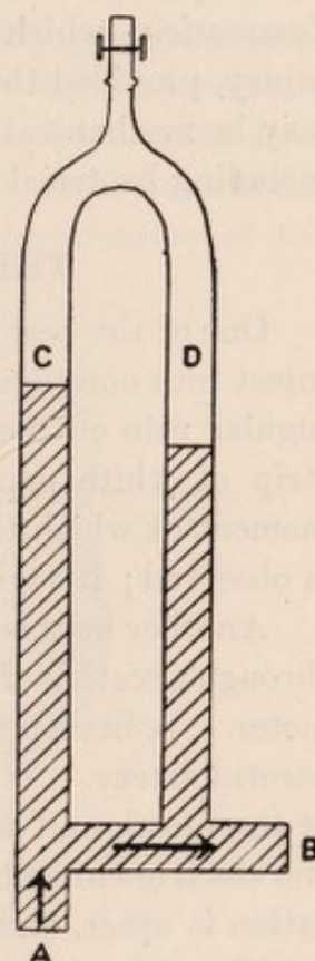
FIG. 78. — Diagram showing the principle of Cybulski's photohæmatachometer.
