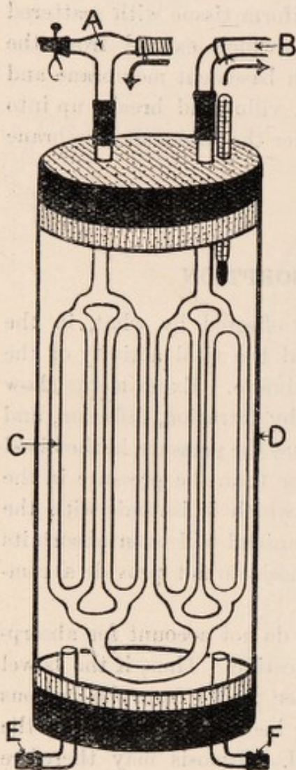
FIG. 153.—Diffusion apparatus (semi-diagrammatic).
