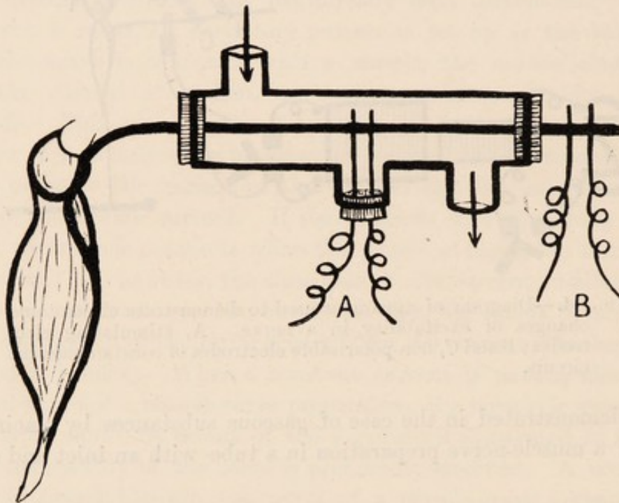
FIG. 16.—Diagram of chamber used to test the effect of gases or volatile drugs on nerve. A, electrodes used to test changes in excitability; B, electrodes used to test changes in conductivity.
