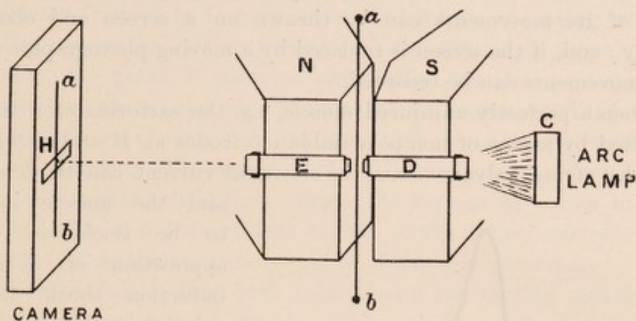
FIG. 10.—Scheme of string galvanometer.
