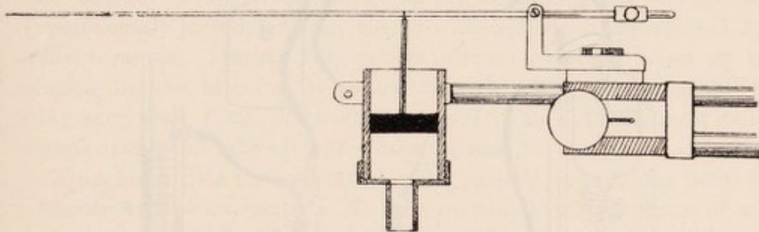
FIG. 87.—Piston recorder. (Diagrammatic.)
