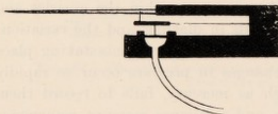
FIG. 84.—Hürthle's manometer. (Diagrammatic.)
