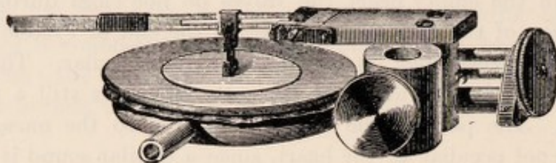
FIG. 83.—Marey's tambour. The writing point of the lever is not shown. (From Messrs Baird & Tatlock.)
