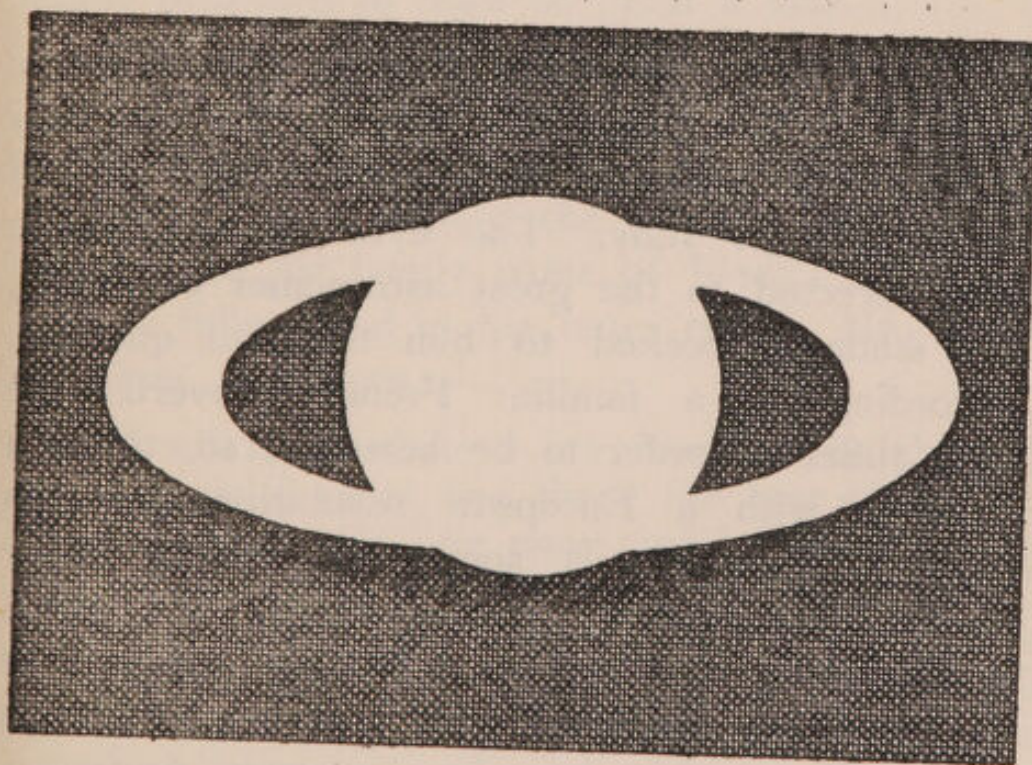
SATURN'S RING AS SEEN BY HUYGENS.
