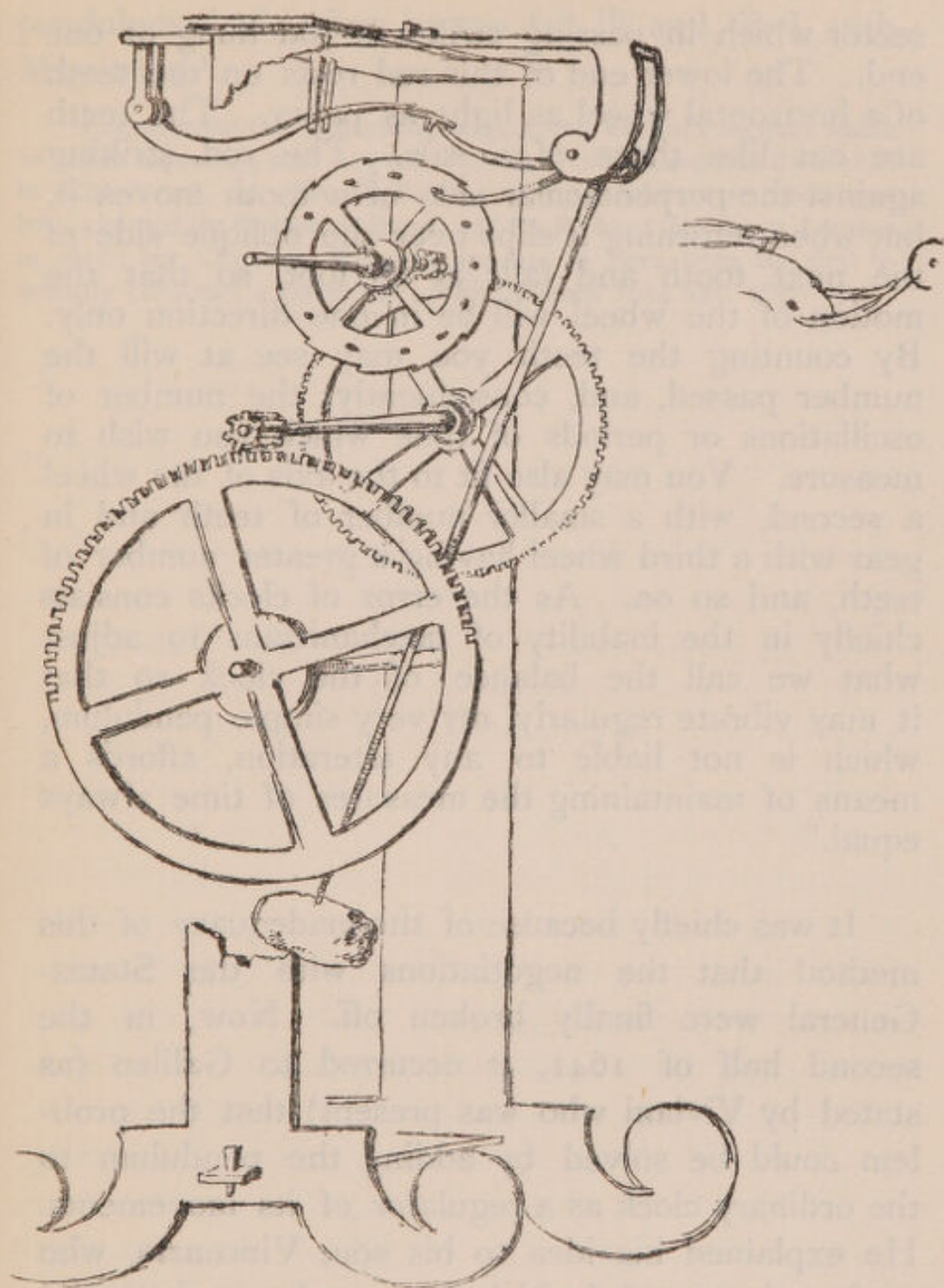
GALILEO'S DESIGN OF A PENDULUM CLOCK ( see next page ).
