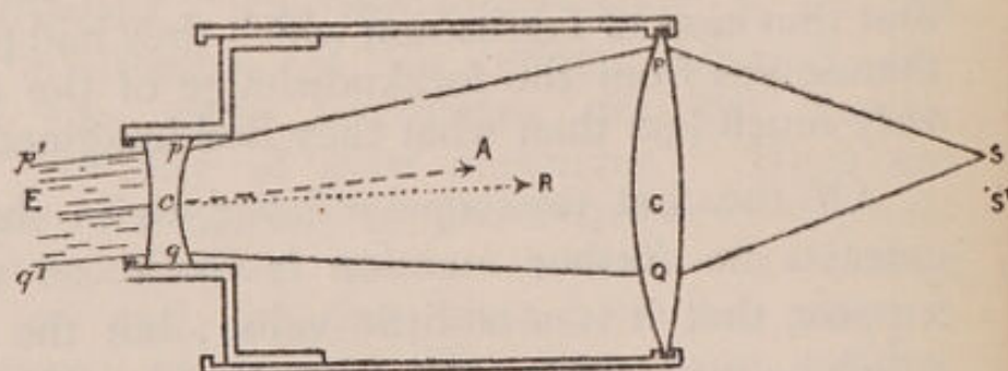
THE GALILEAN TELESCOPE. 1
