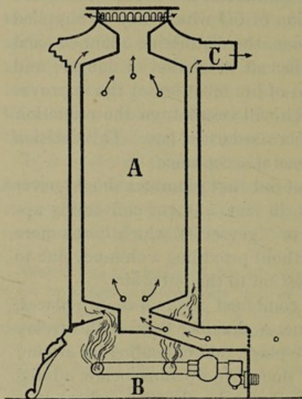
FIG. 34.—EUTHERMIC VENTILATING GAS STOVE.
