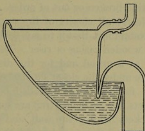
FIG. 15.—WASH-DOWN WATER-CLOSET.
