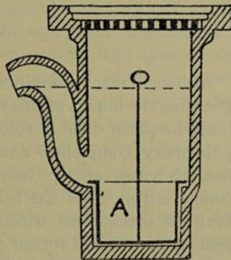
FIG. 29.—DEAN'S SILT GULLEY. A, Cast-iron receptacle to lift in and out.
