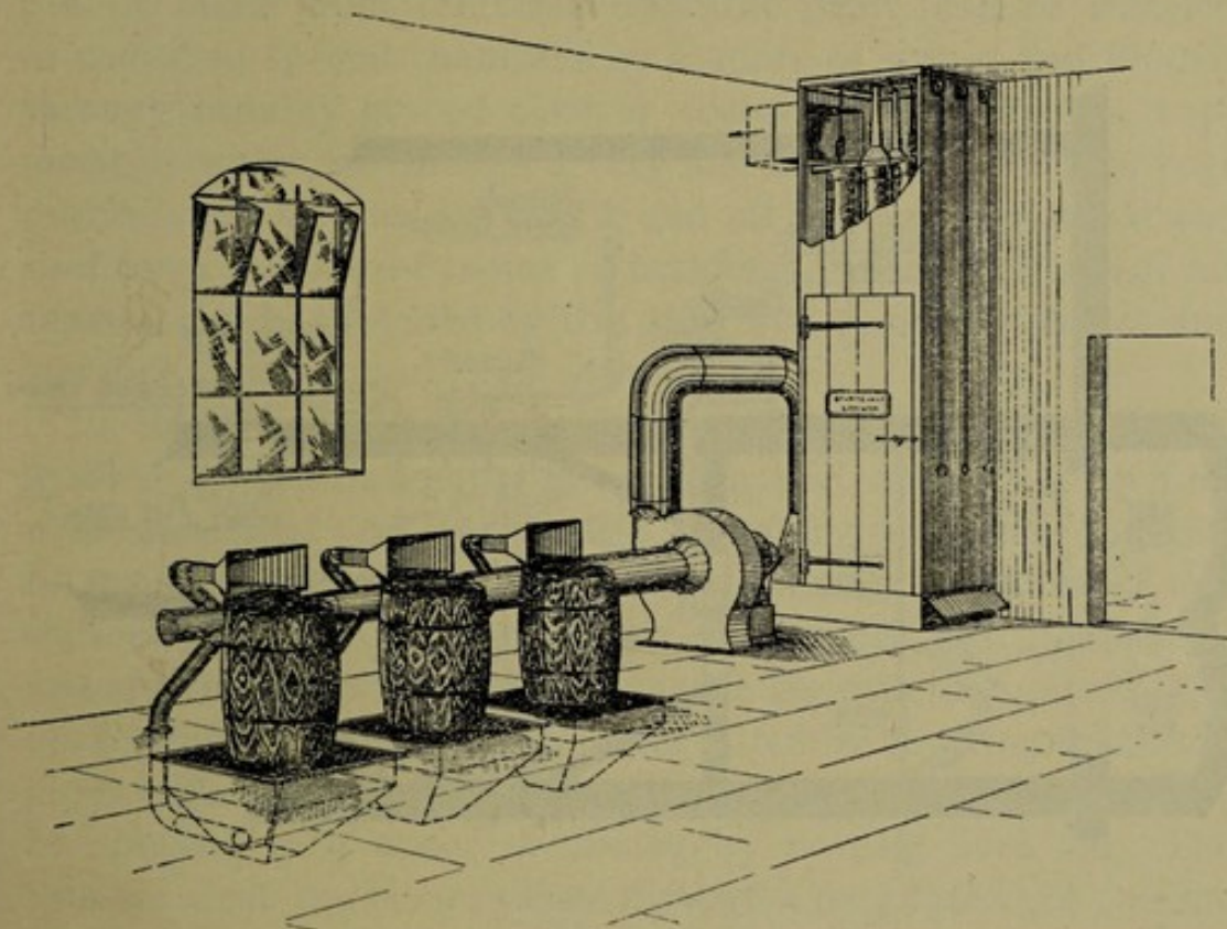
FIG. 31.—STURTEVANT PNEUMATIC DUST COLLECTING SYSTEM.
