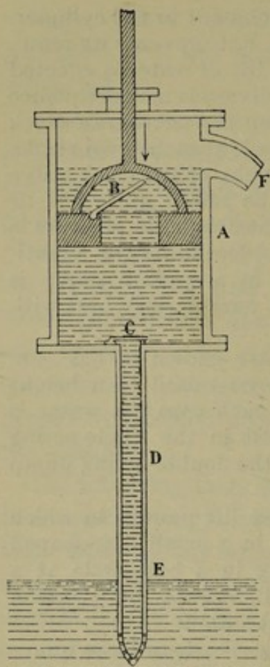
FIG. 4.—SUCTION PUMP.
