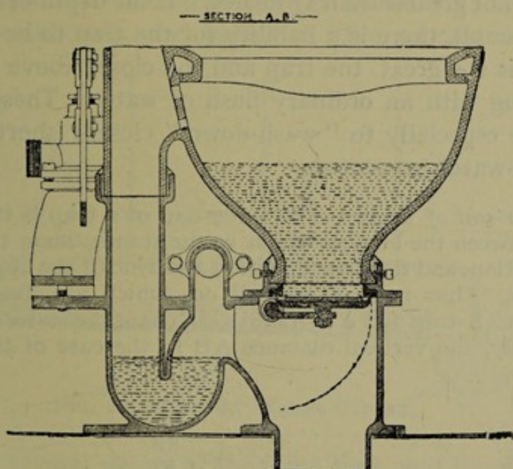
FIG. 18.—ERA VALVE CLOSET.
