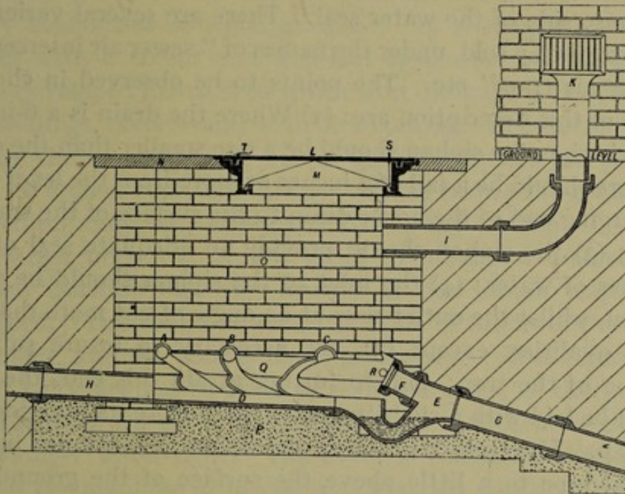
FIG. 26.—SECTION OF DISCONNECTING CHAMBER.
