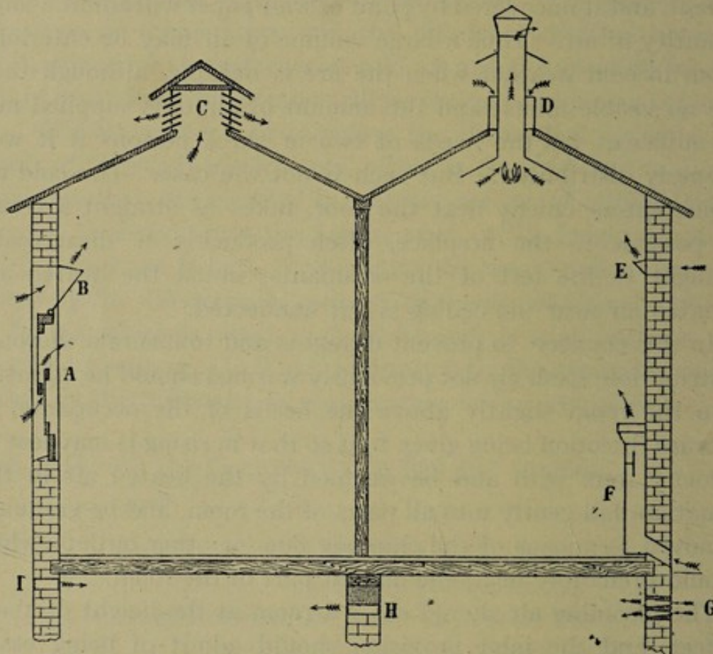
FIG. 30.—DIAGRAMMATIC SKETCH OF VARIOUS PROVISIONS FOR VENTILATION.
