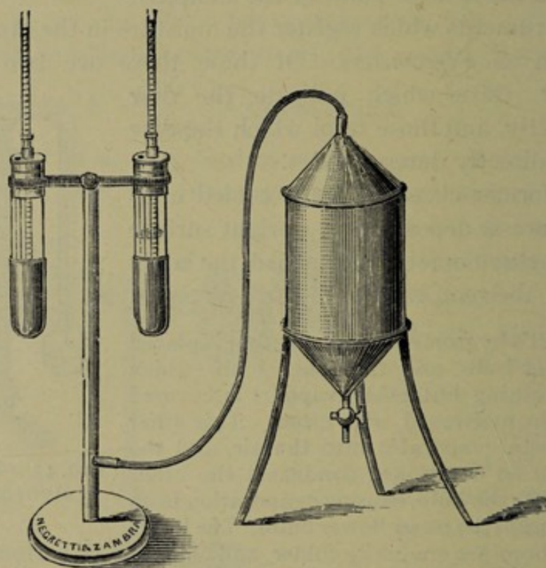
FIG. 44.—REGNAULT'S HYGROMETER.
