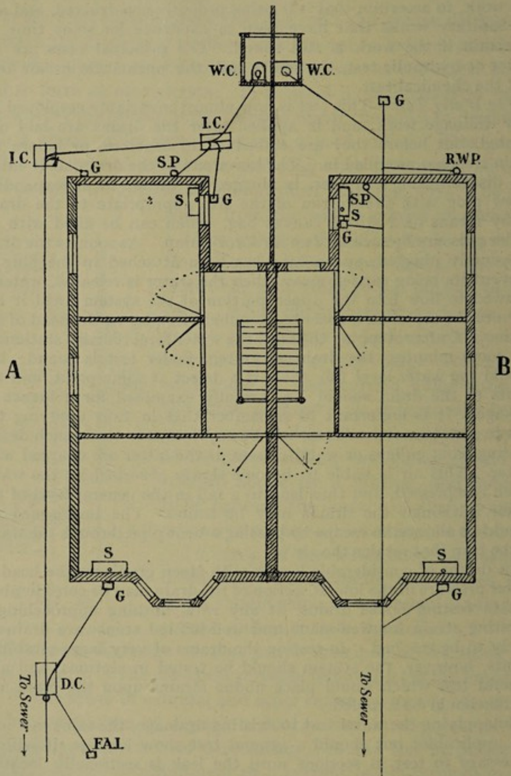
FIG. 28.—SEMI-DETACHED HOUSES.
