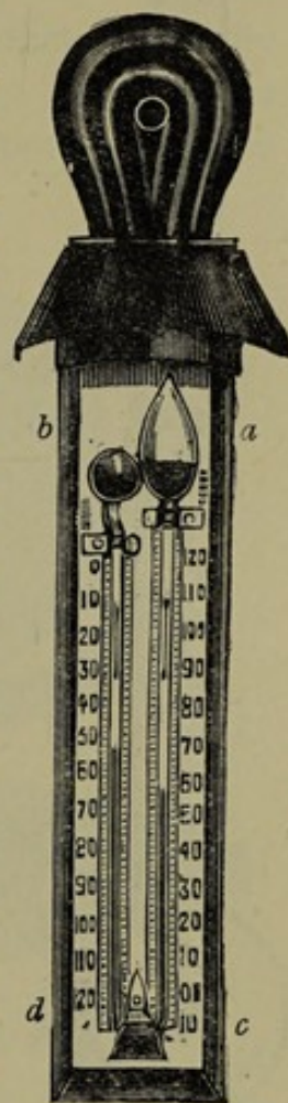
FIG. 47.—SIX'S THERMOMETER.
