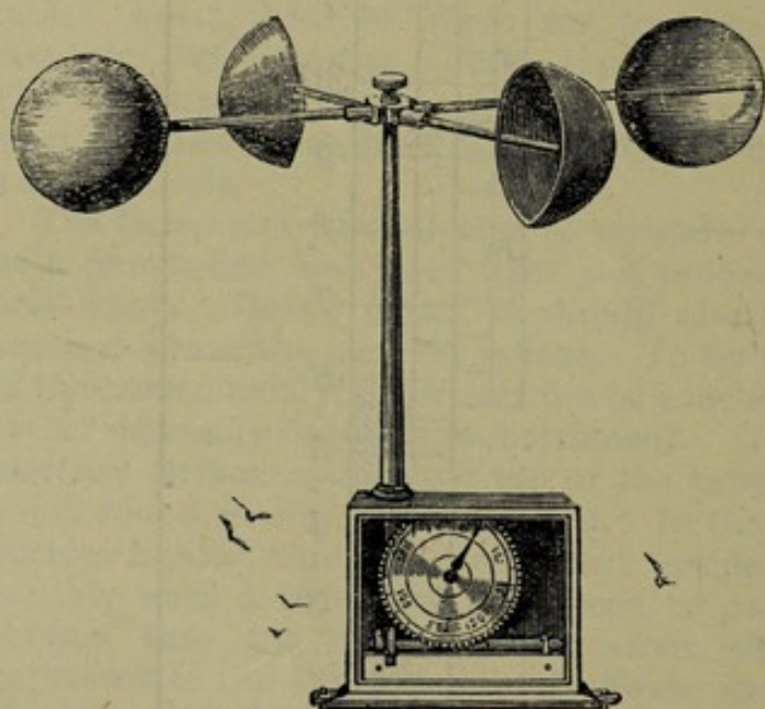
FIG. 42.—ROBINSON'S ANEMOMETER.
