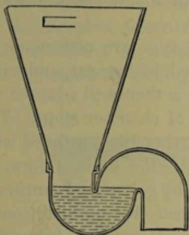
FIG. 14.—LONG HOPPER WATER-CLOSET WITH SIDE-INLET FOR FLUSHING.
