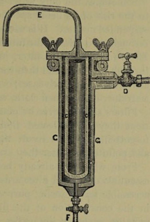
FIG. 10.—BERKEFELD FILTER.
