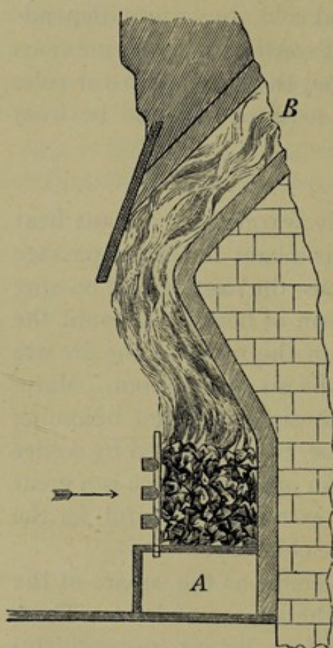
FIG. 33.—RIFLE-BACK STOVE WITH ECONOMIZER.
