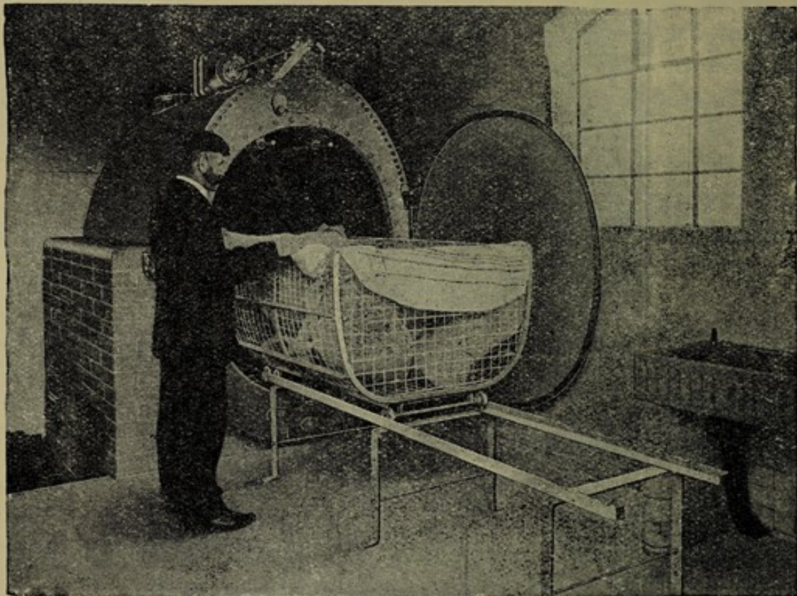
FIG. 89.—FURNACE-HEATED DOUBLE-DOOR DISINFECTOR, SHOWING BRICKWORK SETTING, ETC.
