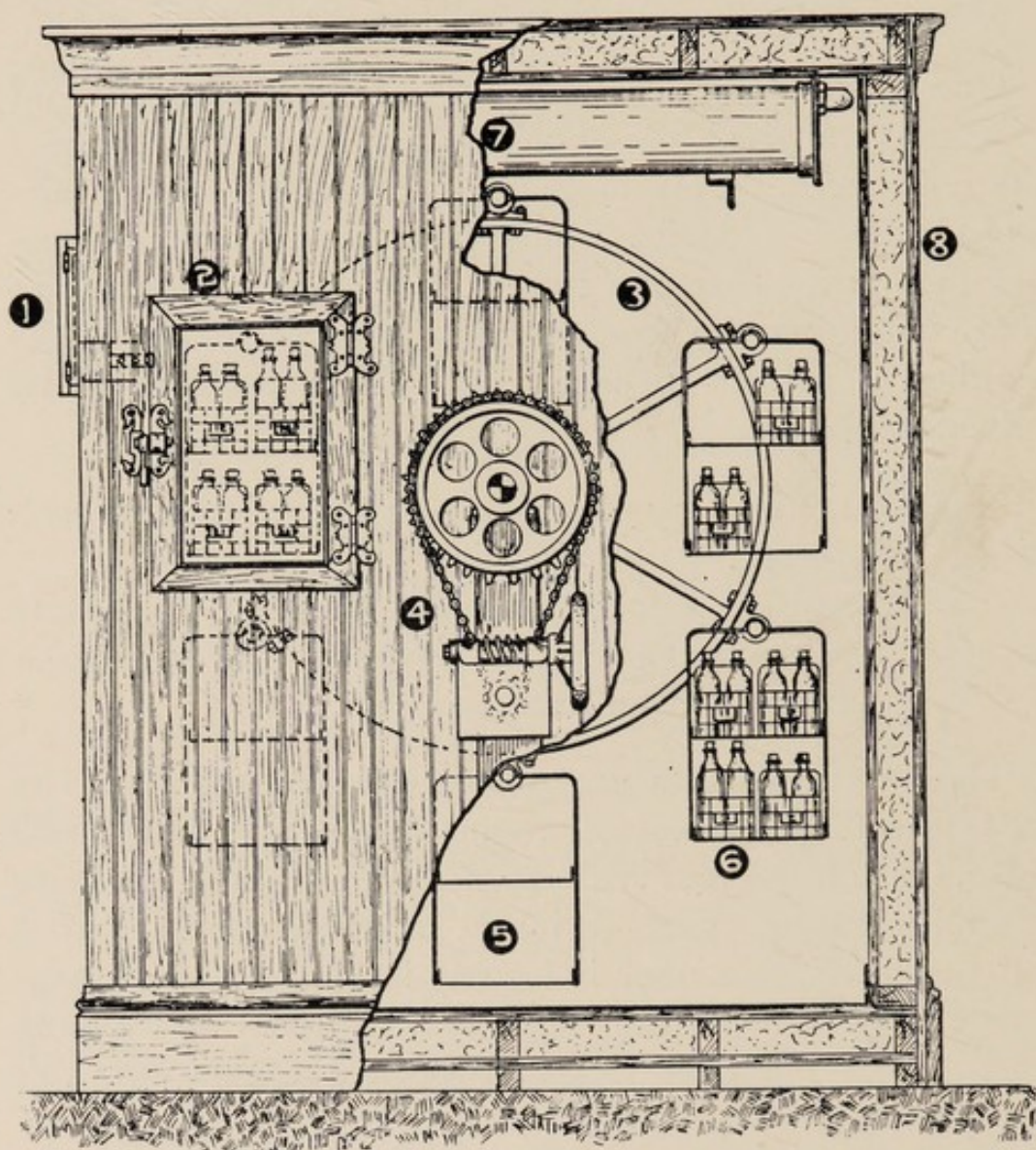
FIG. 8.—DIAGRAMMATIC SKETCH SHOWING THE CONSTRUCTION OF THE COLD STORES.
