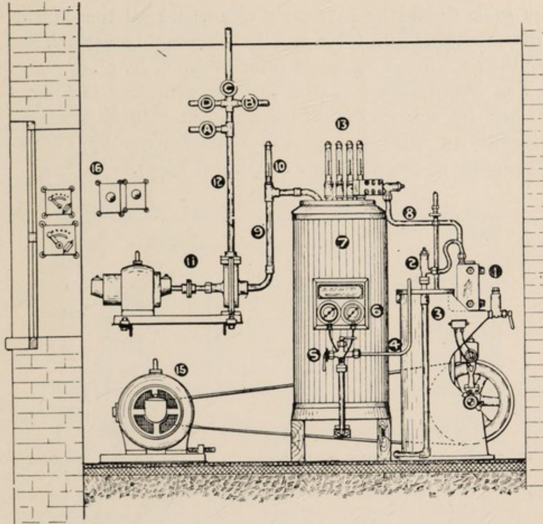
FIG. 6.—DIAGRAMMATIC SKETCH OF THE REFRIGERATING MACHINERY.
