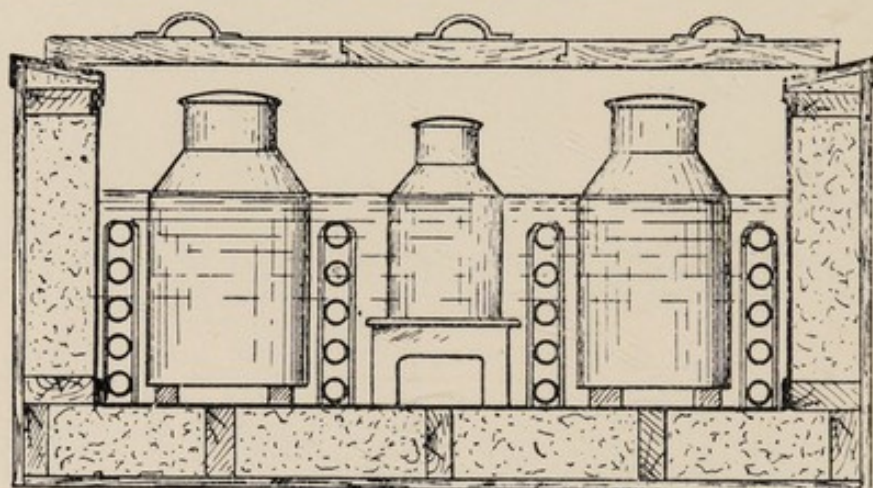
FIG. 7.—COOLING TANK FOR REDUCING SOLUTIONS TO THE REQUIRED TEMPERATURE: AN INSULATED TANK CONTAINING BRINE.
