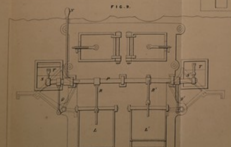
Section thro' EF.
