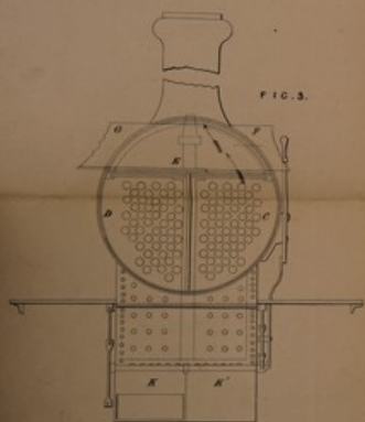
Section thro' GH.
