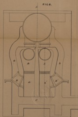
Section thro' EF.
