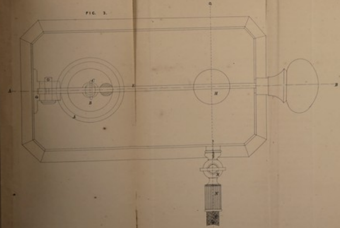
Plan of the double condole (front view of double bellows)
