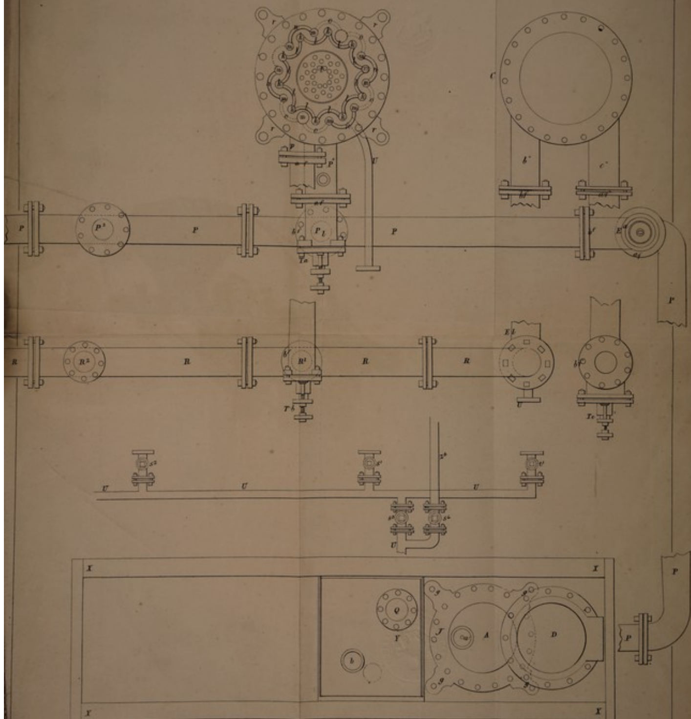
Fig. 1. Plan of the Apparatus. Scale one inch to the feet.
