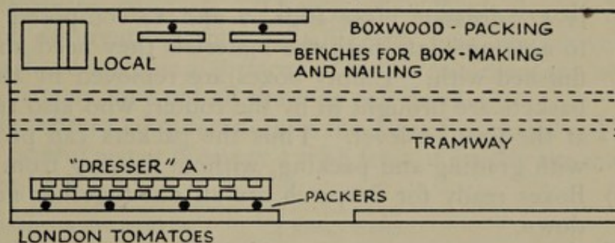
Packing shed of Nursery 2 ( showing suggested reorganisation of work )
