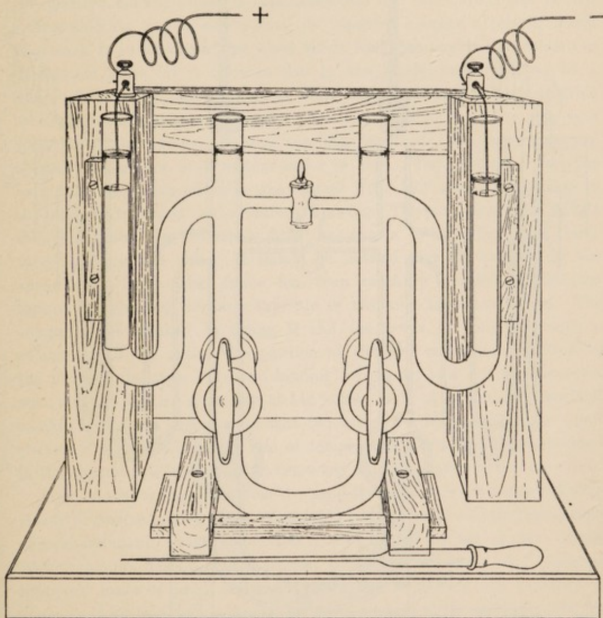
FIG. 1.—Perspective view of apparatus. (Half scale.)
