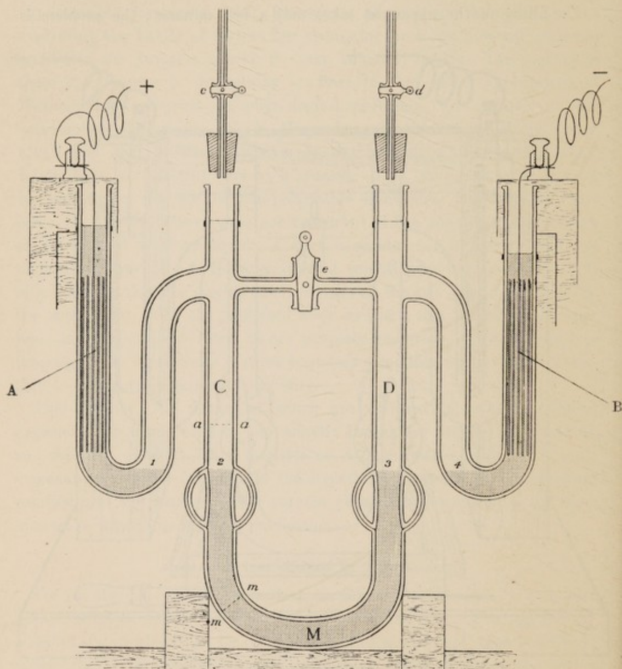
FIG. 2.—Section of apparatus. (Half scale.)
