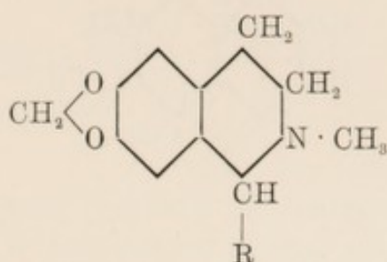
Strychnine-like.
