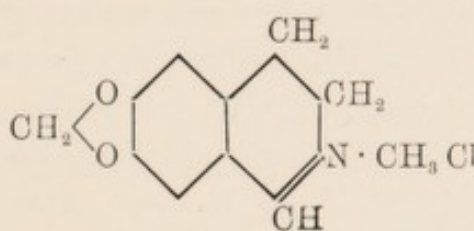
Not Strychnine-like.
