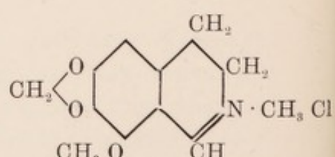
Cotarnine chloride.
