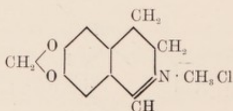
Hydrastinine chloride.
