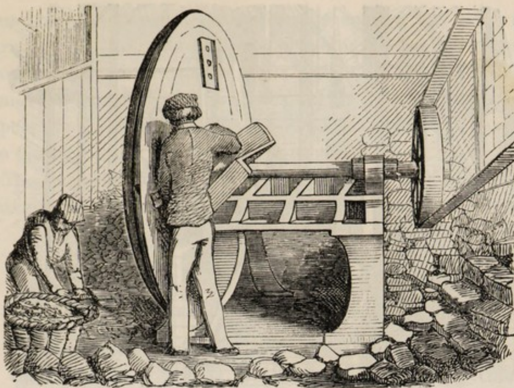
Fig. 5. Cutting Machine.
