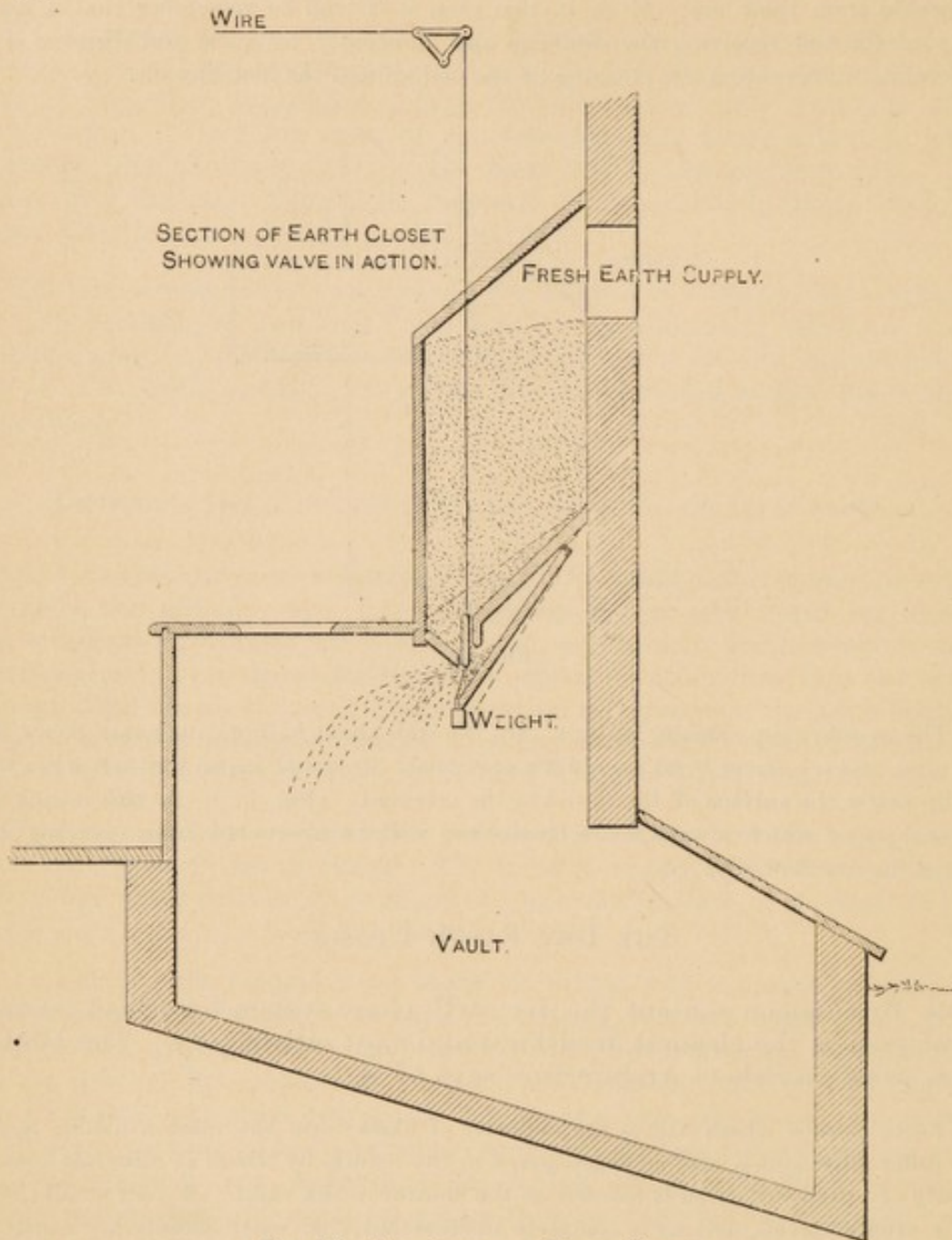
FIG. 12.—SECTION OF AN EARTH CLOSET.
