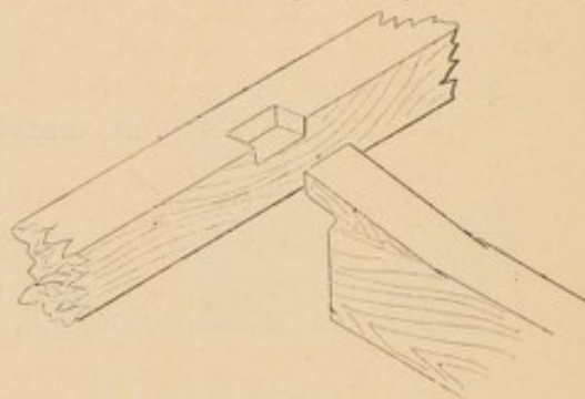
FIG. 29.—A NOTCHED SILL.
