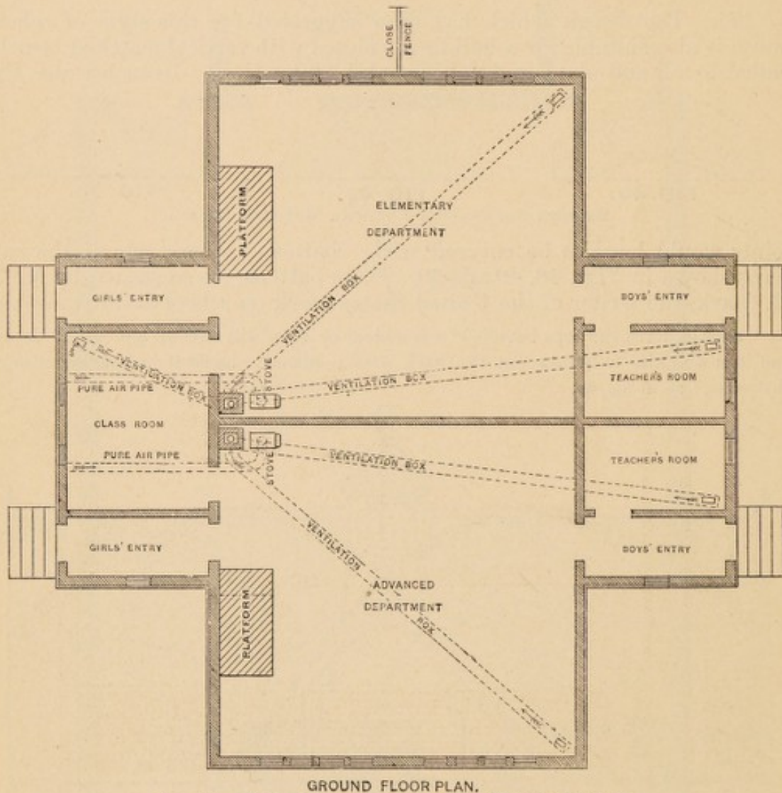
FIG. 52.—FOR A RURAL, OR VILLAGE GRADED SCHOOL.
