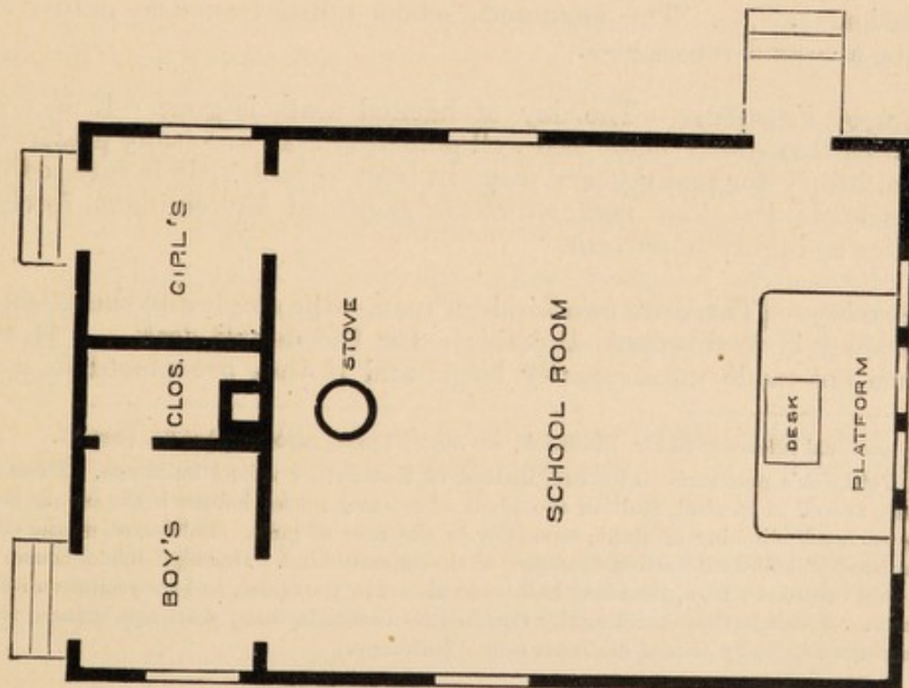
FIG. 59.—GROUND PLAN OF THE RURAL SCHOOL HOUSE, LITCHFIELD.
