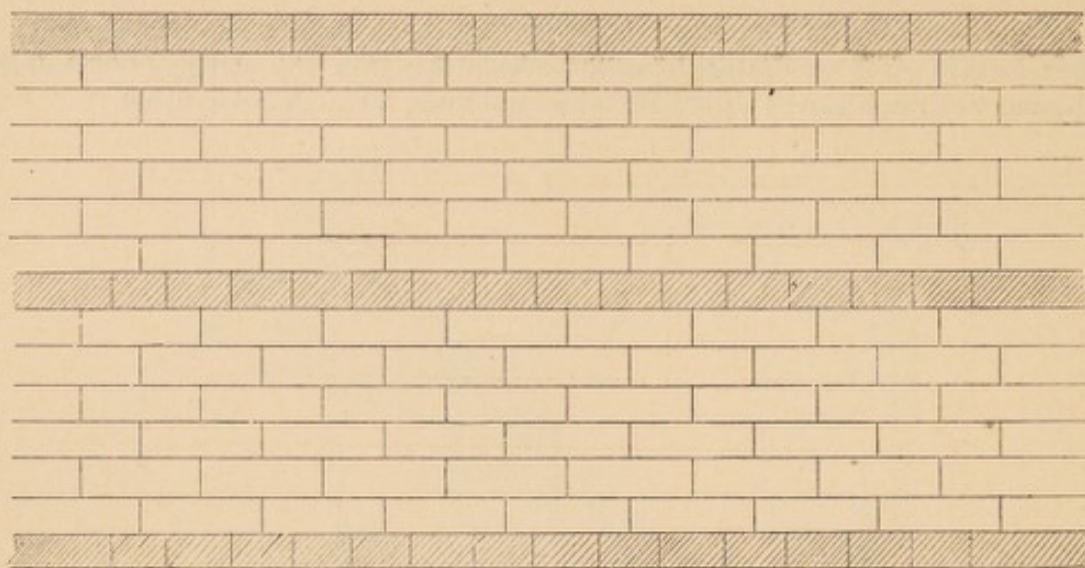
FIG. 28.—SYSTEM OF BRICK BONDINGS.
