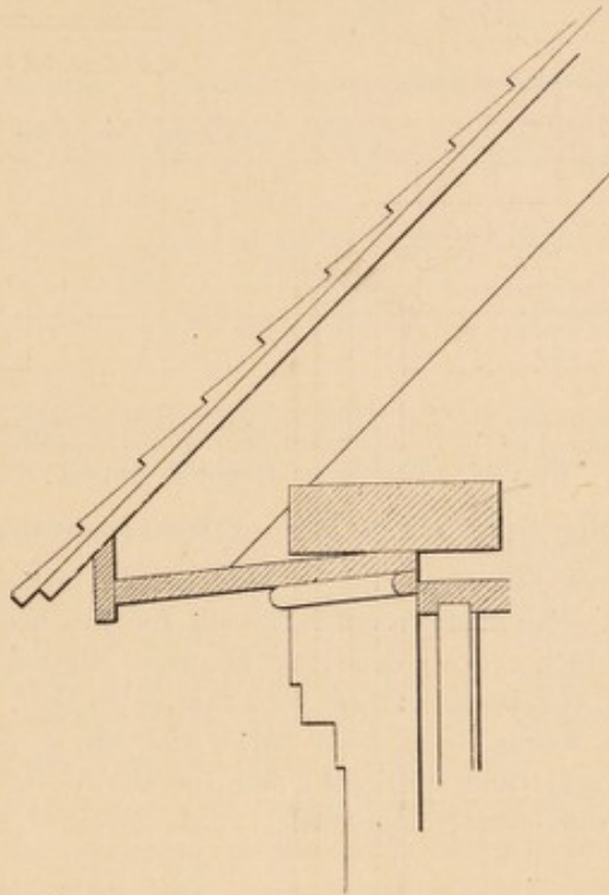
FIG. 23.—SECTION OF BRICK CORNICE.
