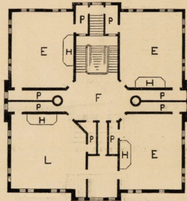
FIG. 57.—UPPER FLOOR OF A TWO-STORY SCHOOL HOUSE.
