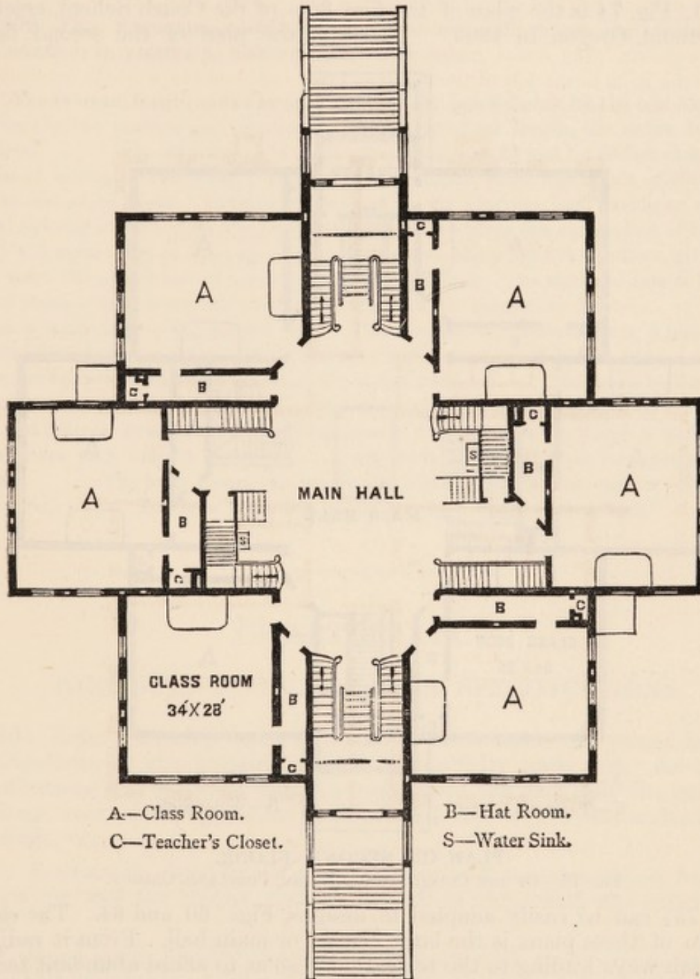
FIG. 74.—OF THE COUCH SCHOOL HOUSE, PORTLAND, OREGON.
