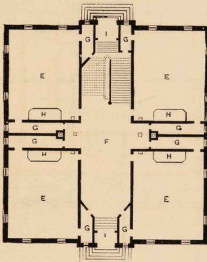
FIG. 62.—GROUND PLAN OF A TWO-STORY SCHOOL HOUSE.
