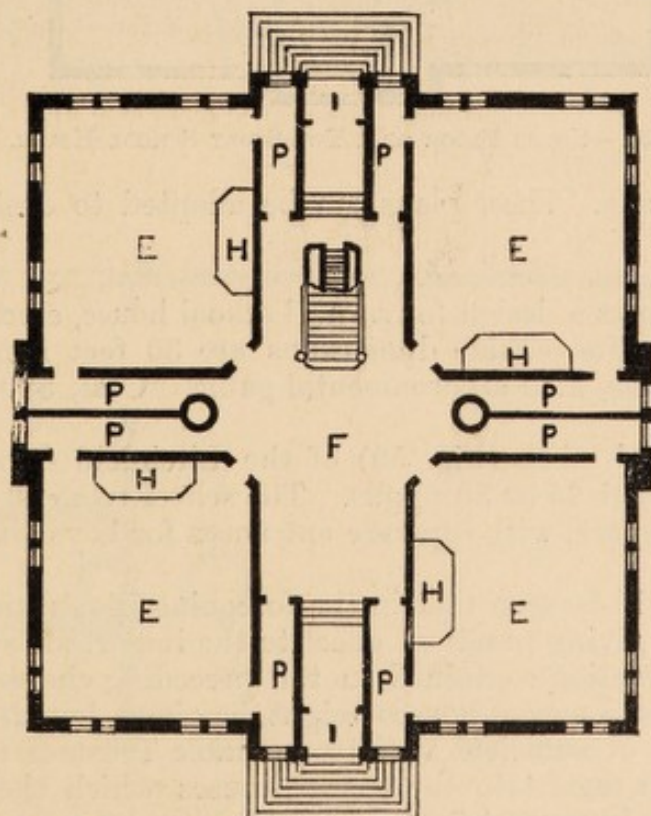
FIG. 56.—GROUND PLAN OF A TWO-STORY SCHOOL HOUSE.
