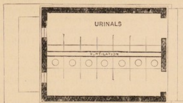
FIG. 10.—COMBINED URINAL AND LATRINE FOR BOYS.
