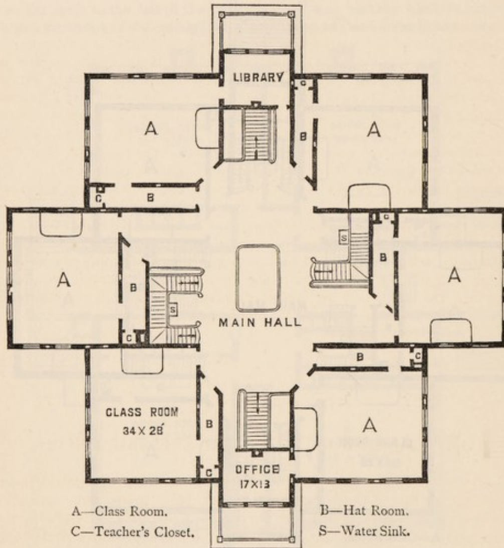
PLAN OF SECOND FLOOR.
