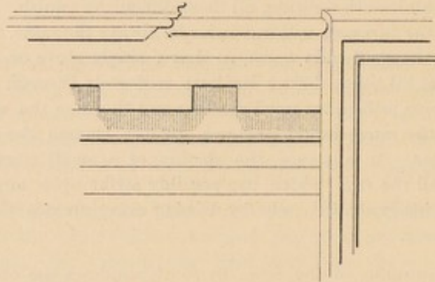
FIG. 40.—WINDOW OPENING, SHOWING OUTSIDE CORNICE.
