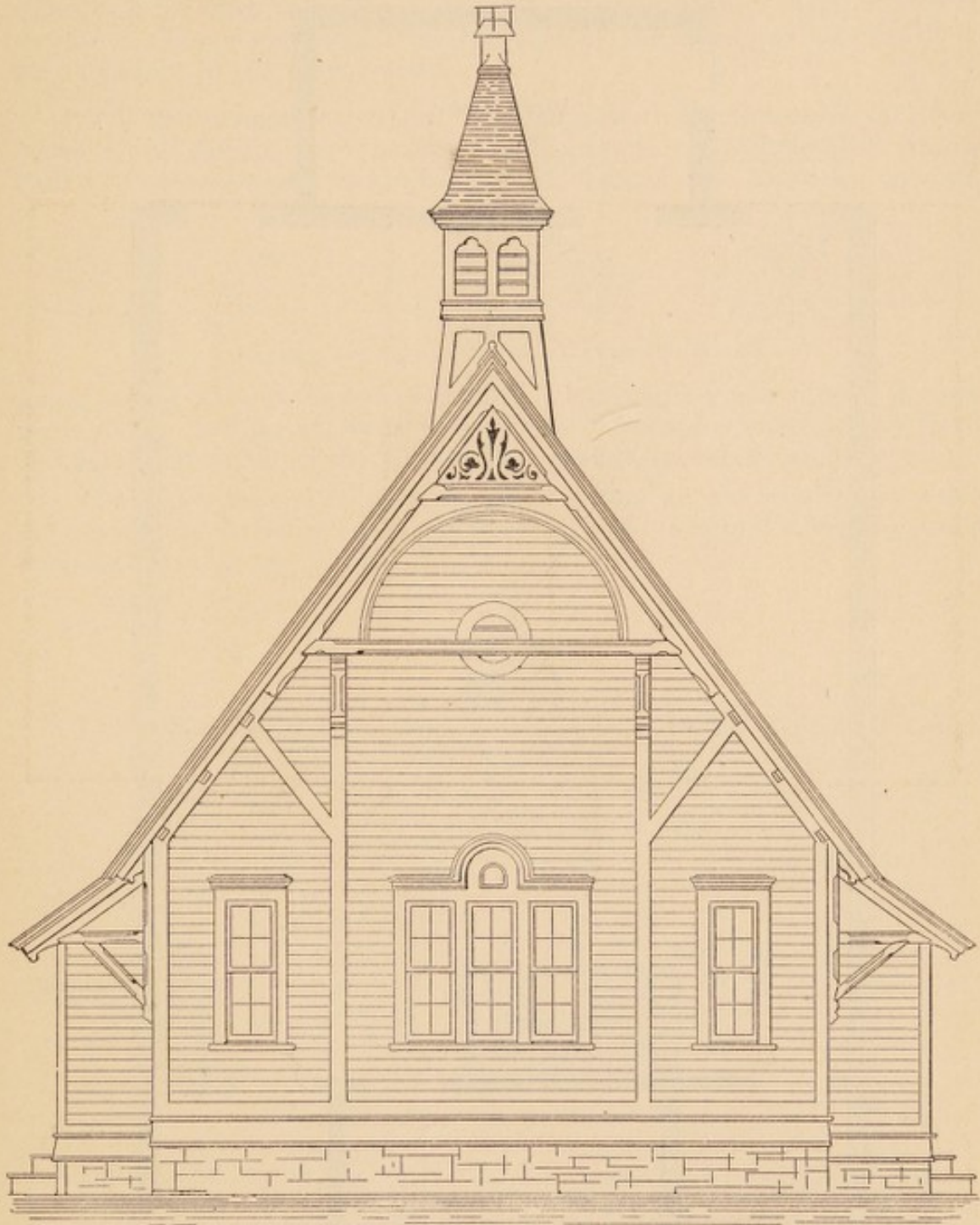
FIG. 46.—DESIGN FOR A RURAL OR A VILLAGE SCHOOL HOUSE.
