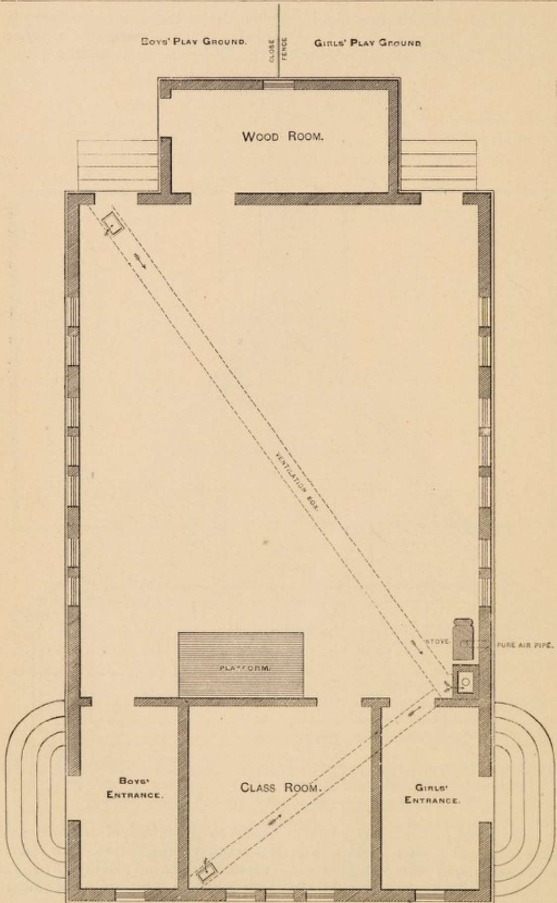
FIG. 47.—ADAPTED TO THE DESIGN SHOWN IN FIG. 46.
