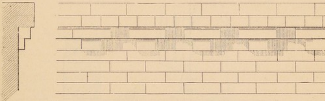
FIG. 18.—CORNICHE OF PROJECTING BRICKS AND SECTION, NO. 1.
