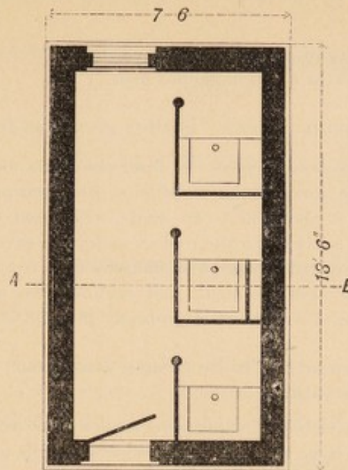
FIG. 9.—LATRINE FOR GIRLS.
