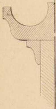
FIG. 32.—CHALK TRAY MOULDING, No. 1.
