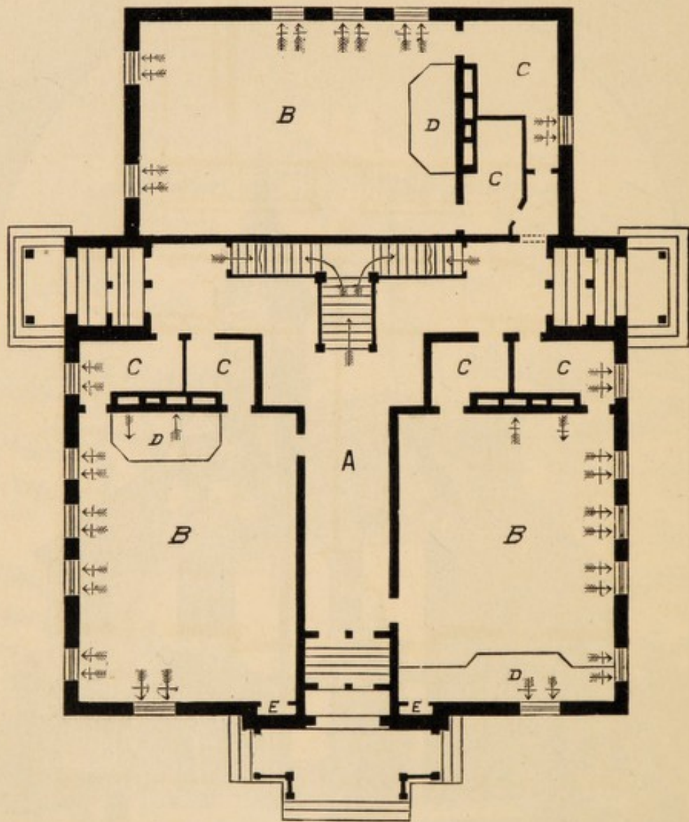
FIG. 65.—GROUND PLAN ADAPTED TO THE FOREGOING DESIGN.
