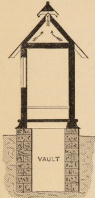
FIG. 7.—SECTION.
