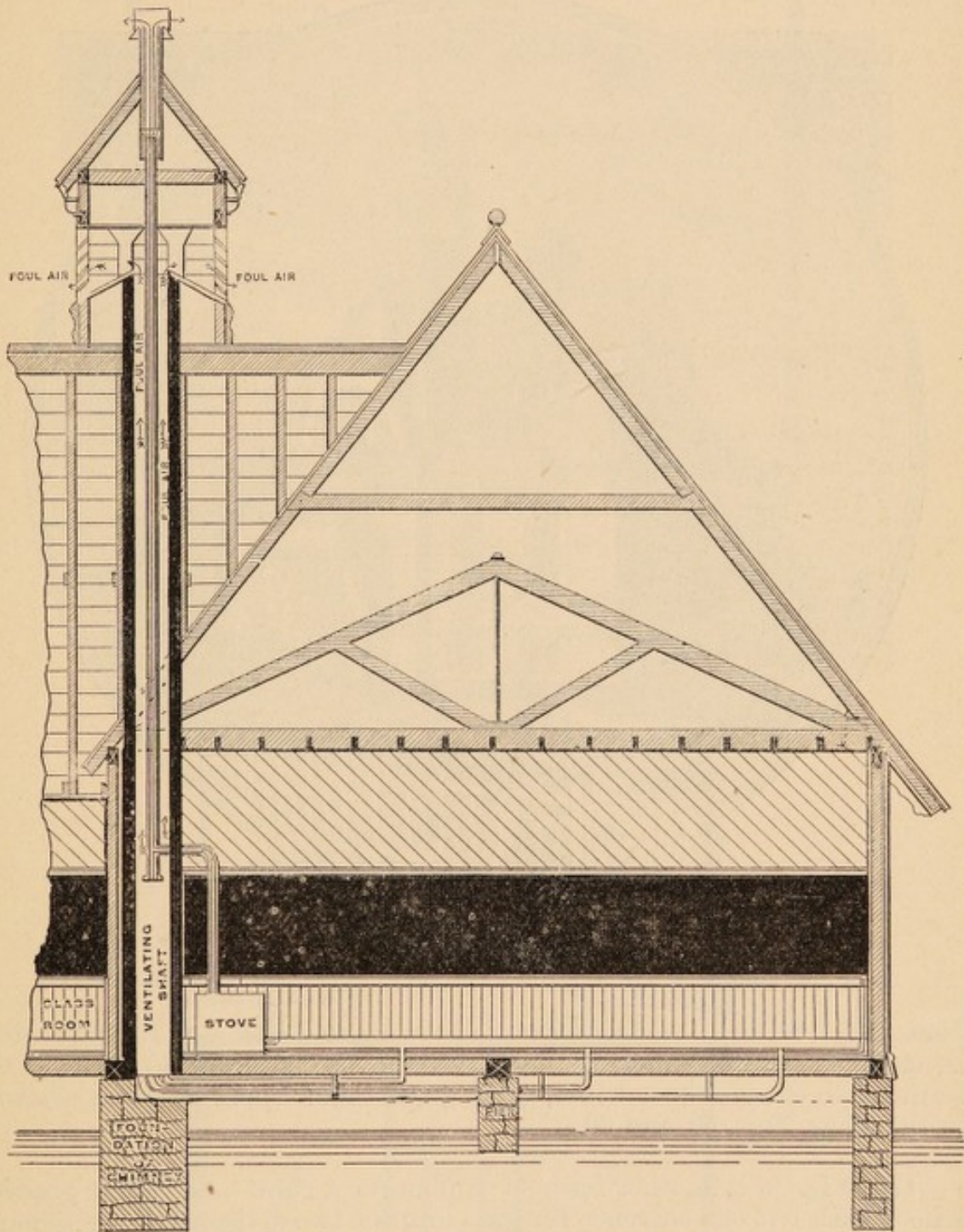
FIG. 53.— SECTION OF THE SCHOOL HOUSE, FIGS. 51 AND 52.
