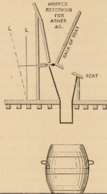
FIG. 13.—SECTION OF DRY ASH SYSTEM.
