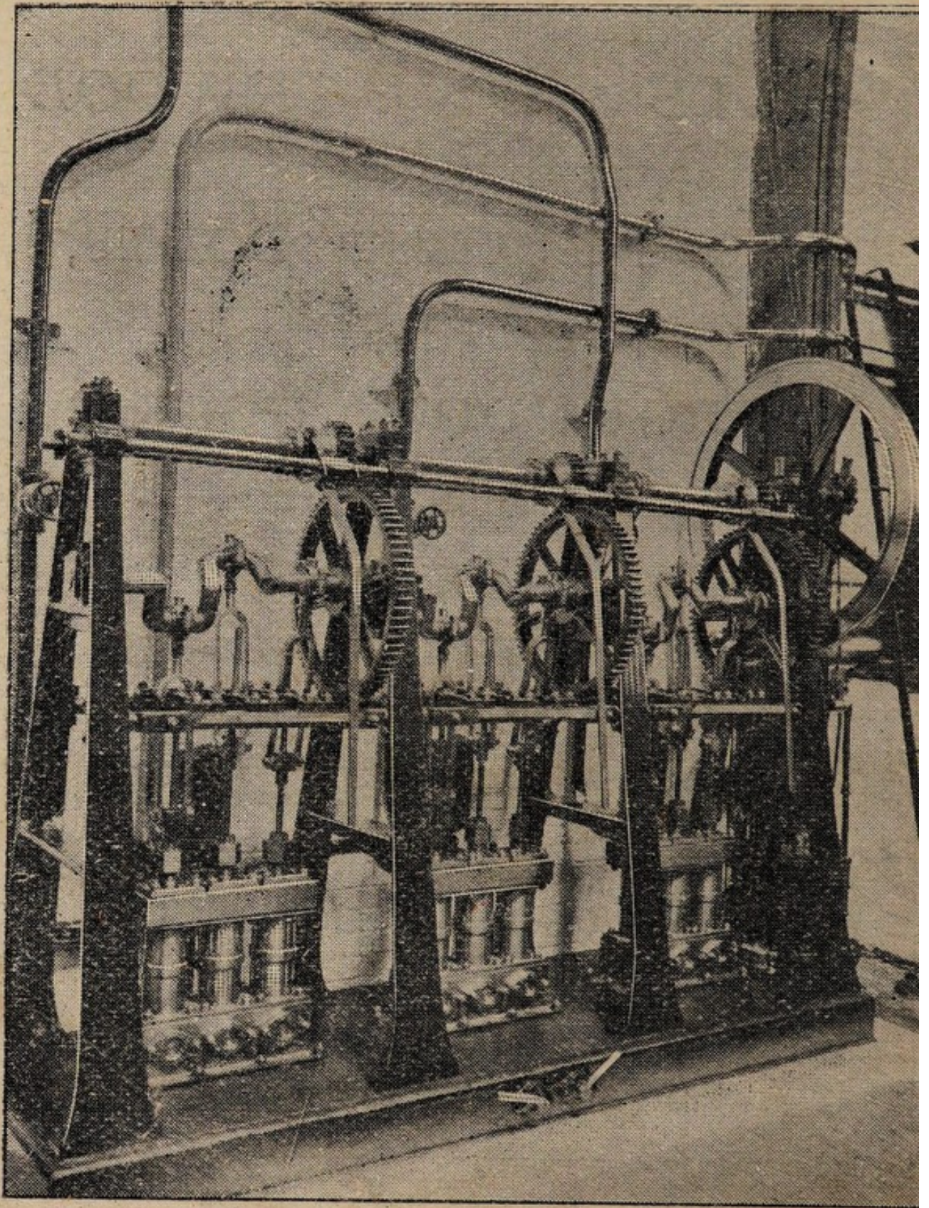
PUMPS IN HILLS & UNDERWOOD'S DISTILLERY, NORWICH.
