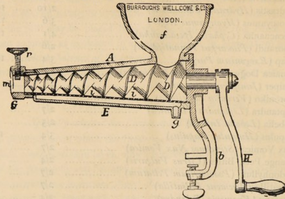
SECTIONAL VIEW OF TINCTURE PRESS.
