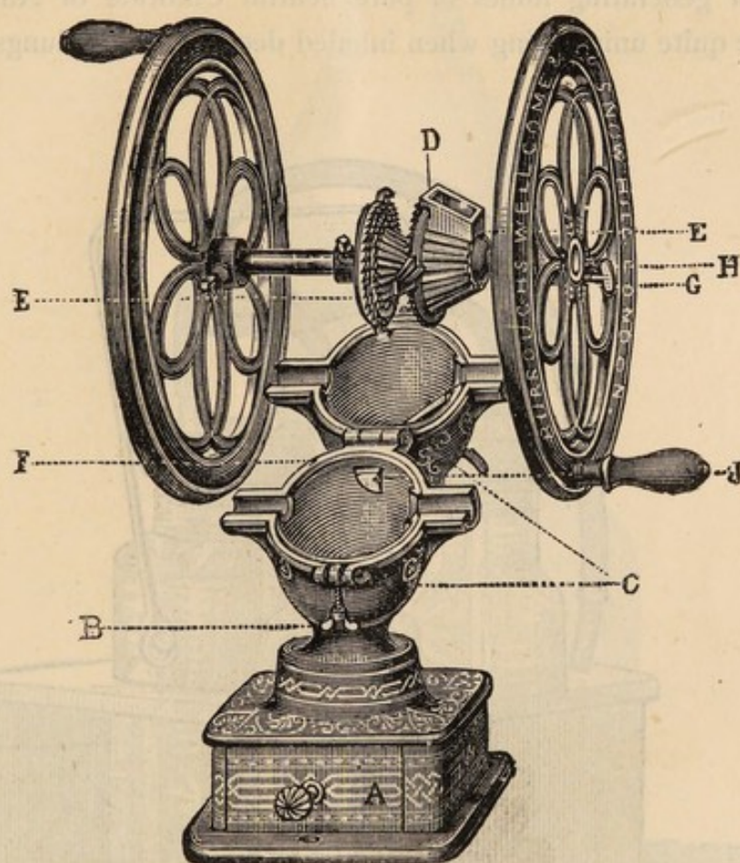
SECTIONAL VIEW.
