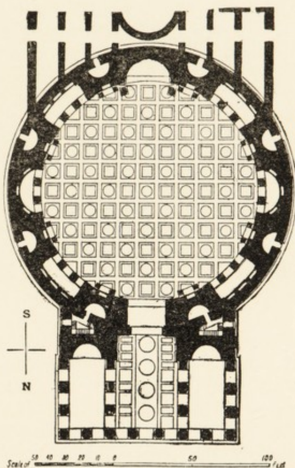
FIG. 5.—PLAN OF THE PANTHEON
