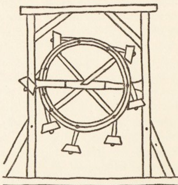
Honnecourt's Overbalanced Wheel.
