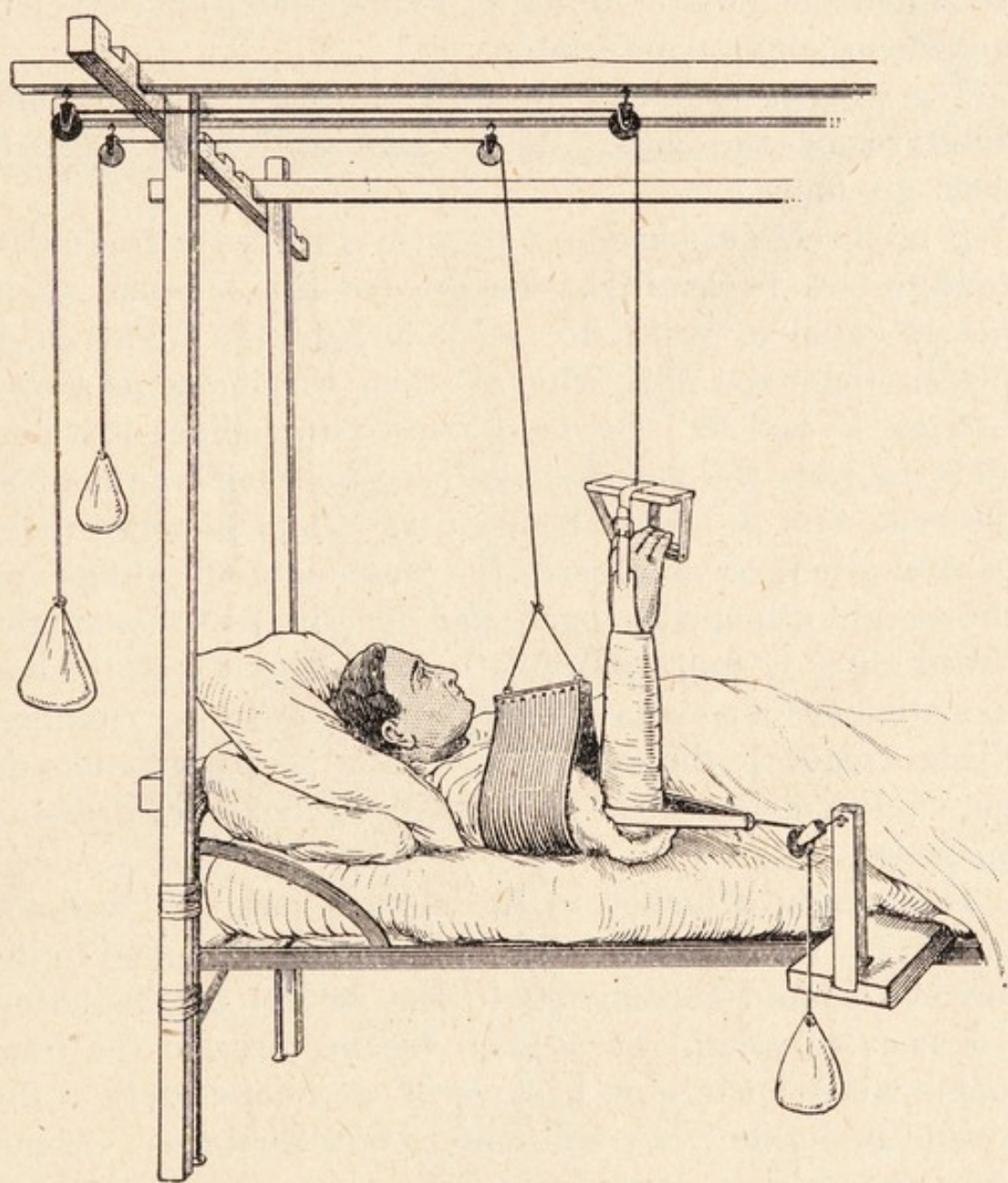
FIG. 18. — A simple method for producing traction and at the same time regulating abduction. The pulley for the weight is attached to an upright fixed at the end of a rough unplanned board which is slipped in under the mattress. The desired abduction is obtained by adjusting the position of the board.
