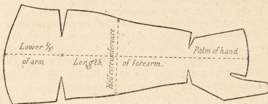
FIG. 40. — Method of cutting thicknesses of crinoline to make moulded plaster splint for wrist.
