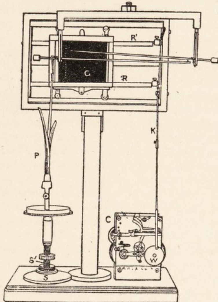
FIG. 17.—The High Magnification Crescograph. P, plant ; C, clockwork for periodic oscillation of recording smoked glass plate (G) ; S S', micrometer screws ; K, crank ; R, eccentric ; W, rotating wheel.
