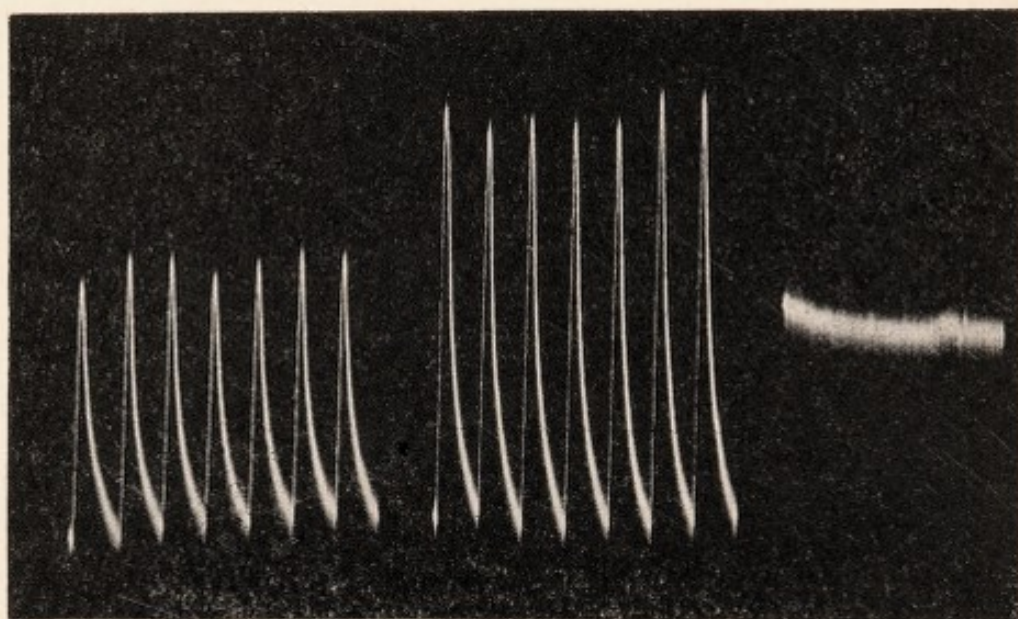
FIG. 6.—Stimulating action of minute quantity of 'poison' which in large doses abolishes the response of metal.
