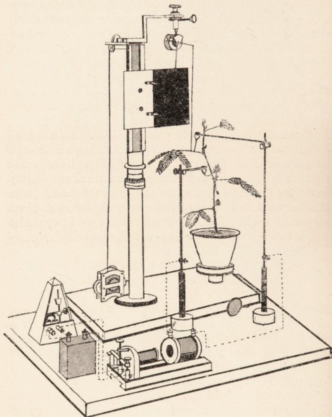
FIG. 11.—General view of the Resonant Recorder and the electrical connections by which excitatory shock of a definite duration is given to the plant; duration of shock determined by metronome, which completes electric circuit.
