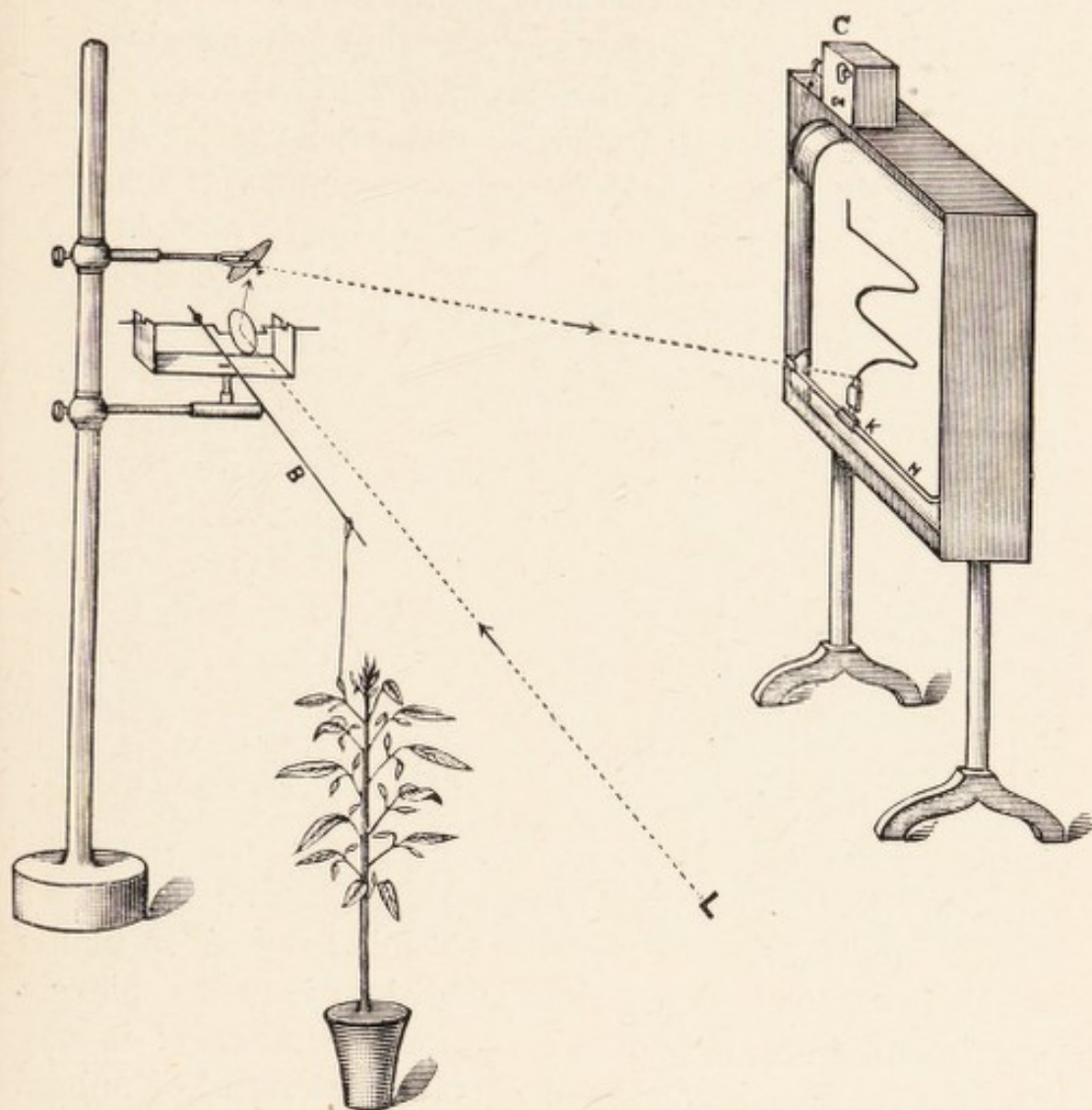
FIG. 7.—The Optical Pulse-Recorder. B, arm of optical lever attached to moving leaflet; L, ray of light, which after two reflections from the two mirrors falls on the recorder; C, clock-work, which keeps twin-drum—on which is wrapped the recording paper—revolving; H, horizontal guide bar; K, inkwell with projecting sponge.
