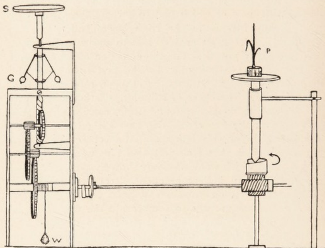
FIG. 19.—The Balanced Crescograph. Compensation of growth-movement produced by equal subsidence of the holder containing the plant (P). Adjusting screw (S) regulates the speed of the governor (G). W, heavy weight actuating clock-work.
