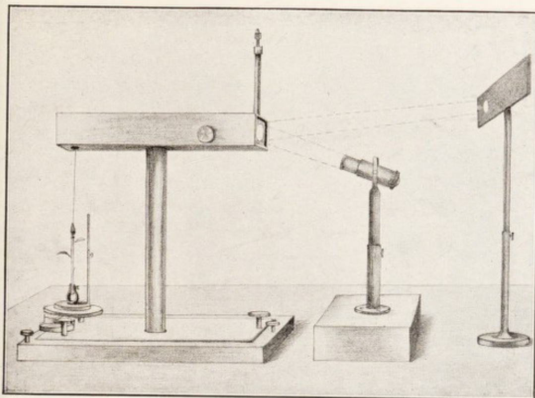
FIG. 18.—The Magnetic Crescograph for magnifying imperceptible growth of plants ten million times.
