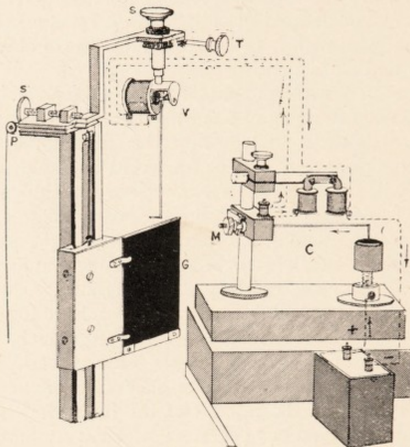
FIG. 10.—Upper part of the Resonant Recorder. Thread from clock, not shown, passes over pulley (P), letting down recording smoked glass plate (G) ; C, coacting reed which by its vibration sets recorder (V) in sympathetic vibration. The axis of recorder (V) is supported perpendicularly at centre of circular end of magnet. S S', adjusting screws ; M, micrometer ; T, tangent screw.
