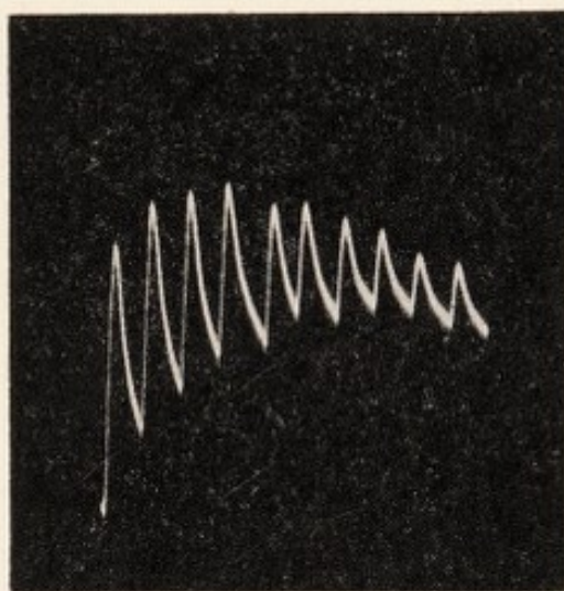
FIG. 3.—Electric response of metal showing fatigue (tin).
