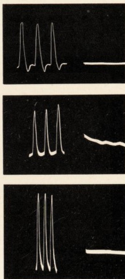
FIG. 5.—Action of poison in abolishing response of muscle (uppermost record), plant (middle record), and metal (lowest record).
