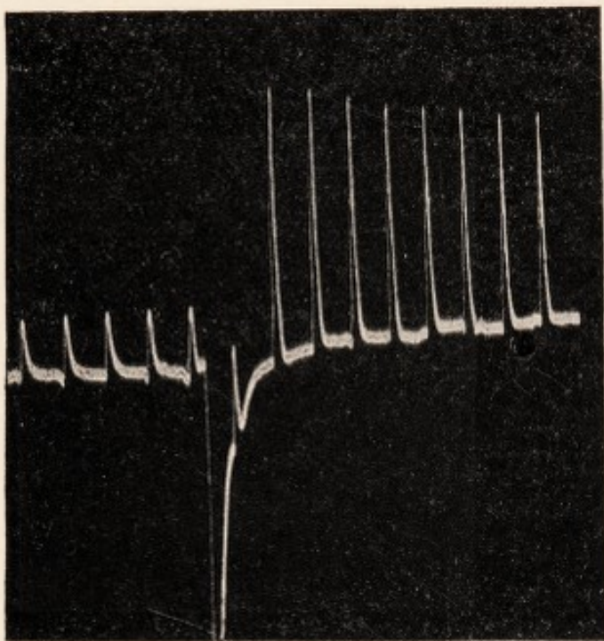
FIG. 4.—Action of stimulant in enhancing response of metal (platinum). In this and in following records the first series exhibit the normal response; the subsequent series show the effect of chemical agent.
