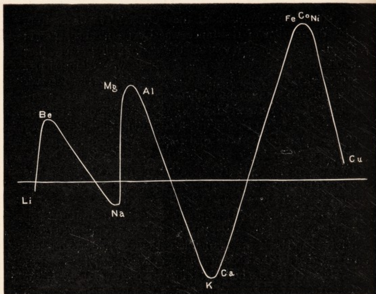
FIG. 1.—Periodicity of Electric Touch. Abscissa represents the atomic weight ; ordinate the electric touch positive or negative.
