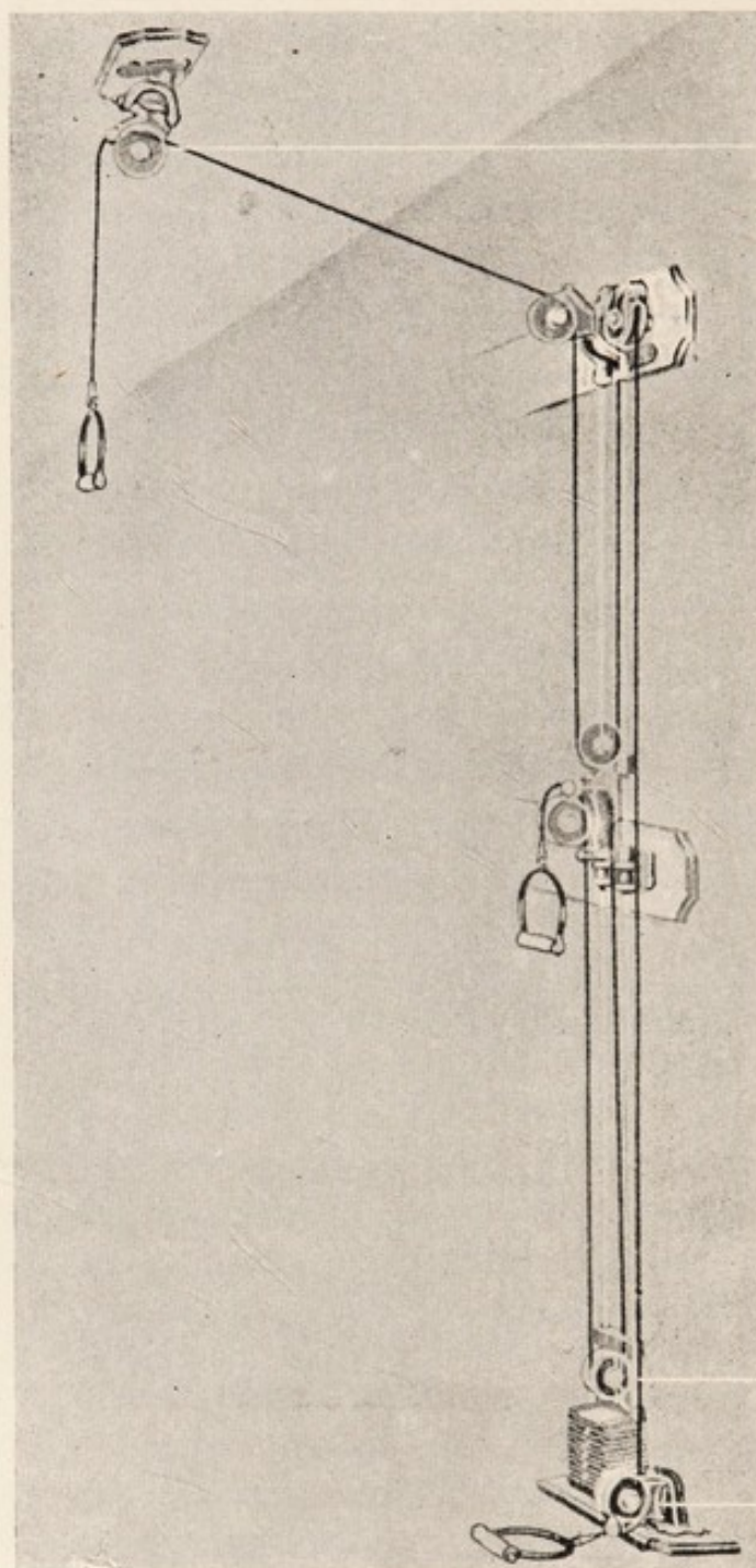
FIG. 41.—TRIPLEX PULLEY WEIGHT MACHINE.
