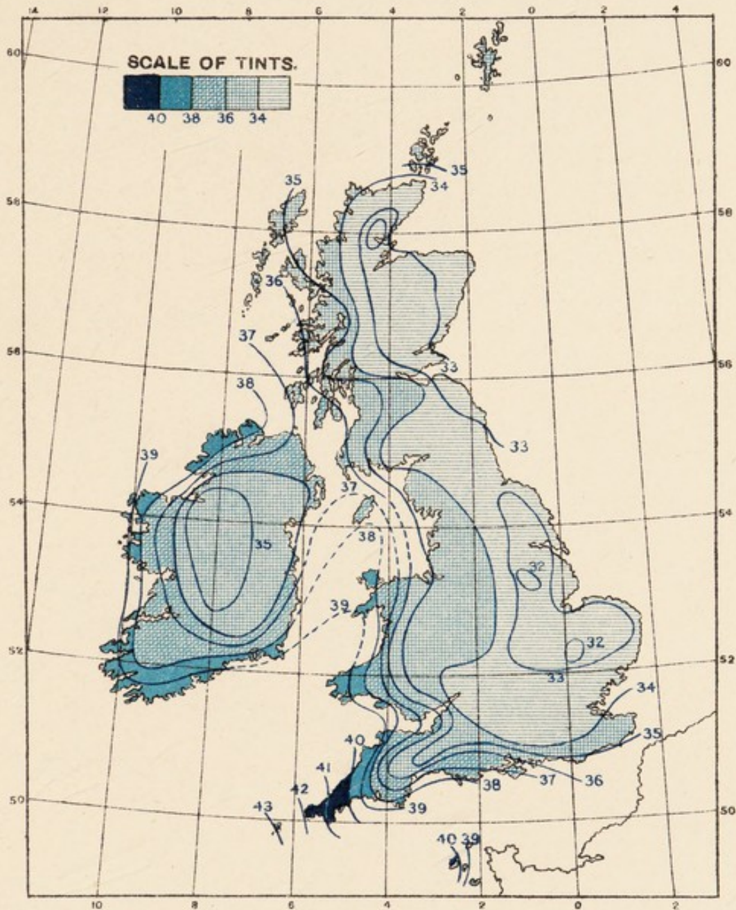
FIG. 86.—Mean Minimum (night) temperature of the British Islands for January (1875-1910): From the Monthly Normals of Temperature, Rainfall and Sunshine of the Meteorological Office. (By permission of H.M. Stationery Office.)
