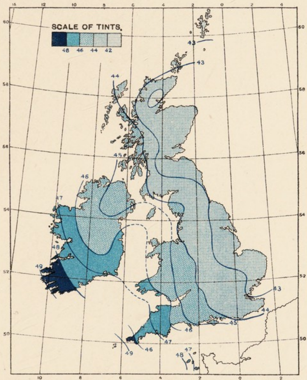
FIG. 85.—Mean Maximum (day) temperature of the British Islands for January. (By permission of H.M. Stationery Office.)
