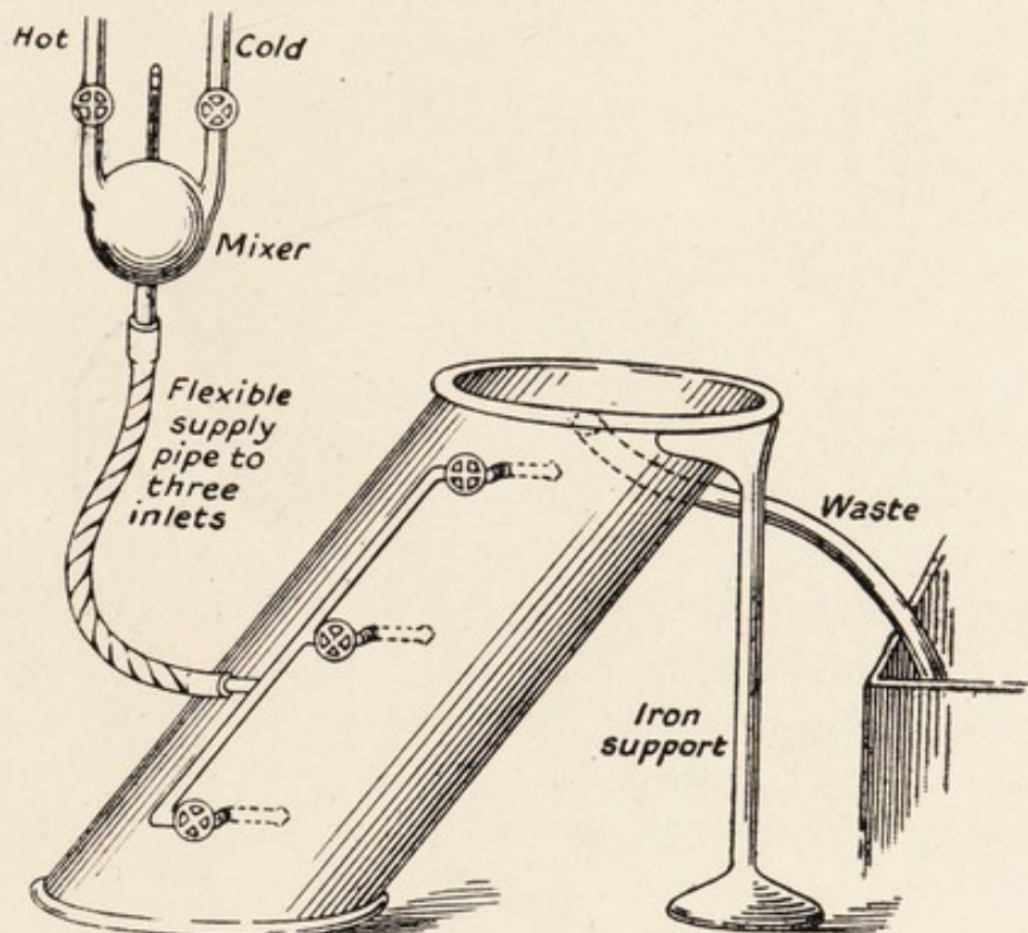
FIG. 6.—FRENCH "EAU COURANTE" BATH FOR THE LEG.
