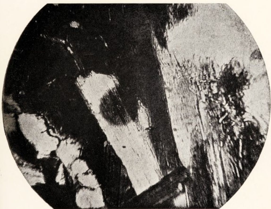
HALO IN BIOTITE.
