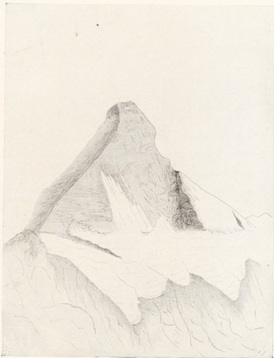
THE FOLDED ROCKS OF THE MATTERHORN : A SKETCH MADE IN 1906.
