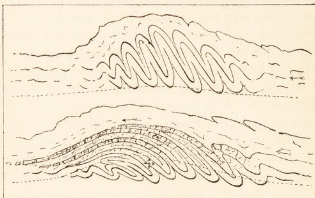
FORMATION OF RECUMBENT FOLDS.
