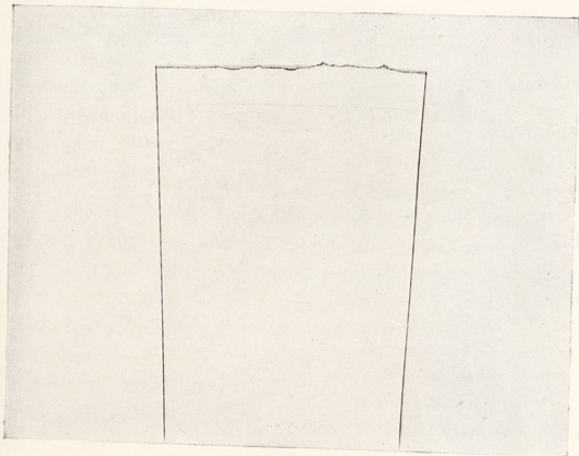
SECTOR OF THE EARTH.
