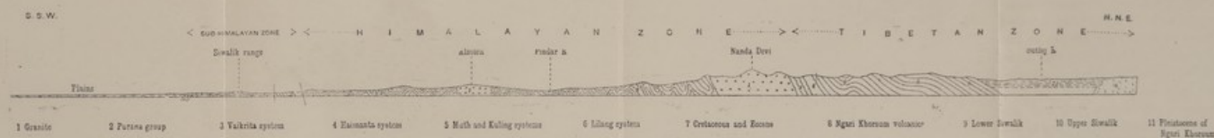
FIG. 2. THROUGH NANDA DEVI TO THE SUTLEJ
