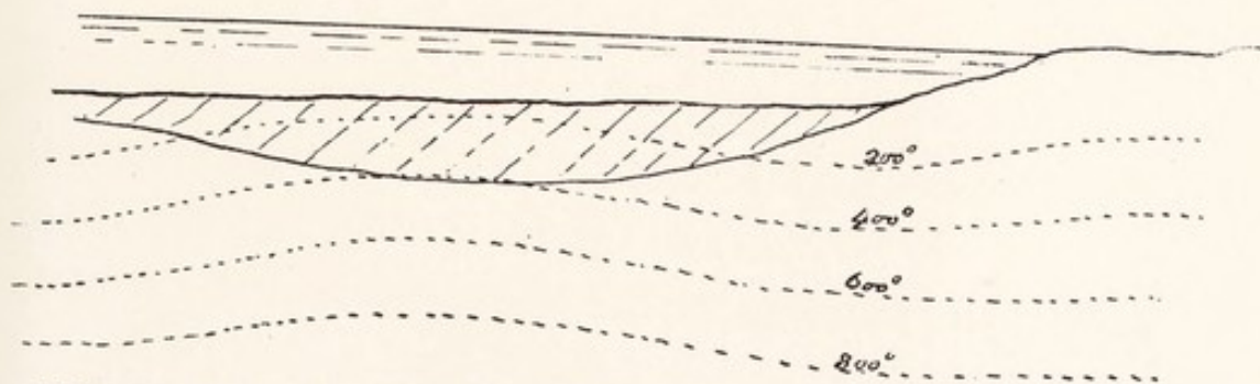
RISE OF ISOGEOTHERMS INTO A DEPOSIT EVOLVING RADIOACTIVE HEAT. Facing p. 118.
