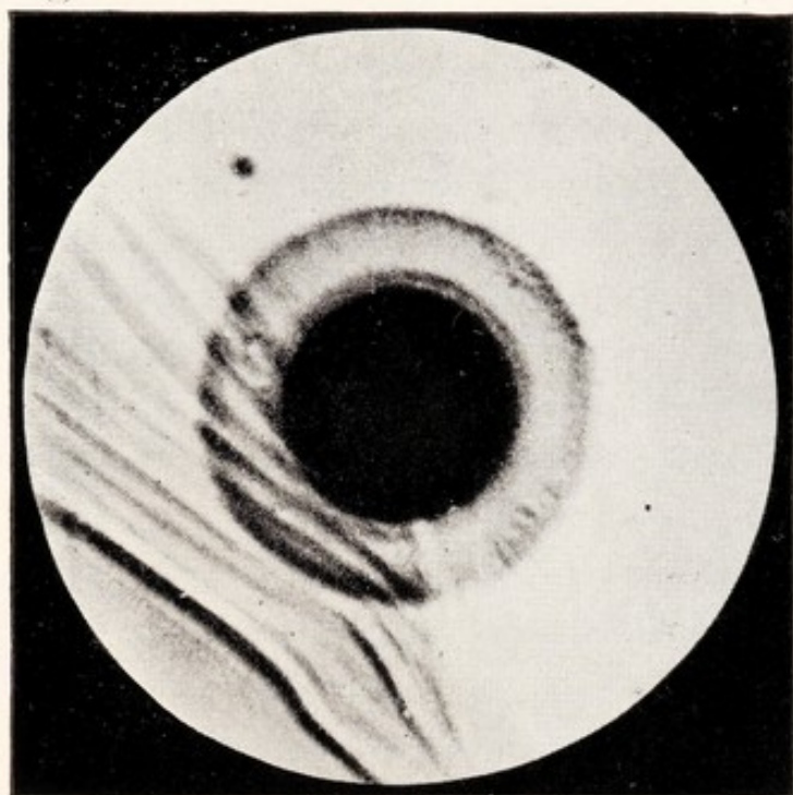
RADIUM HALO, MUCH ENLARGED.
