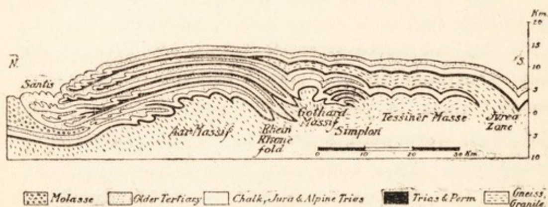
DIAGRAMMATIC SECTION THROUGH THE SWISS ALPS (AFTER SCHMIDT).
