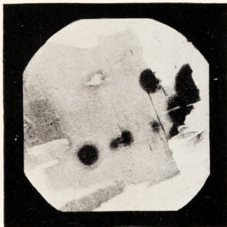
THORIUM AND RADIUM HALOES IN MICA.
