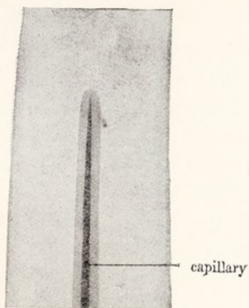
HALO ROUND CAPILLARY IN GLASS TUBE.
