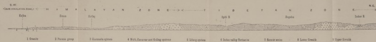
FIG. 1. THROUGH SPITI TO THE INDUS
