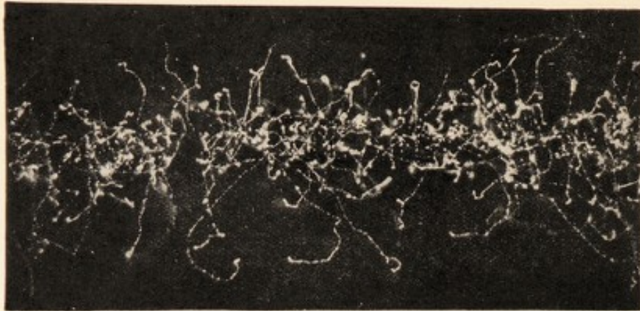
FIG. 1.—A photograph of the ionisation by an X-ray beam, showing paths of electrons liberated from atoms of gaseous matter.
