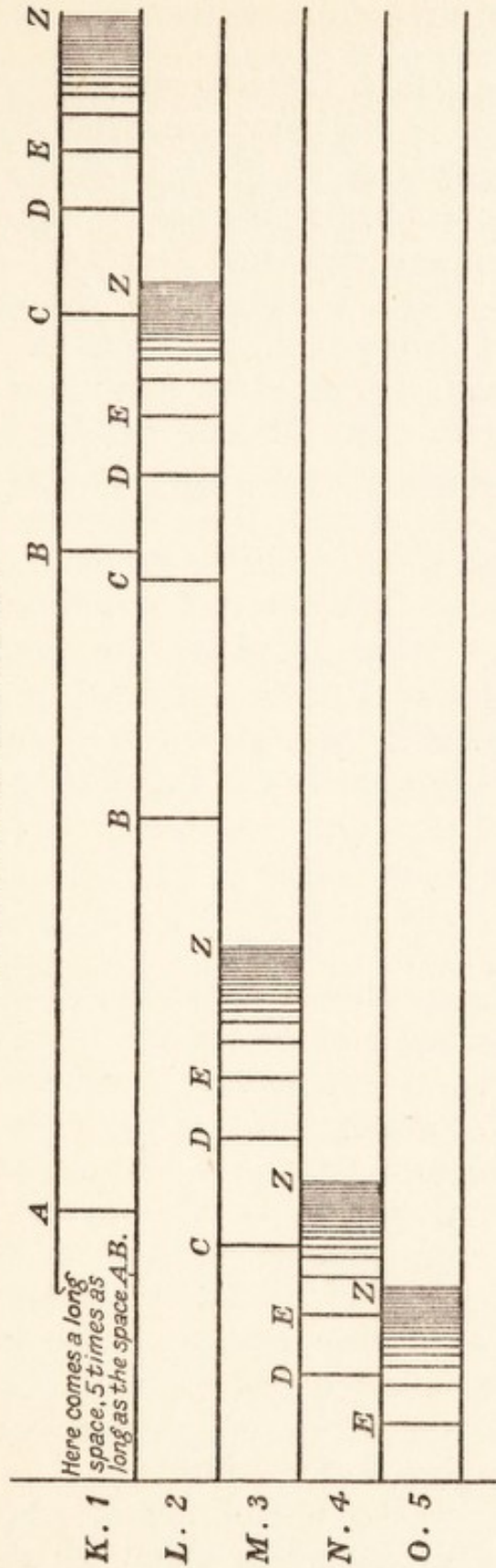
TYPICAL SERIES OF LINE SPECTRA.
