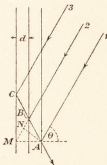
FIG. 4.—THEORY OF X-RAY SPECTROMETER.
